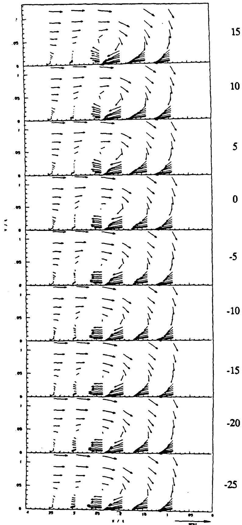
Figure 80: Vectors of velocity conditionally averaged on a pressure fall at x/t = -0.20 . Numbers indicate time before pressure switch in 10,000ths of a second.
