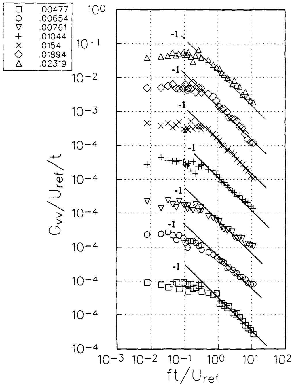
Figure 39a: Normalized v power spectral distribution at x/t = -.193 . Note offset ordinate and legend of y/t locations.
