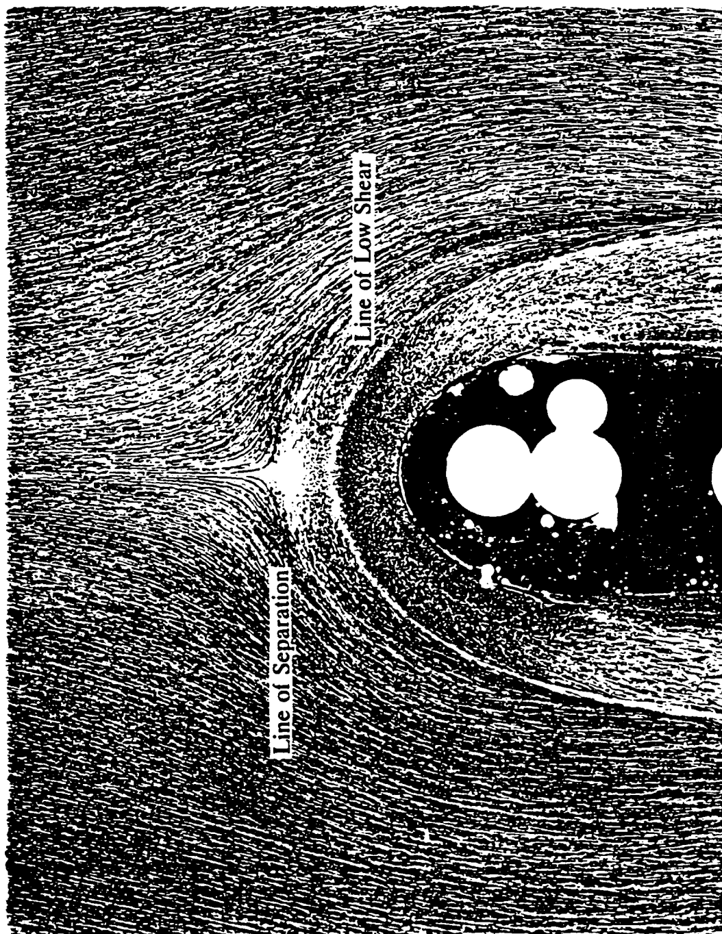
Figure 3: Oil flow in the nose region of the wing-body junction from Devenport and Simpson (1990b). Note line farthest away from nose is line of separation while line nearest nose is line of low shear.
