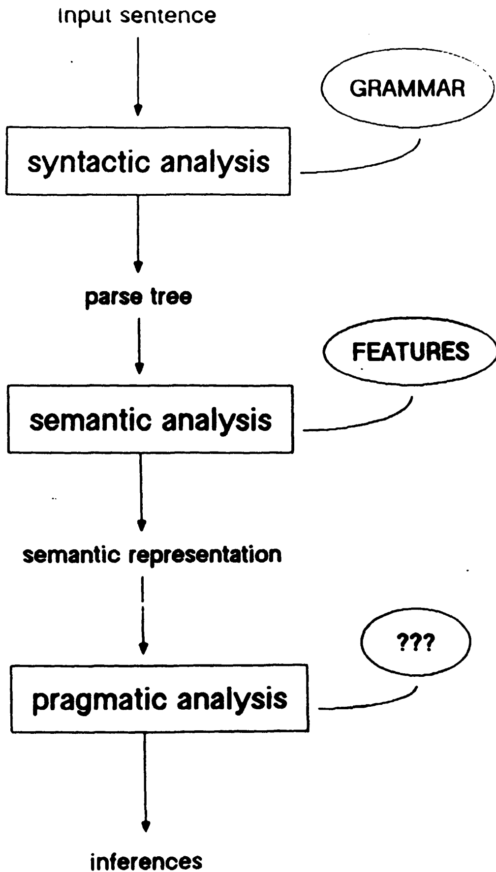
Figure 9. Serial Flow of Control
