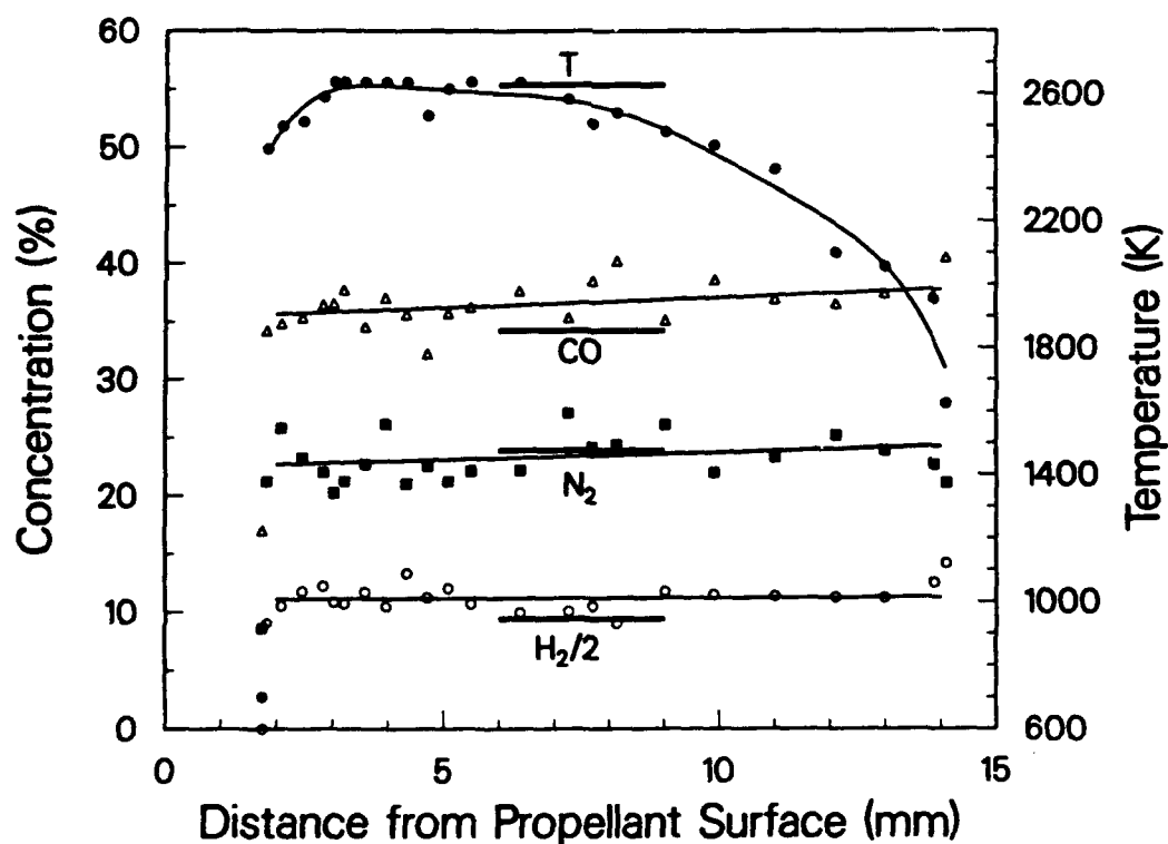
FIGURE 8 Summary of CARS measurements from HMX/TMETN combustion at 23.1 atm. ●—Temperature, \Delta —CO concentration, \circ —H 2 concentration, ■—N 2 concentration. The thick horizontal bars above each experimental parameter represent the value predicted from chemical equilibrium calculations. The thin lines are least-squares fits to the data points.
