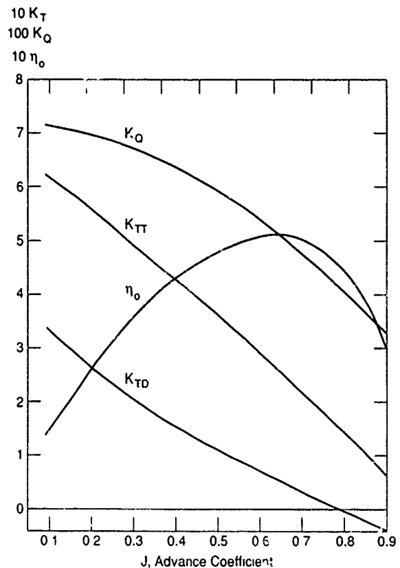
Figure 26. Propulsion characteristics (SSPA results).
