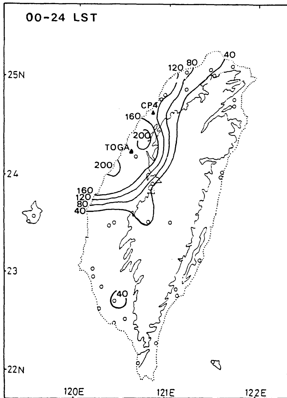
Figure 3.10. The accumulated amount of rainfall in 24 hours in 25 June 1987 over Taiwan. Contour interval is 40 mm per 24 hours.
