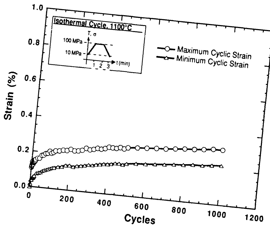
Figure 4-4. Cyclic strain response of [0]_{16} SiC/CAS-II to an isothermal fatigue profile with a 60 sec. hold at \sigma_{\max} . \sigma_{\max} = 100 MPa (14.5 ksi), R = 0.1
