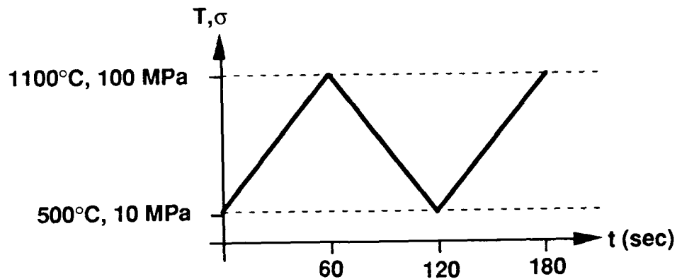
Figure 3-19. Thermomechanical fatigue profile with no hold.
