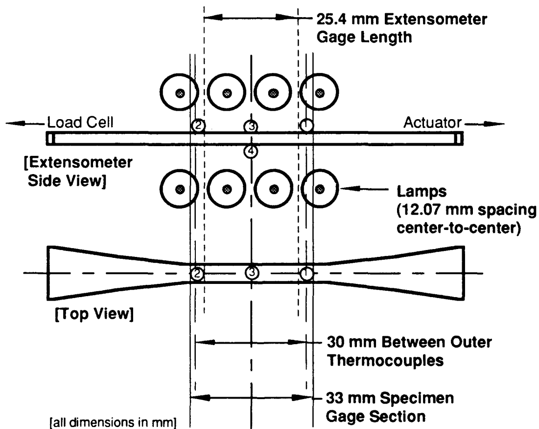
Figure 3-12. Thermocouple Positions. Numbers correspond to zones controlled by the numbered thermocouple.
