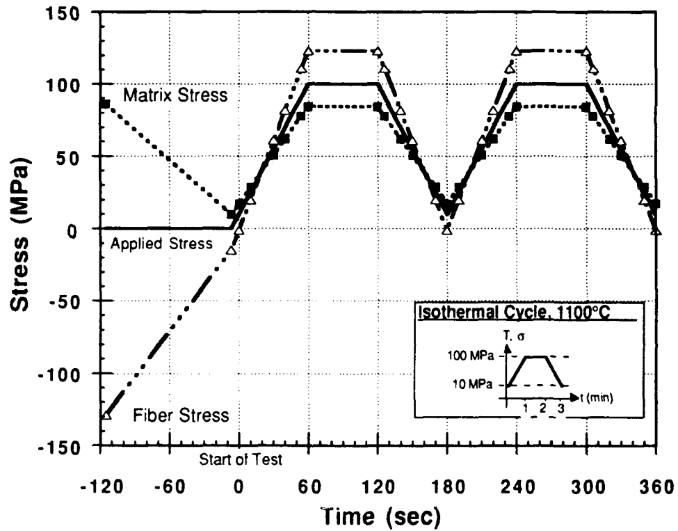
Figure 4-14. Axial stress states in the fiber and matrix plotted with applied stress for an isothermal fatigue cycle including a 60 sec. hold at \sigma_{\max} .
