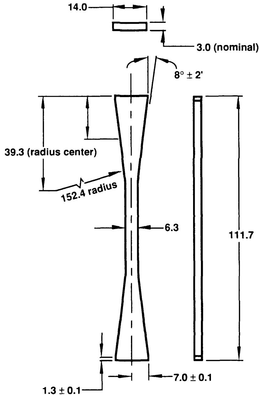
Figure 3-7. Edge-loaded test specimen geometry. All dimensions in mm.
