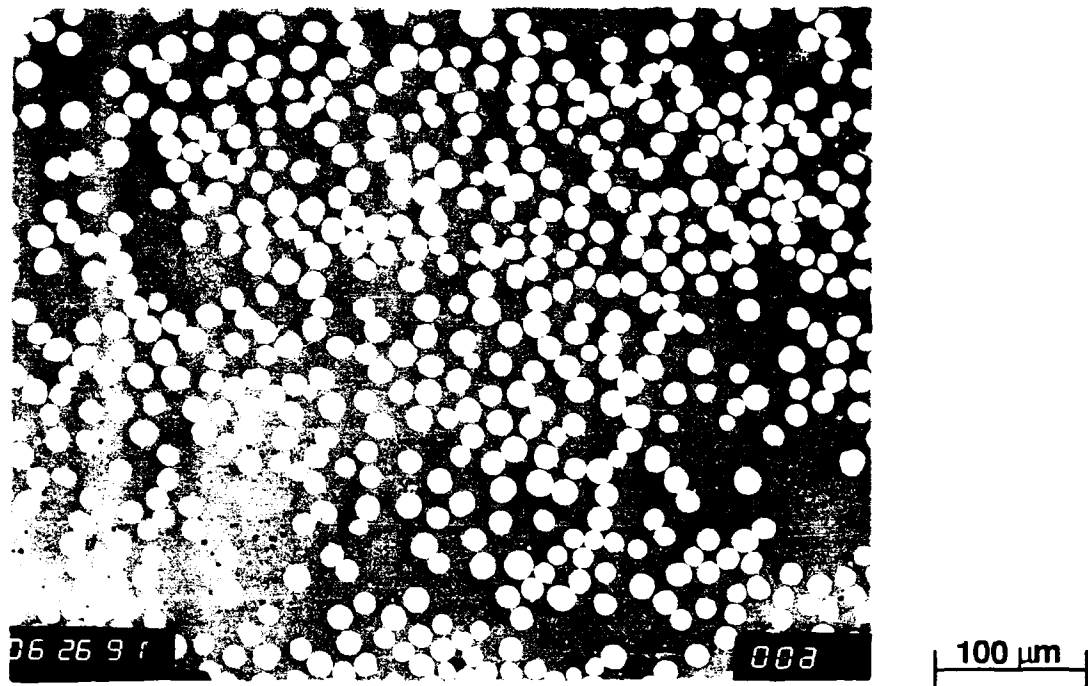
Figure 3-1. Microstructure of SiC/CAS-II, Transverse View. 200X
