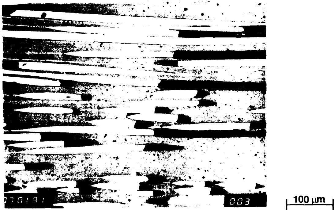
Figure 3-2. Microstructure of SiC/CAS-II, Longitudinal View. 200X
