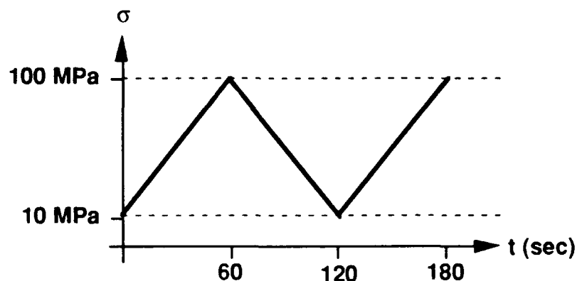
Figure 3-17. Isothermal fatigue profile with no hold.
