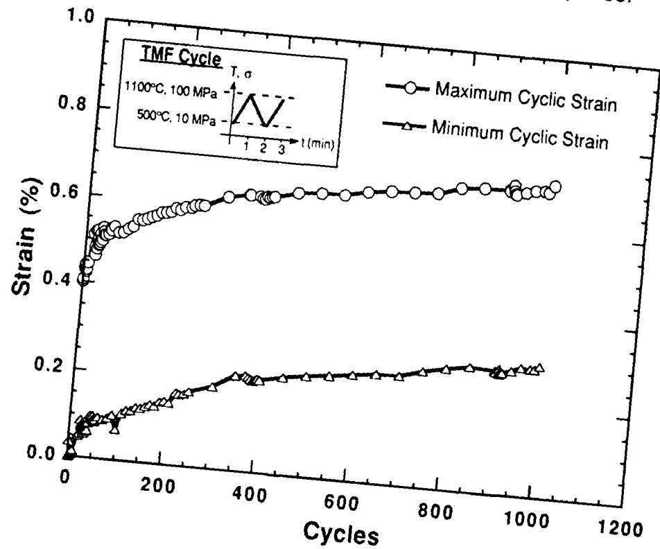
Figure 4-5. Cyclic strain response of [0]_{16} SiC/CAS-II to a thermomechanical fatigue profile. \sigma_{\max} = 100 MPa (14.5 ksi), R = 0.1 , T_{\text{range}} = 500\text{-}1100^{\circ}\text{C} .
