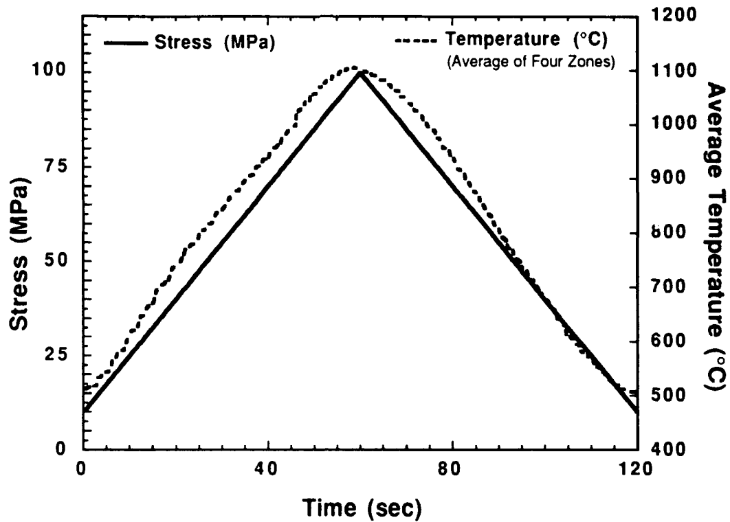
Figure 3-15. Typical stress and temperature profiles for thermomechanical fatigue tests without hold time. Temperature shown is the average temperature from the four control zones.
