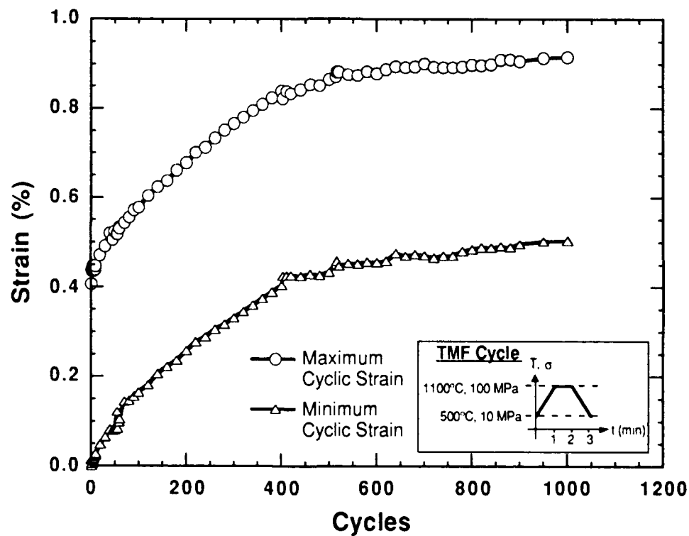
Figure 4-6. Cyclic strain response of [0] 16 SiC/CAS-II to a thermomechanical fatigue profile with a 60 sec. hold at \sigma_{\max} . \sigma_{\max} = 100 MPa (14.5 ksi), R = 0.1 , T_{\text{range}} = 500\text{-}1100^{\circ}\text{C} .
