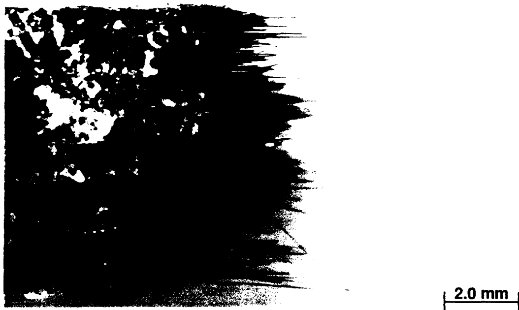
Figure 4-18. Surface of a specimen thermomechanical fatigue profile with a 60 sec. hold at \sigma_{\max} . The bubbly appearance indicates possible localized melting. White areas are residual cement used to affix thermocouples. 12.5X
