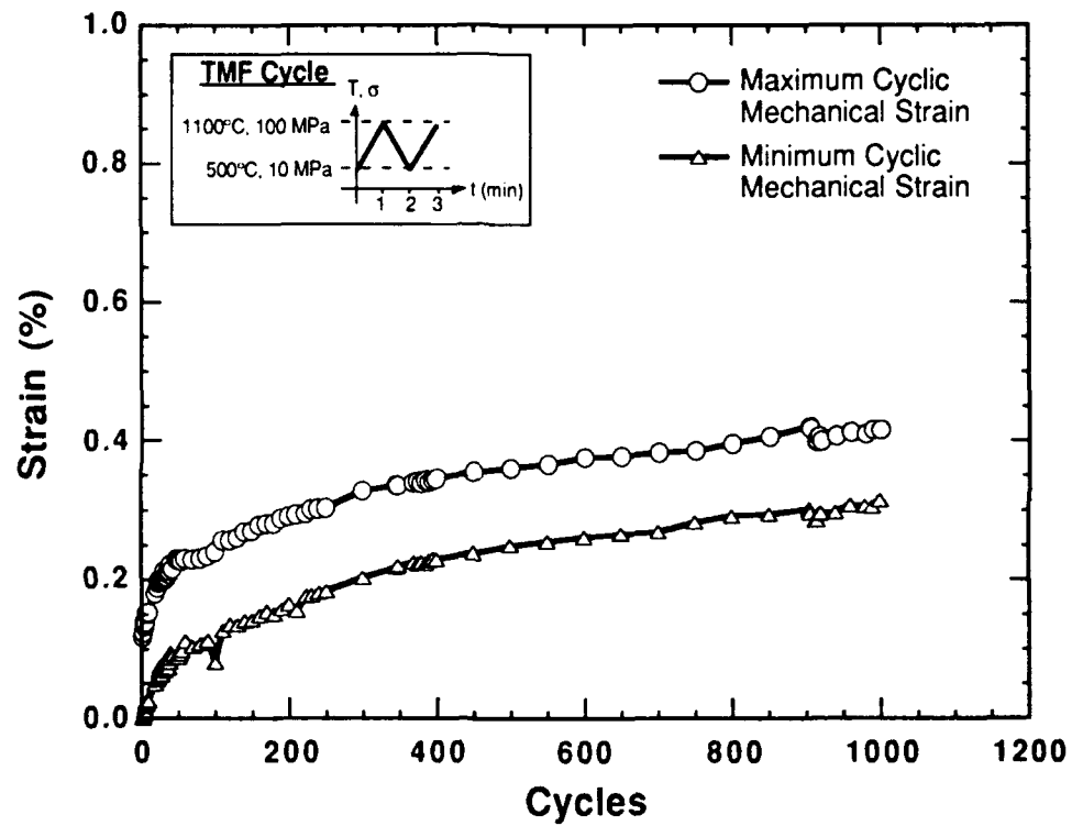
Figure 4-7. Cyclic mechanical strain response of [0]_{16} SiC/CAS-II to the same thermomechanical fatigue profile depicted in Figure 4-5. \sigma_{\max} = 100 MPa (14.5 ksi), R = 0.1 , T_{\text{range}} = 500\text{-}1100^{\circ}\text{C} .
