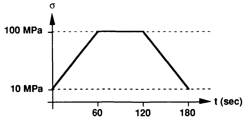
Figure 3-18. Isothermal fatigue profile with 60 sec. hold at maximum stress and temperature.
