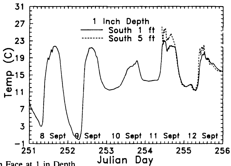
Figure B-1. Temperatures From "Joyce Kilmer" for 8 - 12 Sept From the (a.) North and (b.) South Face Probes at the 1 in Depth
