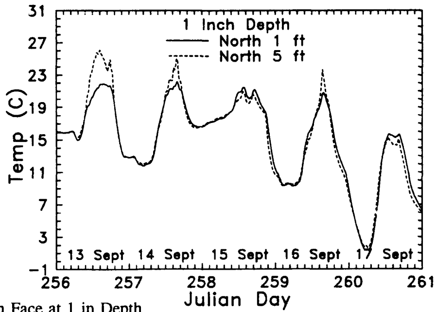
(a.) North Face at 1 in Depth
