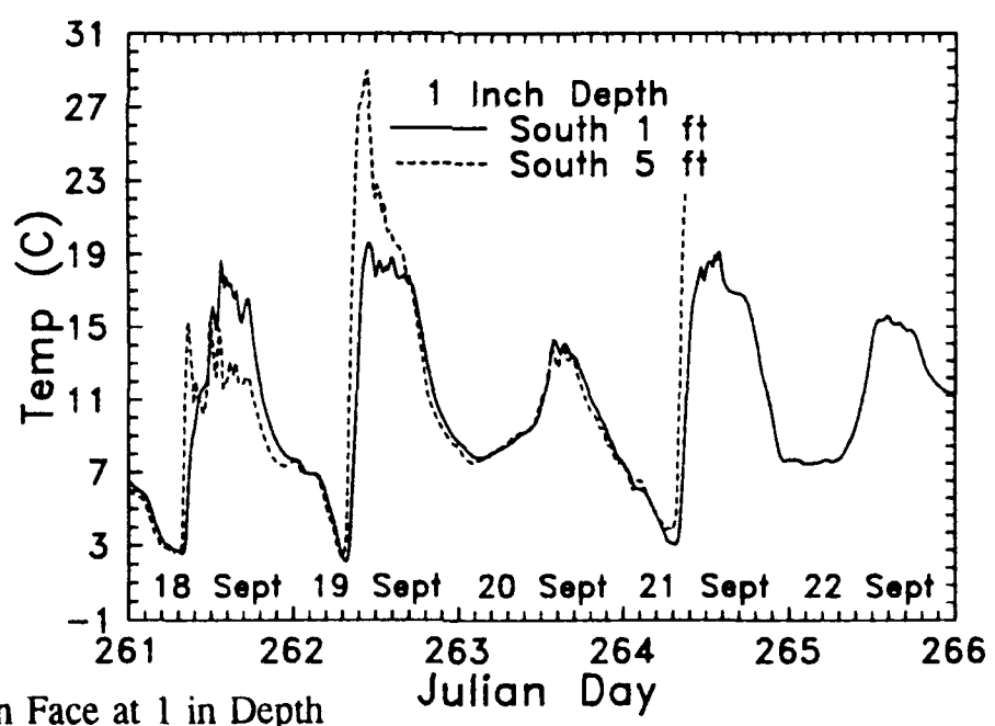
Figure B-3. Temperatures From "Joyce Kilmer" for 18 - 22 Sept From the (a.) North and (b.) South Face Probes at the 1 in Depth
