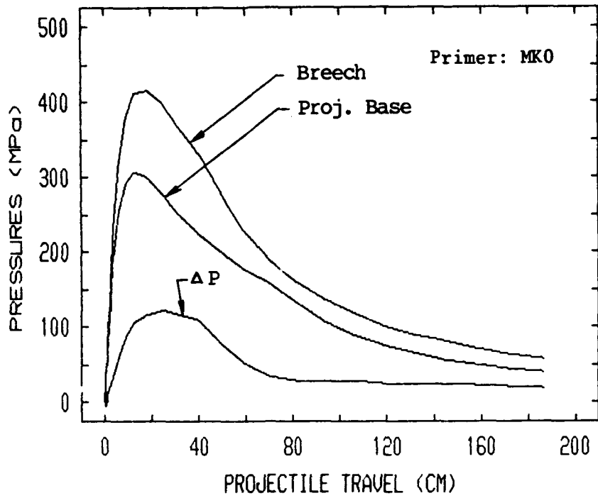
Figure 10. Pressures at Breech and Projectile Base and Their Differential (Single-Base Charge).
