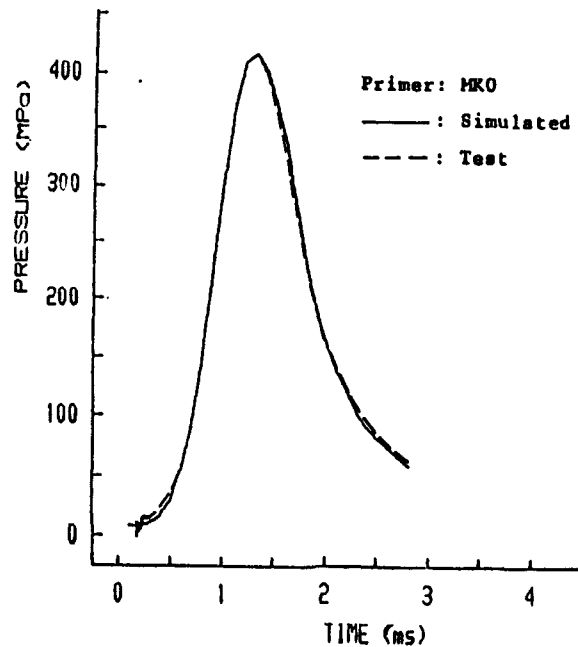
Figure 6. Breech Pressures: Tested and Simulated (Single-Base Charge)
