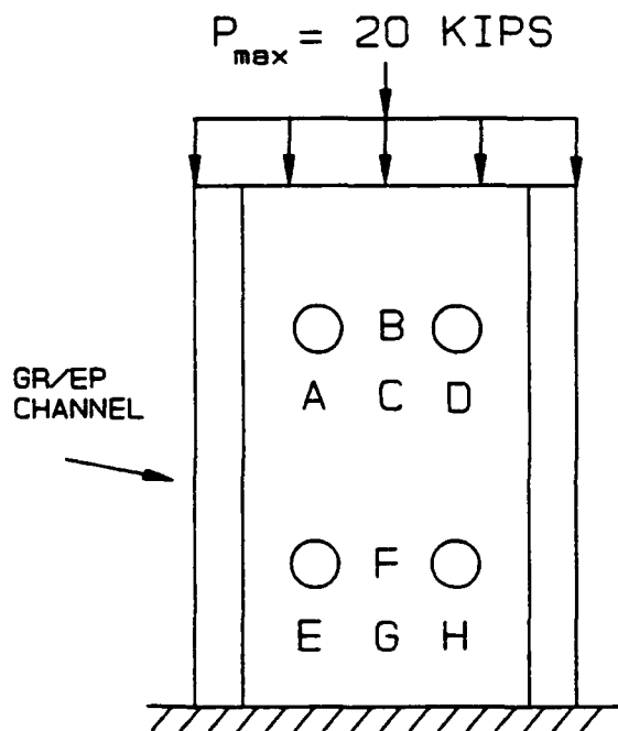
Figure 21. Loading configuration and strain data.
