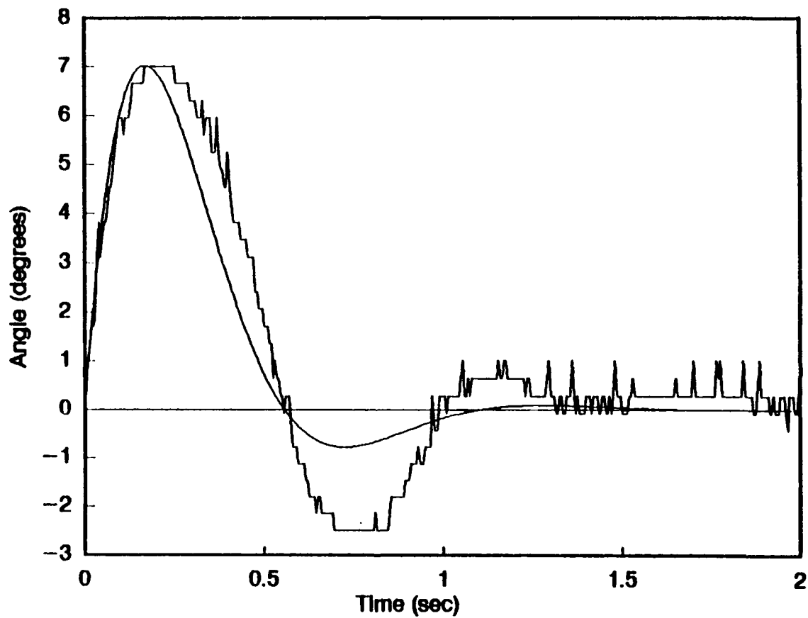
Figure 78. Comparison of the azimuth trace and the model using \zeta=0.57 and \lambda_n=4.83 m from the 5 \text{ m s}^{-1} run TADE where \Lambda_0 was found to be 94.66 \text{ deg s}^{-1} .
