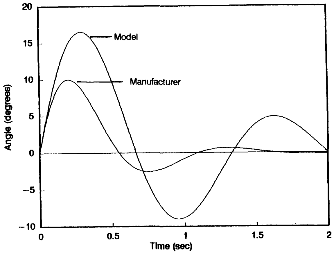
Figure 75. Same as in Figure 74, but for the elevation response.
