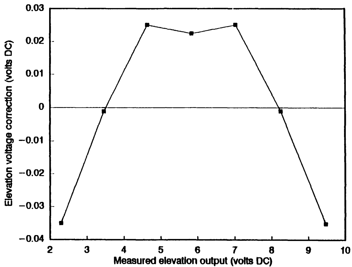
Figure 16. Same as Figure 15, but for elevation correction values.
