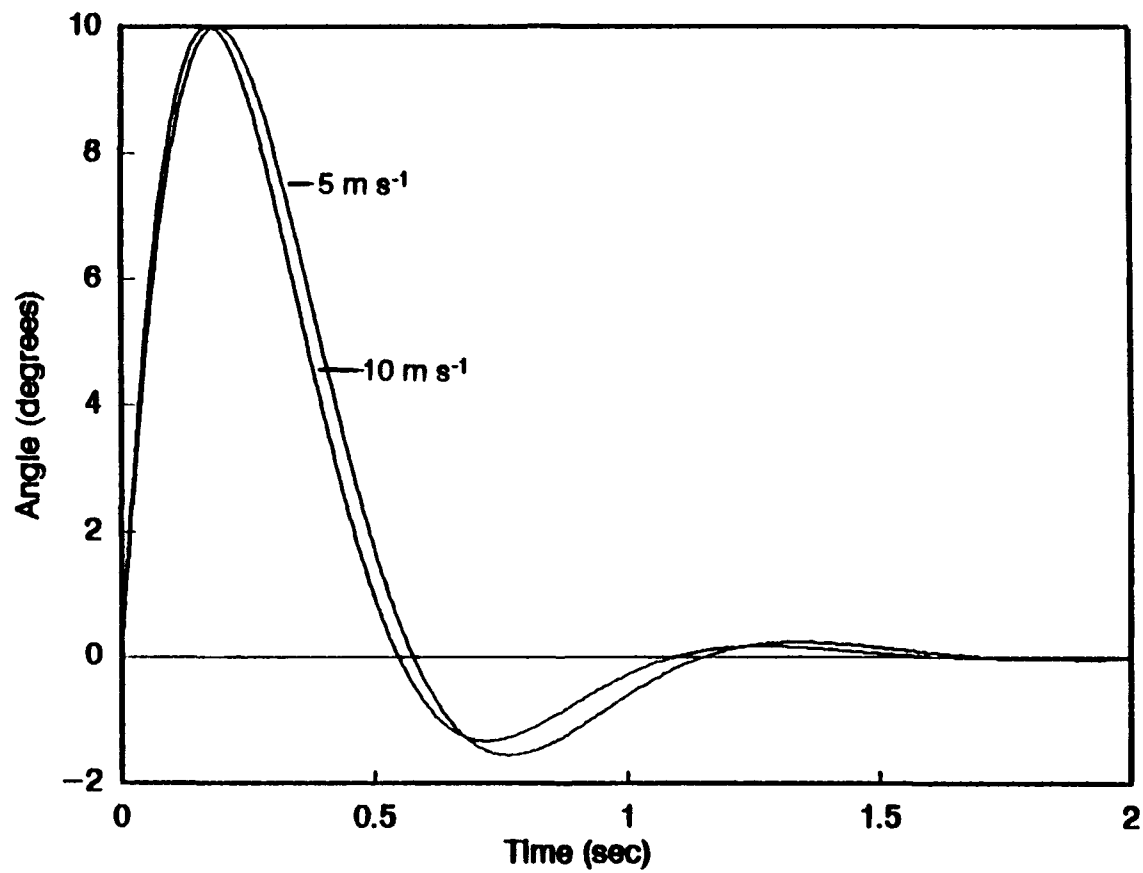
Figure 58. Same as Figure 57, but with the 10 m s -1 trace forced to a first peak of 10° by increasing \Lambda_0 .
