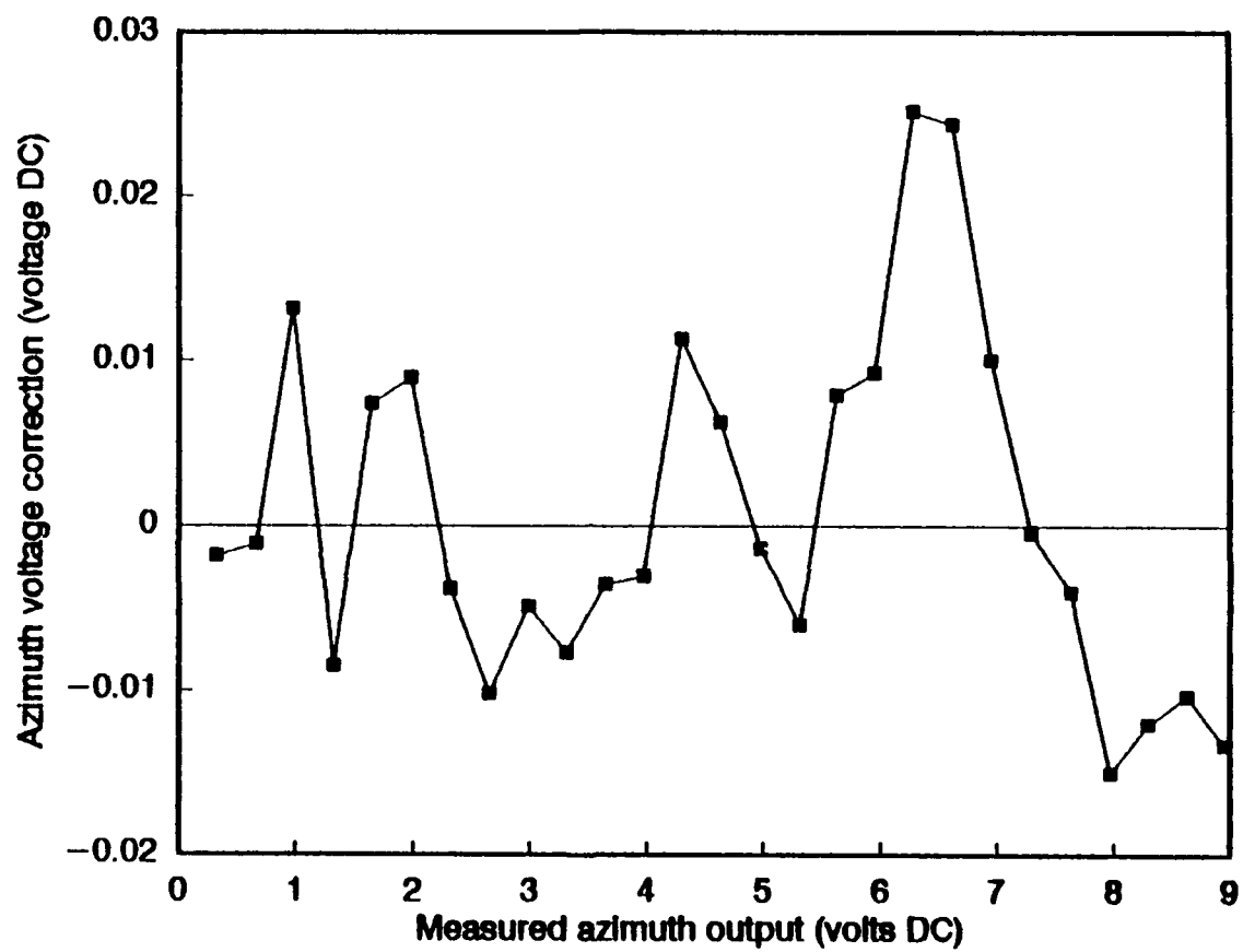
Figure 15. Azimuth correction values as a function of voltage output derived for this particular R. M. Young bivane.
