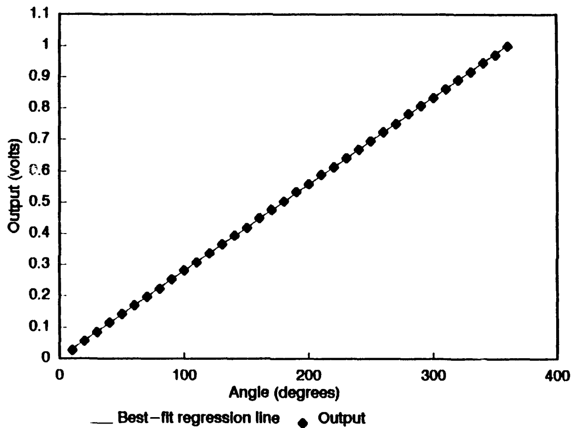
Figure 33. Consolidated output voltages from the Ciimatronics bivane azimuth static test with a best-fit regression line.
