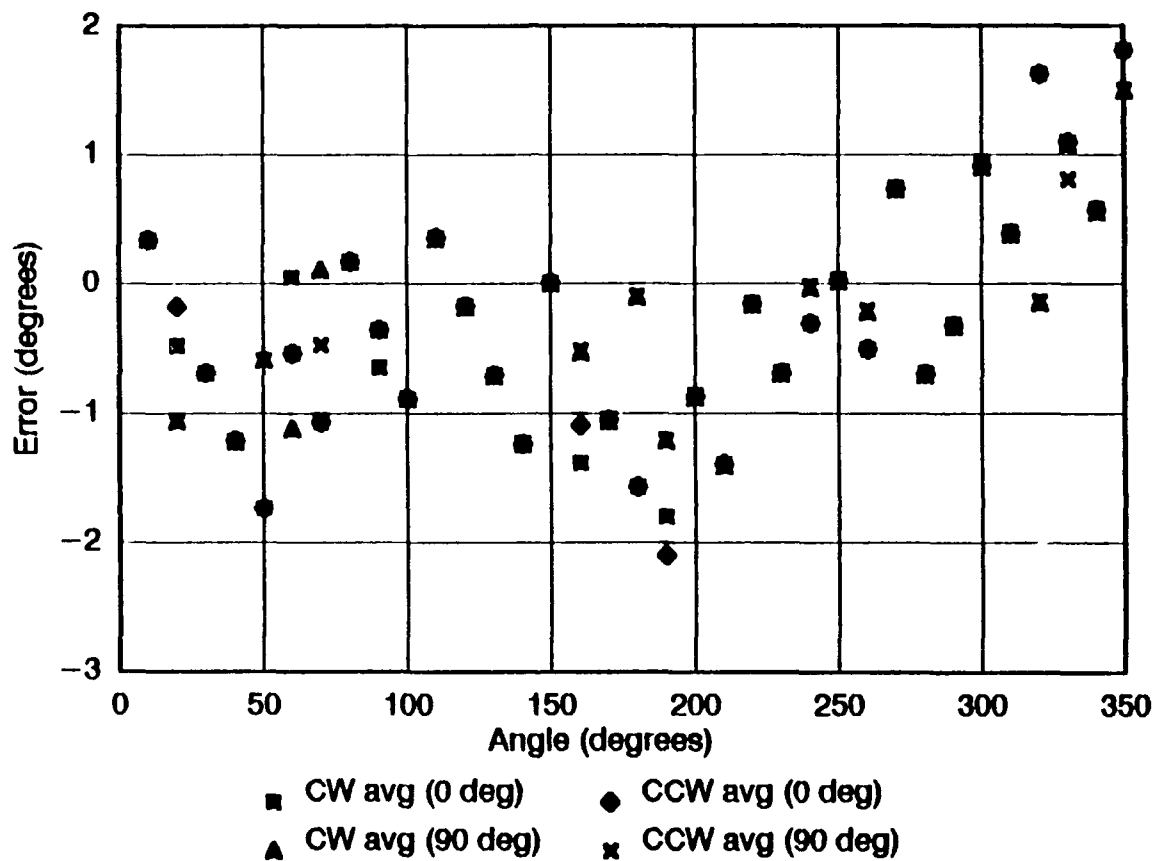
Figure 35. Climatronics bivane azimuth static test at the 25° vertical position. Clockwise (CW) and counterclockwise (CCW) data from both horizontal positions (0° and 90°) of the machined static test wheel are shown with the best-fit regression subtracted from the individual voltage values.
