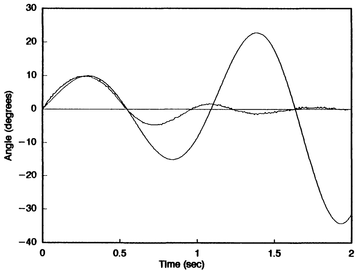
Figure 79. Same as in Figure 78, but for the elevation data \zeta=-0.13 and \lambda_n=5.73 m where \Lambda_0 was found to be 46.58 \text{ deg s}^{-1} .
