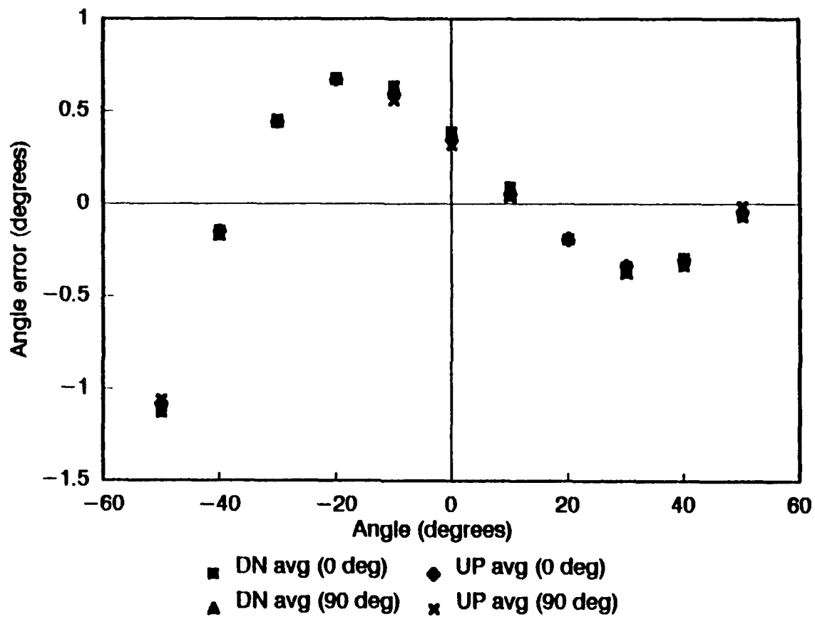
Figure 37. Climatronics bivane elevation static test. Up and down data from both horizontal positions (0° and 90°) of the machined static test wheel are shown with the best-fit regression line subtracted from the individual voltage values.
