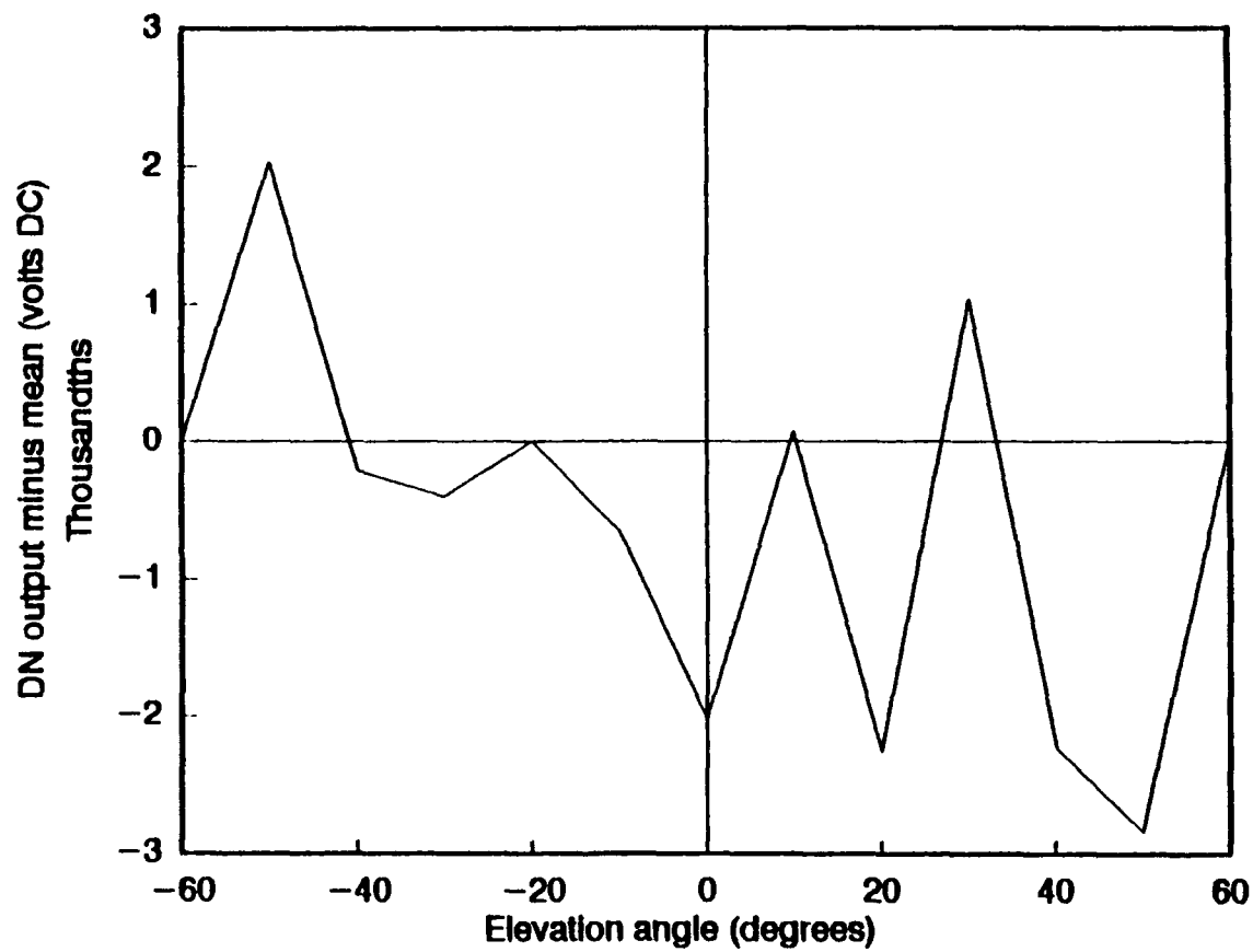
Figure 31. Same as in Figure 20 with down motion, but for the Teledyne Geotech elevation resolver that produces no \Delta V .
