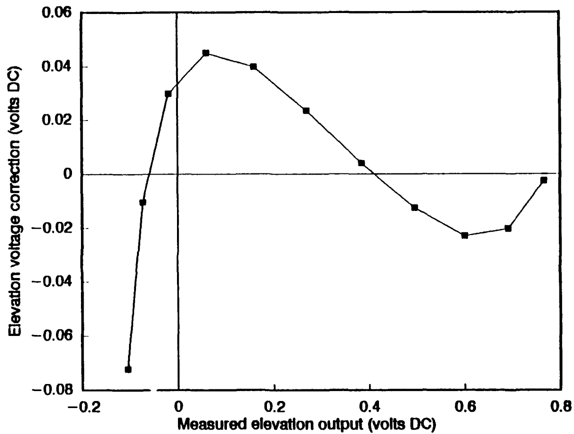
Figure 38. Elevation correction values as a function of voltage output derived for this particular Climatronics bivane.
