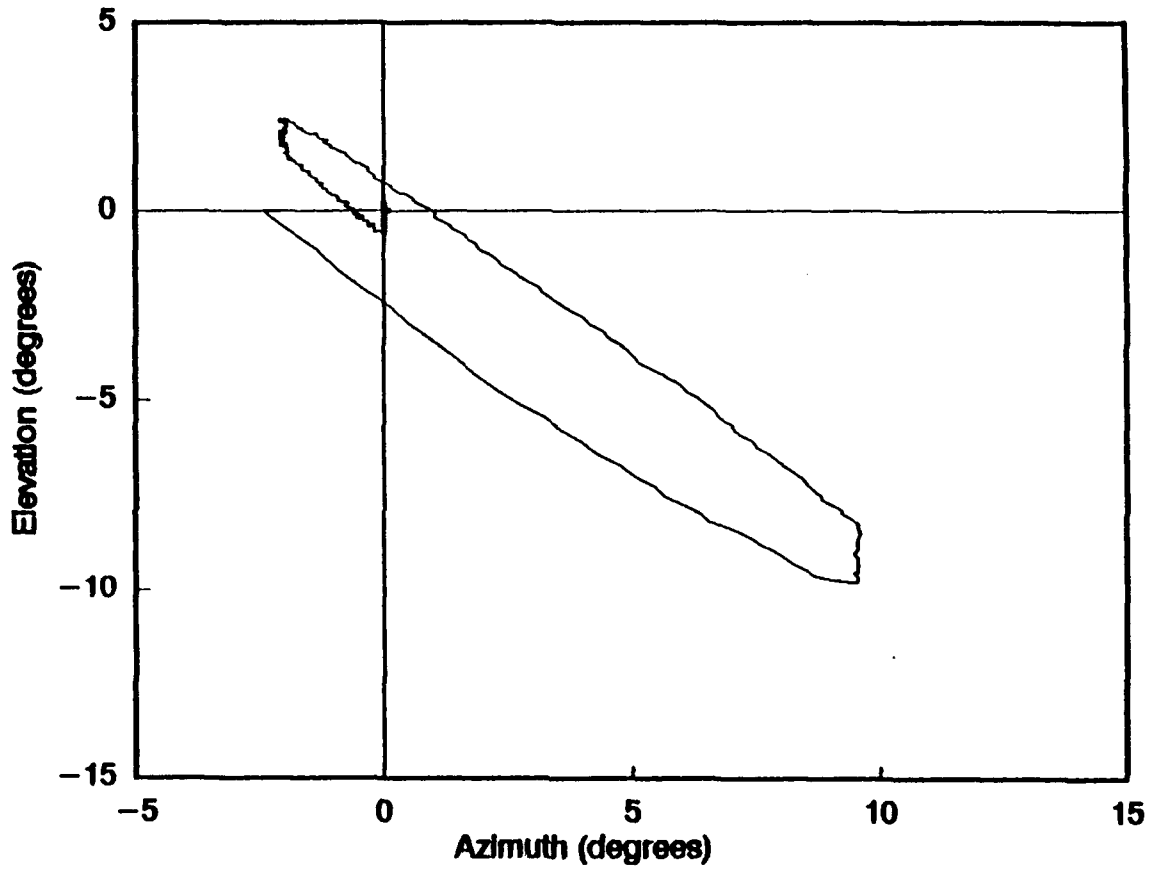
Figure 61. Plot showing the spiral into the equilibrium position resulting from a mismatch in the azimuth and elevation dynamic characteristics (from run YABC). The trace begins at the first zero-crossing.
