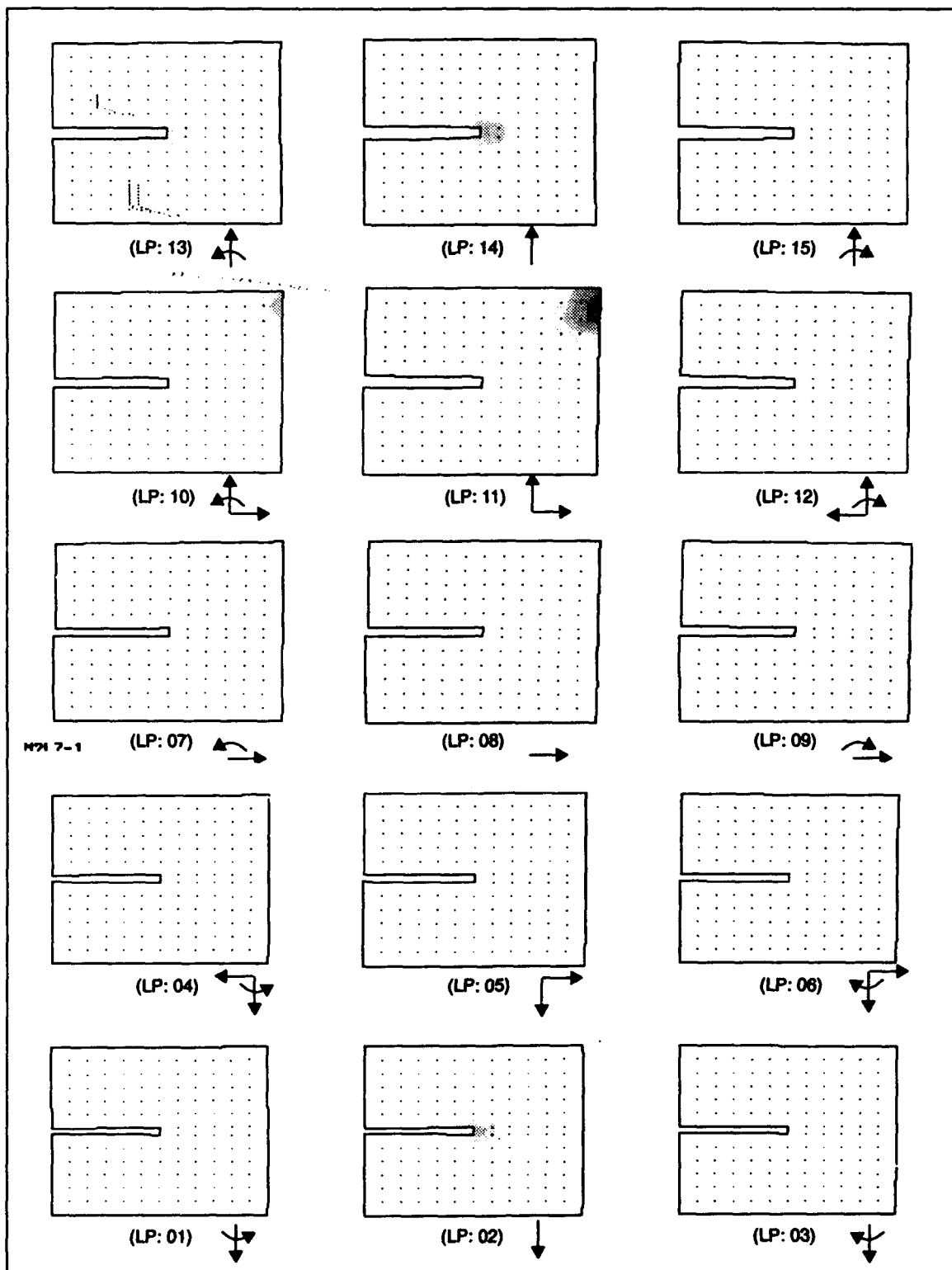
Fig. 25 — Distributions of dissipated energy on the deformed specimen for load magnitude 2, material 002 (AS1/3506-1 [+/- 30°]), for each of the load paths 1-15
