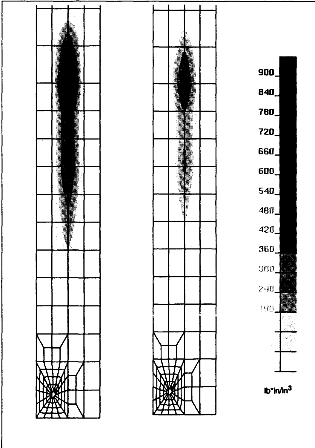
Fig. 21 — Front views of dissipated energy distributions of ship mast made out of thermoset material 007 (AS4/3501-6 [+/-60°]) (left) and out of thermoplastic material 040 (AS4/PEEK [+/-60°]) (right), for 3x of the total loading corresponding to front wind
