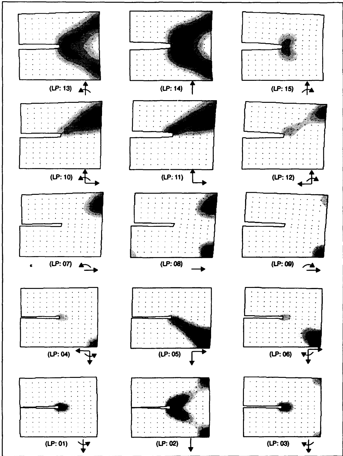
Fig. 27 — Distributions of dissipated energy on the deformed specimen for load magnitude 4, material 002 (AS1/3506-1 [ \pm 30^\circ ]), for each of the load paths 1-15
