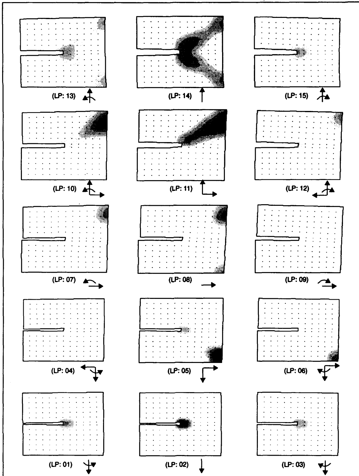
Fig. 26 — Distributions of dissipated energy on the deformed specimen for load magnitude 3, material 002 (AS1/3506-1 [ \pm 30^\circ ]), for each of the load paths 1-15
