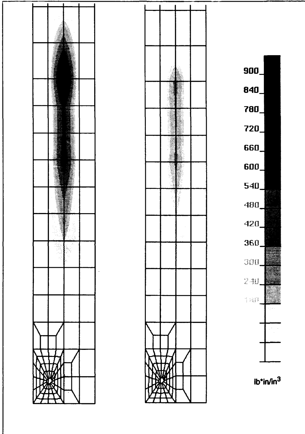
Fig. 20 — Front views of dissipated energy distributions of ship mast made out of thermoset material 007 (AS4/3501-6 [+/-60°]) (left) and out of thermoplastic material 040 (AS4/PEEK [+/-60°]) (right), for 2x of the total loading corresponding to front wind
