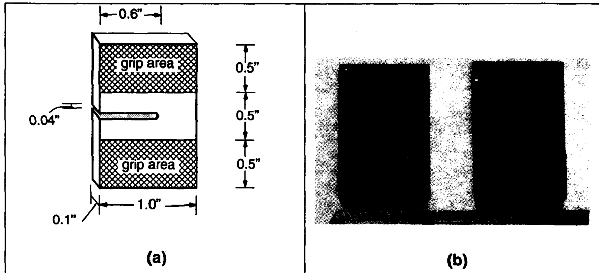
Fig. 3 — (a) Schematic of the specimen and the associated areas, (b) photos of representative specimen before testing (left) and after testing (right) for material 2 with 3501-6 resin AS1 fiber and +/- 30° layup and loading path 11
