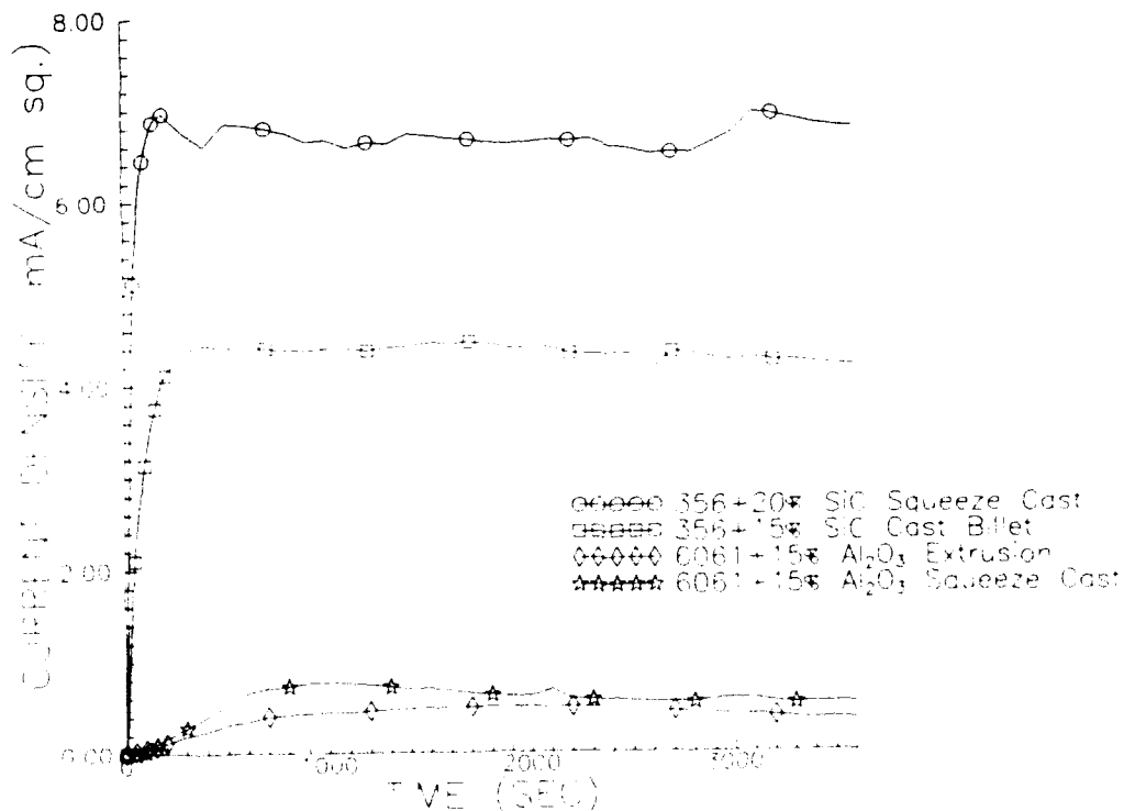
Figure 8. Potentiostatic behavior of the MMCs at -0.7volts for 60min in 3.5% NaCl pH 6 solution.
