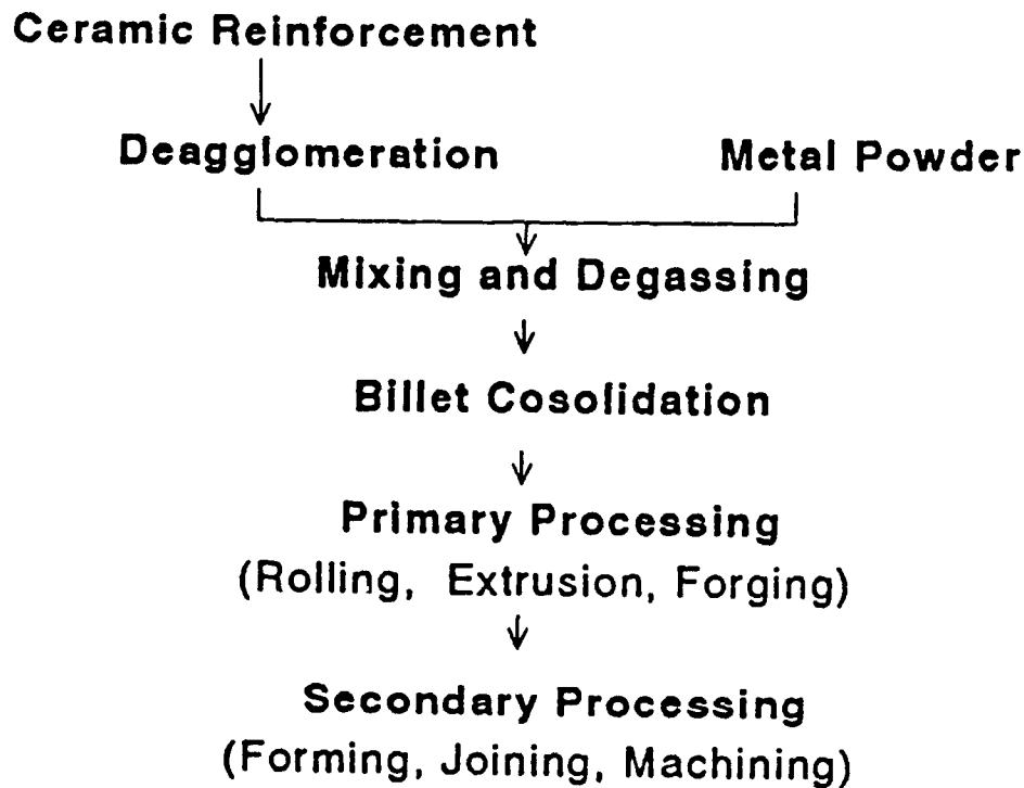
Figure 1. Schematic of PM-MMC fabrication (ref 8.)
