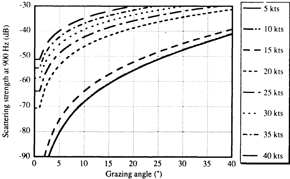
Fig. 6 - Surface scattering strengths as a function of grazing angle and wind speed for a frequency of 900 Hz
