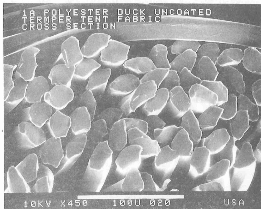
Figure 6: SEM photograph of a yarn of polyester duck showing gaps between fibers. (x450)
