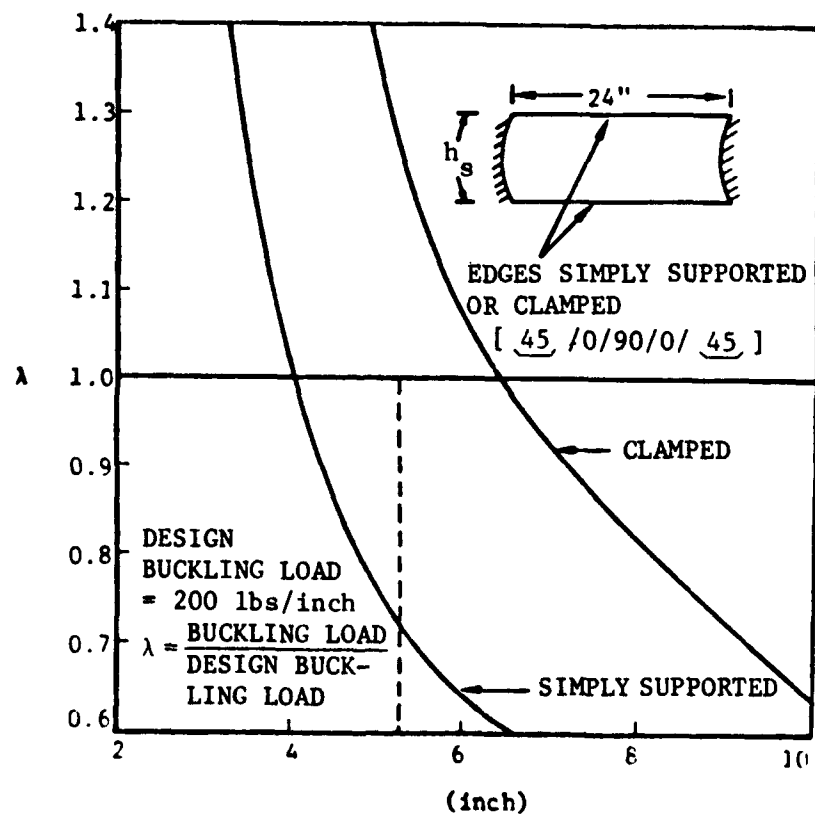
Figure 10. Shear Buckling Load N_{xy}^0 Versus Stringer Spacing for [ 45_2/90/45_2 ] and [ 45_0/90/0/45 ] Skin Layouts.
