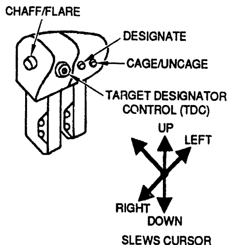
Figure 4. Throttle Switches
