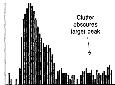
Fig 4 Regular histogram
