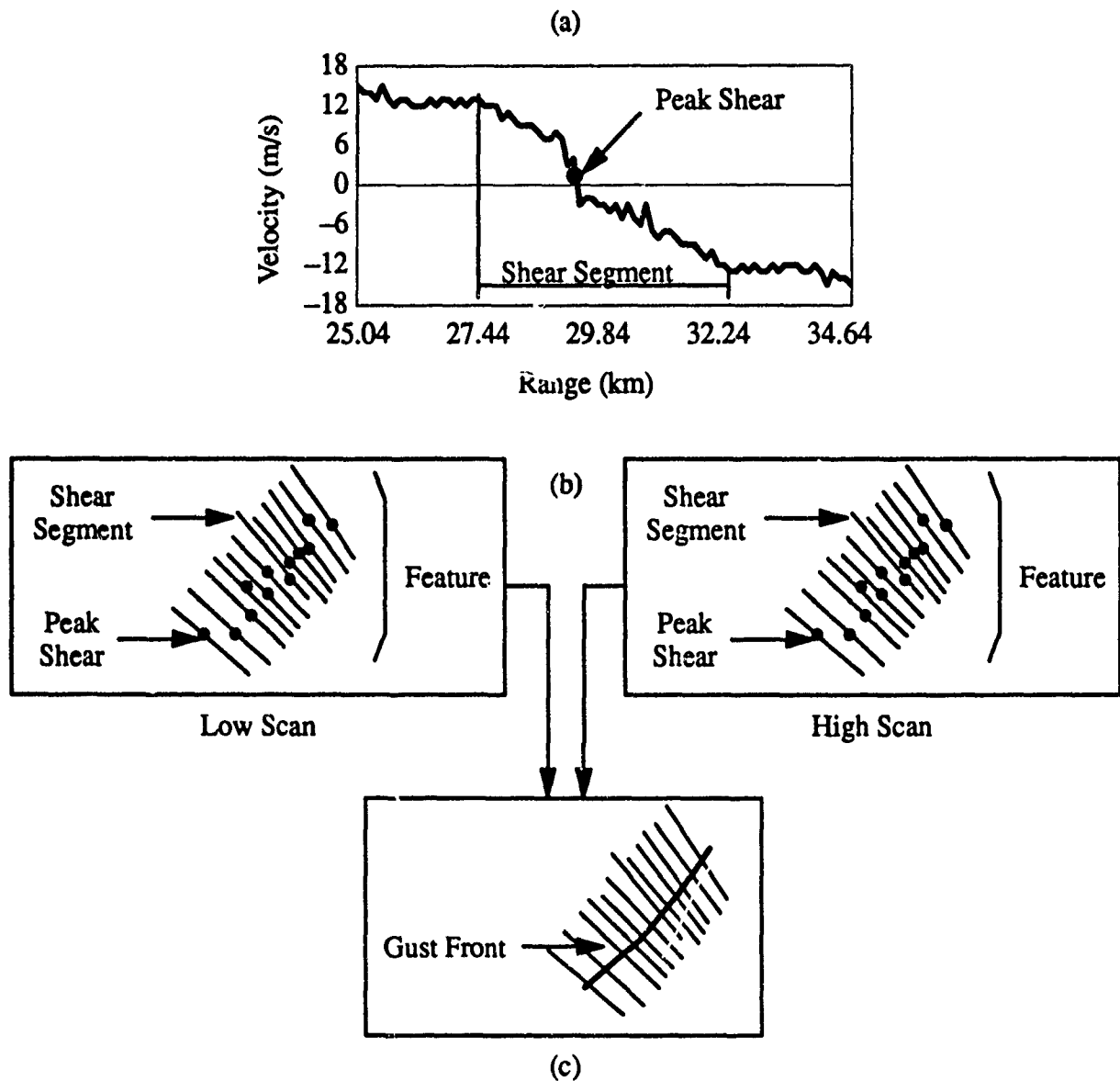
Figure 1. Diagram illustrating gust front detection. (a) Radial velocity data are searched for segments of decreasing Doppler velocity, which indicate radial convergence. The dots represent the locations of the peak shears along each segment. (b) Segments from the low and high scans are associated into features, and (c) features are grouped together based on spatial proximity into gust fronts.
