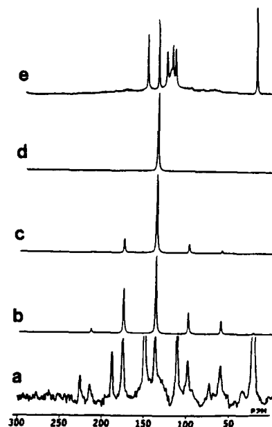
✓ Figure 8. Experimental and simulated ^{13}\text{C} MAS spectrum probing motion in the mesomorphic phase of PB3MP: (a) cross polarization spectrum with interrupted decoupling spectrum showing C3, C1, and \text{CH}_3 in the crystalline phase; (b) simulated spectrum of C3 showing the effect of motion \phi_1 ; (c) simulated spectrum of C3 showing the effect of \phi_1 and \phi_2 ; (d) simulated spectrum of C3 showing the effect of \phi_1 , \phi_2 , and \phi_3 ; (e) Bloch decay spectrum of PB3MP showing all signals from the mesomorphic phase. The cross polarization and Bloch decay spectra were obtained at -50 and 23^\circ\text{C} , respectively. All spectra are at a spinning speed of 2900 Hz.
