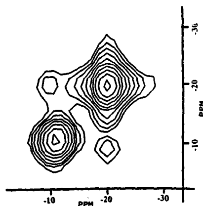
✓ Figure 4. ^{31}\text{P} 2D exchange spectrum of PB3MP at 23 °C using a 2-s mixing time. The cross peaks connecting the diagonal resonances for the two phases confirm the existence of a magnetization transfer process.
