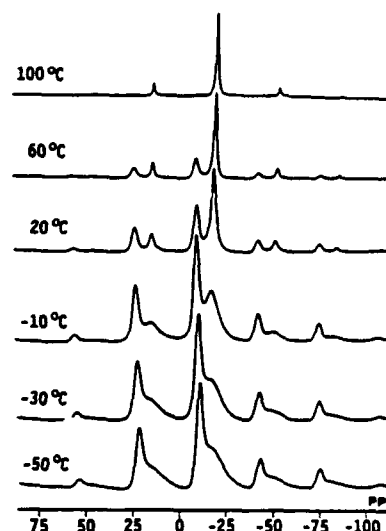
Figure 1. Variable-temperature ^{31}\text{P} MAS Bloch decay spectra of PB3MP showing isotropic peaks at -10.7 ppm (crystalline) and -19.4 ppm (mesomorphic) and their associated spinning sidebands.
