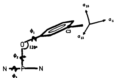
✓ Figure 7. Schematic diagram of the model used to interpret slow-speed ^{13}\text{C} MAS spectra of PB3MP in terms of molecular motion in the mesomorphic phase. \phi_1 , \phi_2 , and \phi_3 designate the three continuous diffusional processes used in simulations. The assumed orientation of the shielding tensor of C3 is indicated (see text).
