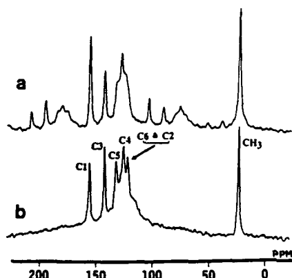
Figure 2. ^{13}\text{C} MAS NMR spectra of PB3MP using (a) cross polarization to emphasize the crystalline phase and (b) a 90^\circ pulse (Bloch decay) with a 20-s pulse delay to emphasize the mesomorphic phase. Assignments were made by analogy to m -cresol.
