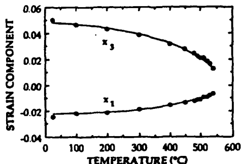
FIG. 2. Measured strain components, x_1 and x_3 , vs temperature for a c -axis oriented \text{PbTiO}_3 thin film.
