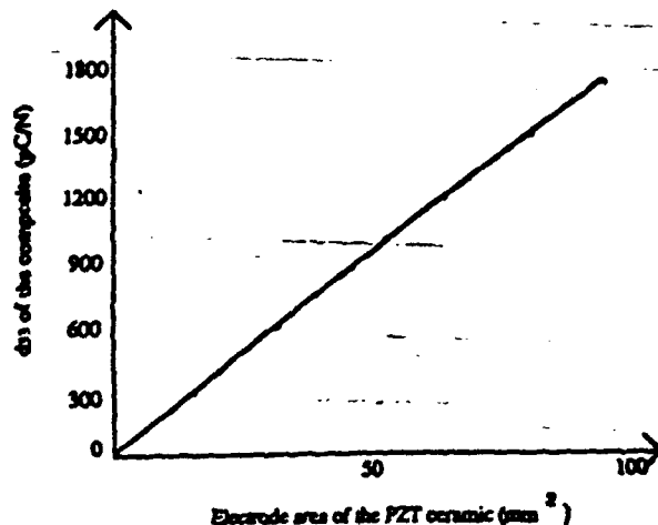
Figure 10. Effective d_{33} vs. electrode area of the ceramic.
