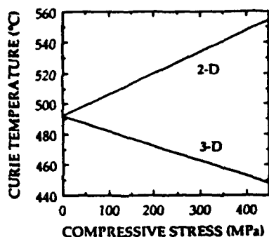
FIG. 1. Calculated shift of the Curie temperature for \text{PbTiO}_3 subjected to two-dimensional (2-D) compressive stress oriented orthogonal to the c axis and hydrostatic (3-D) compressive stress.
