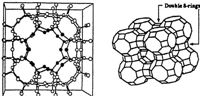
Figure 5. a) Zeolite RHO cage with 120 framework atoms; b) 3-d surface of interconnected cages.
