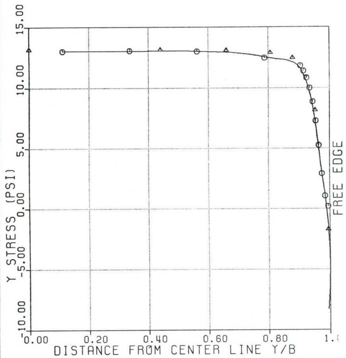
Figure 41: Y-stress at R5 for 22-layer coupon.
