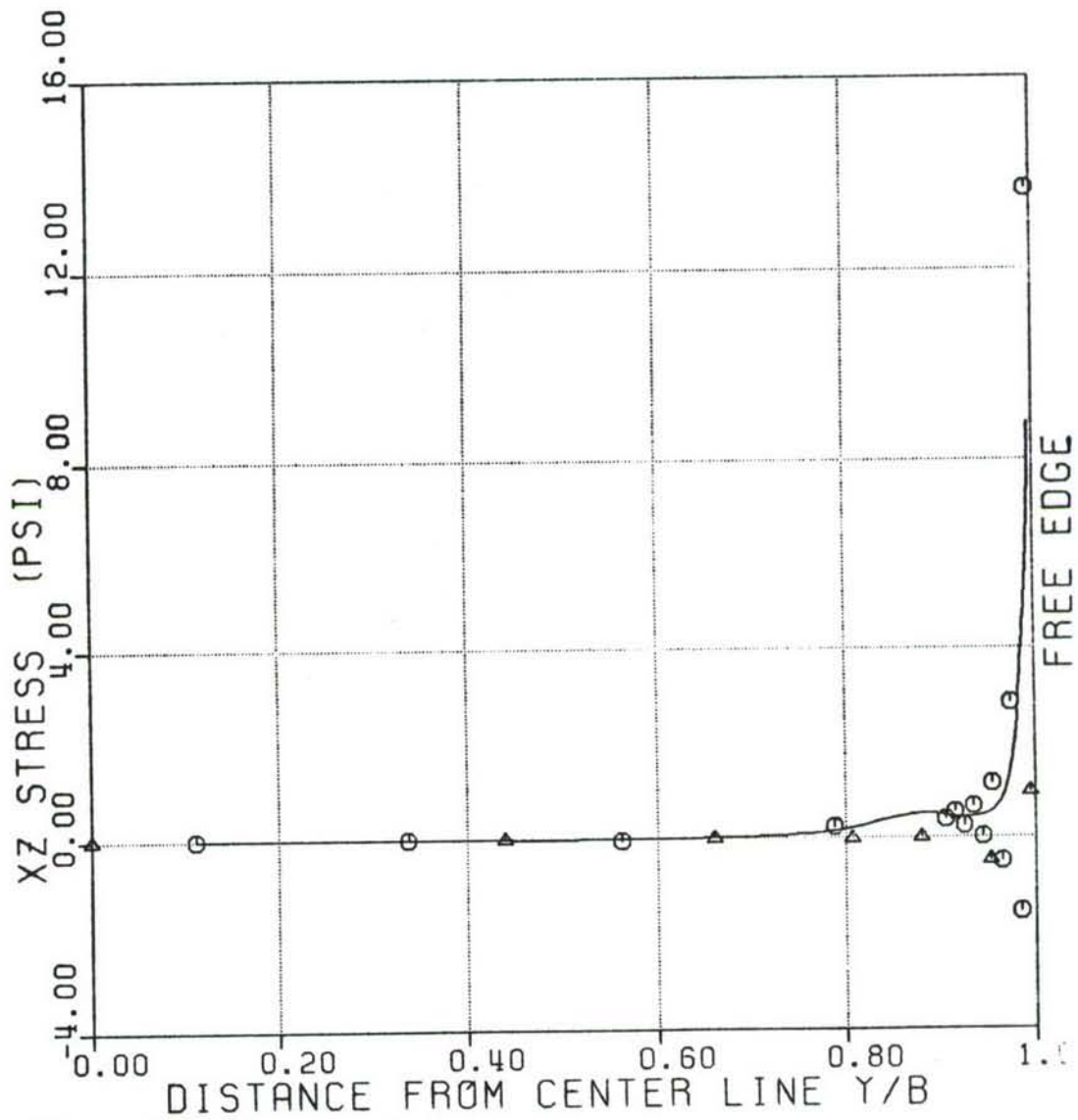
Figure 47: ZX-stress at R11 for 22-layer coupon.
