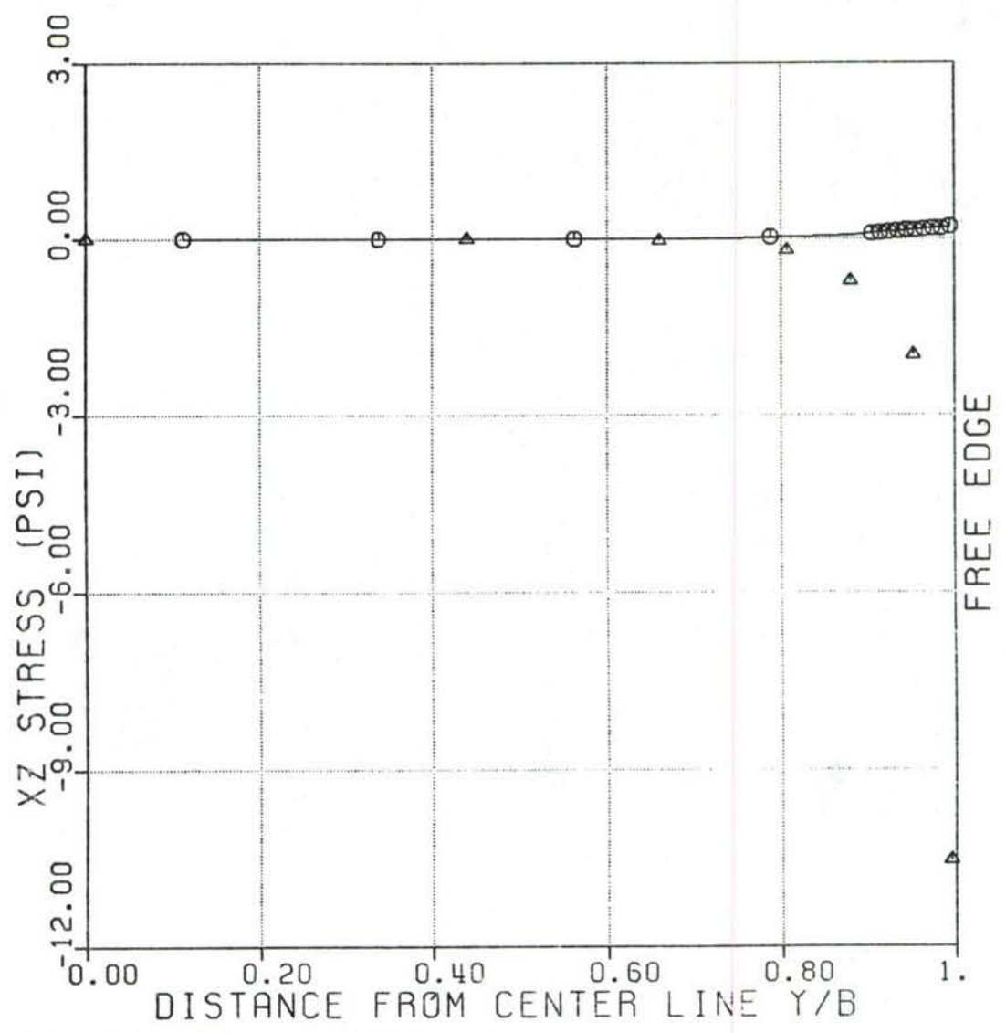
Figure 46: ZX-stress at R6 for 22-layer coupon.
