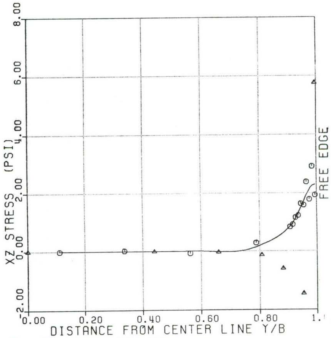
Figure 45: ZX-stress at R5 for 22-layer coupon.
