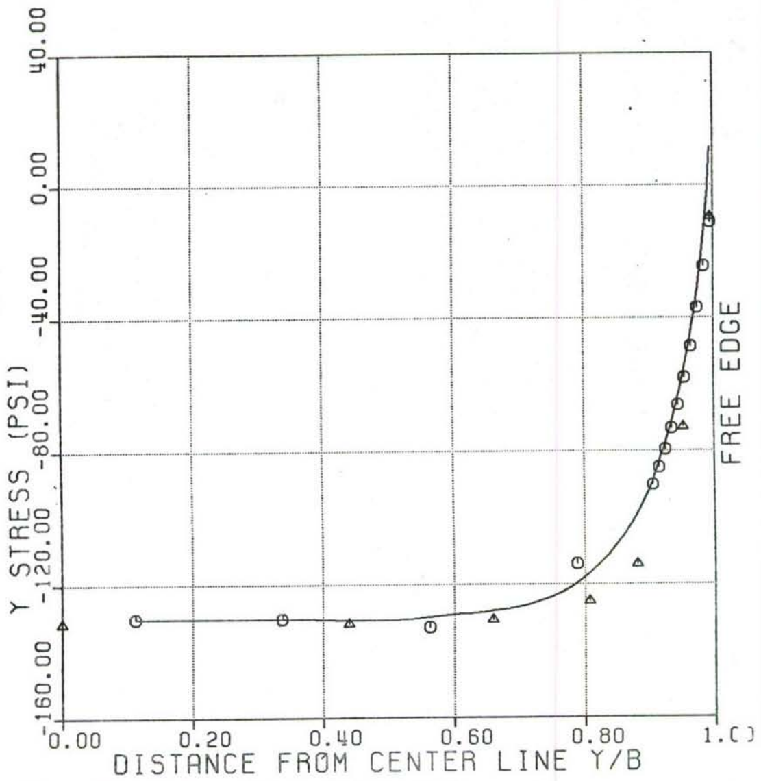
Figure 40: Y-stress at R1 for 22-layer coupon.
