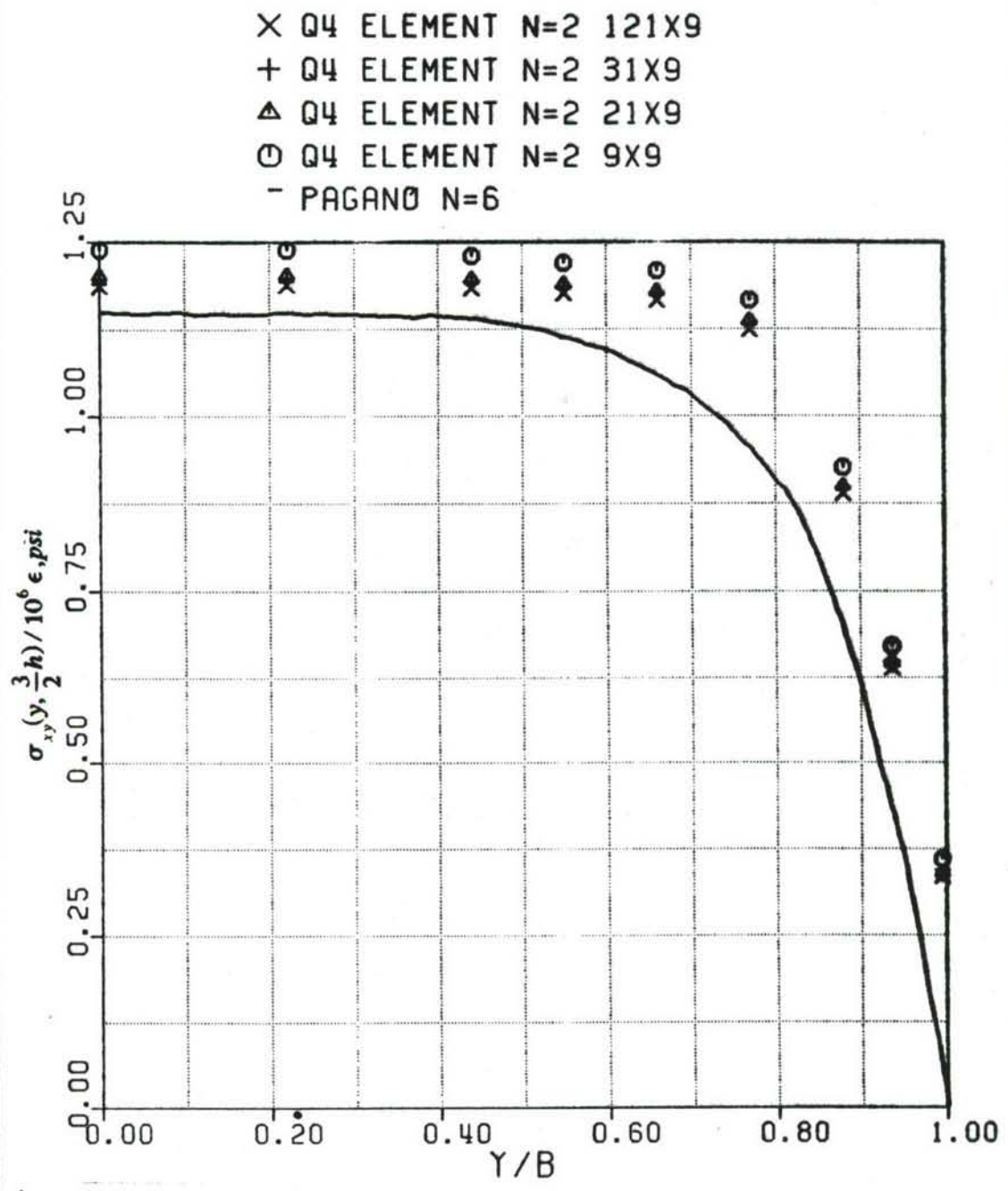
Figure 18: XY-stress at midsurface of top layer with refinement in x-direction; Angle-ply specimen.
