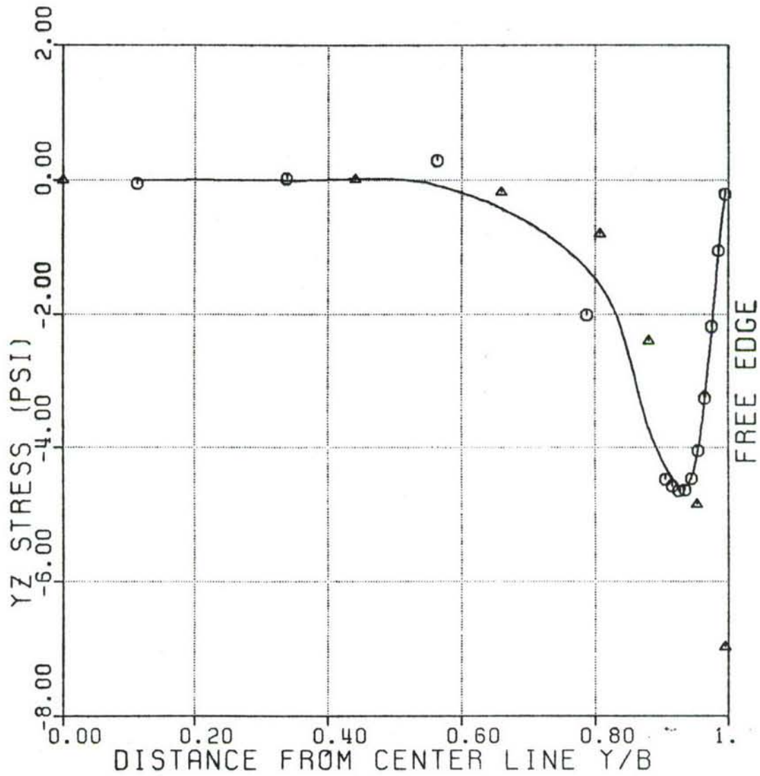
Figure 49: YZ-stress at R6 for 22-layer coupon.
