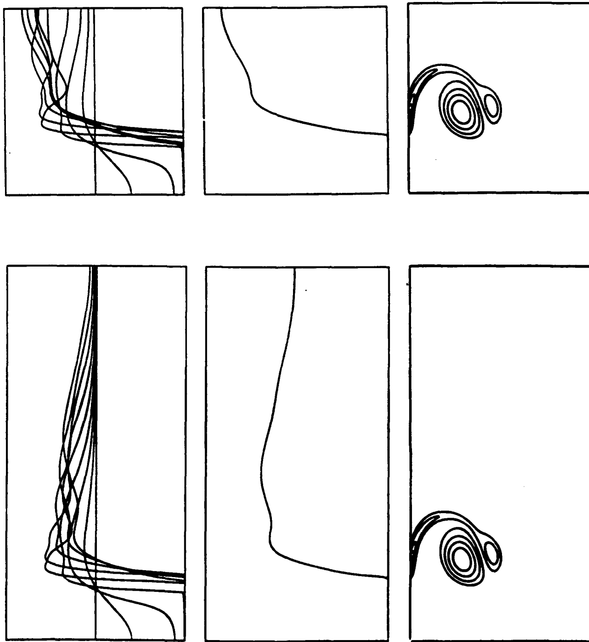
Figure 6. The solution for Re=1680 and W=0.95 at time 52.1 as calculated both in a short and a long computational domain. The contamination profiles are also
