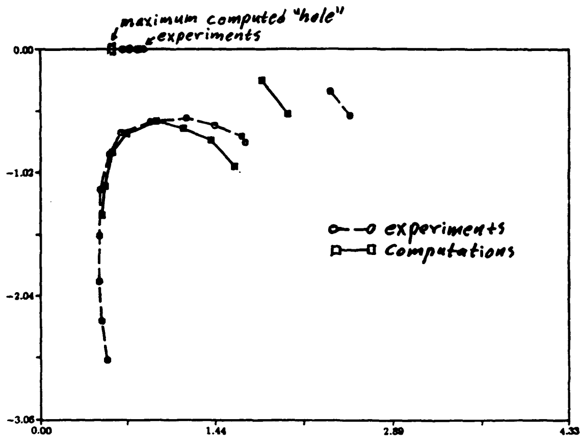
Figure 12. Comparison with experiments, Vortex paths, and the extend of the clean "hole" in the contaminant layer.
