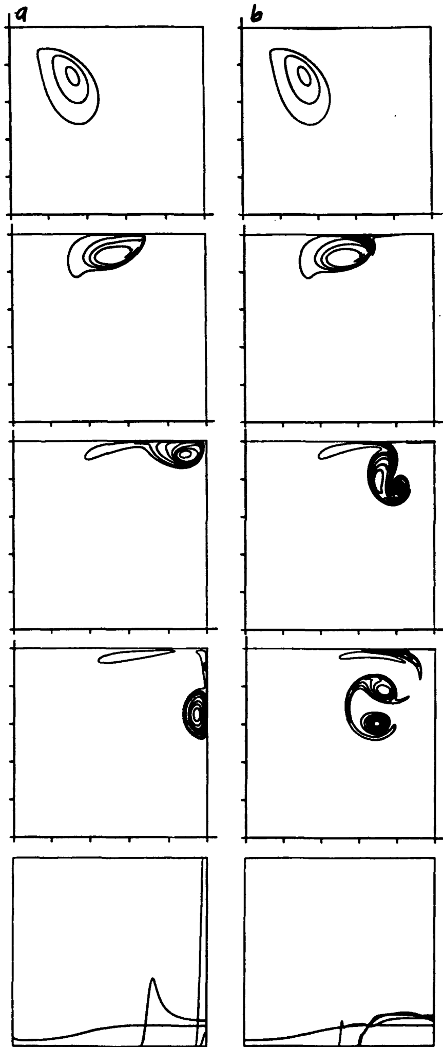
Figure 13. The evolution of an axisymmetric vortex ring (a) clean surface; (b) contaminated surface
