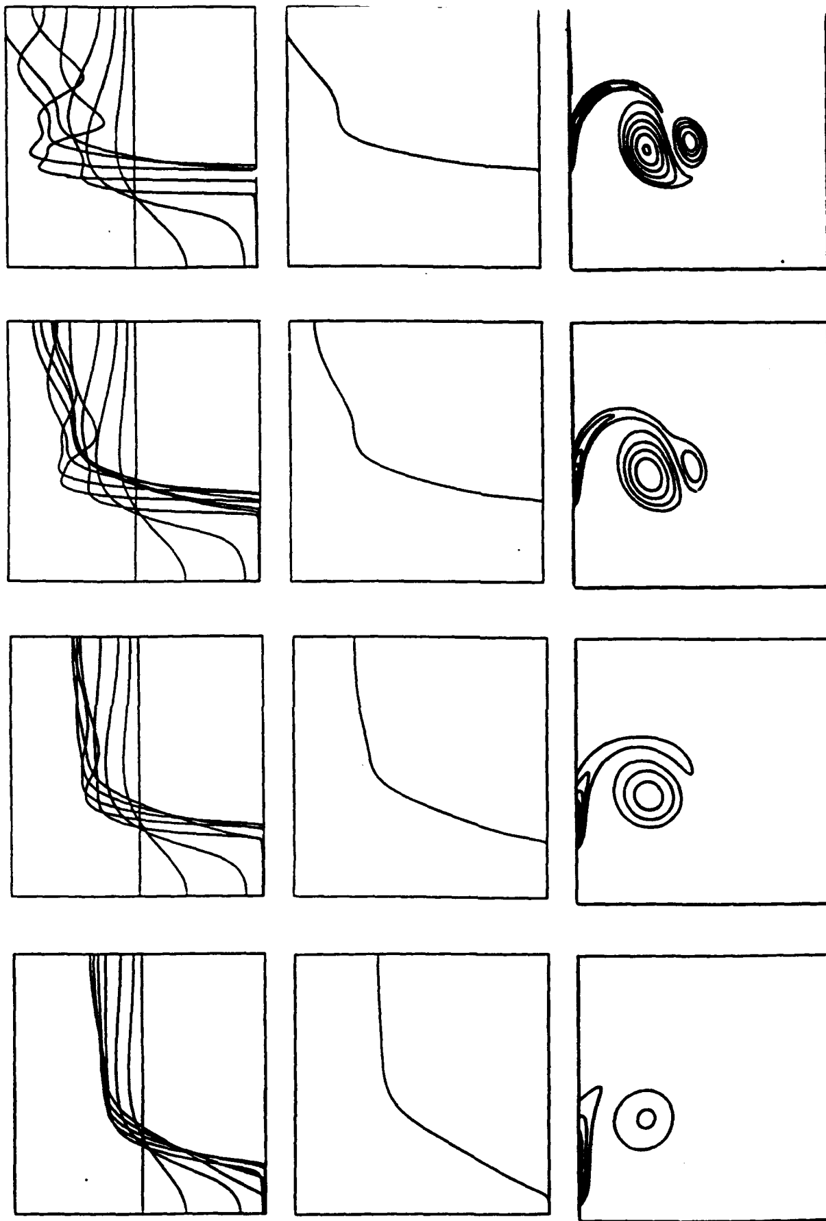
Figure 7. The effect of Reynolds number. (a) Re = 420 ; (b) Re = 840 ; (c) Re = 1680 ; (d) Re = 3360 . The vorticity and the contamination profiles at time 52.1 is shown, and several intermediate contamination profiles.
