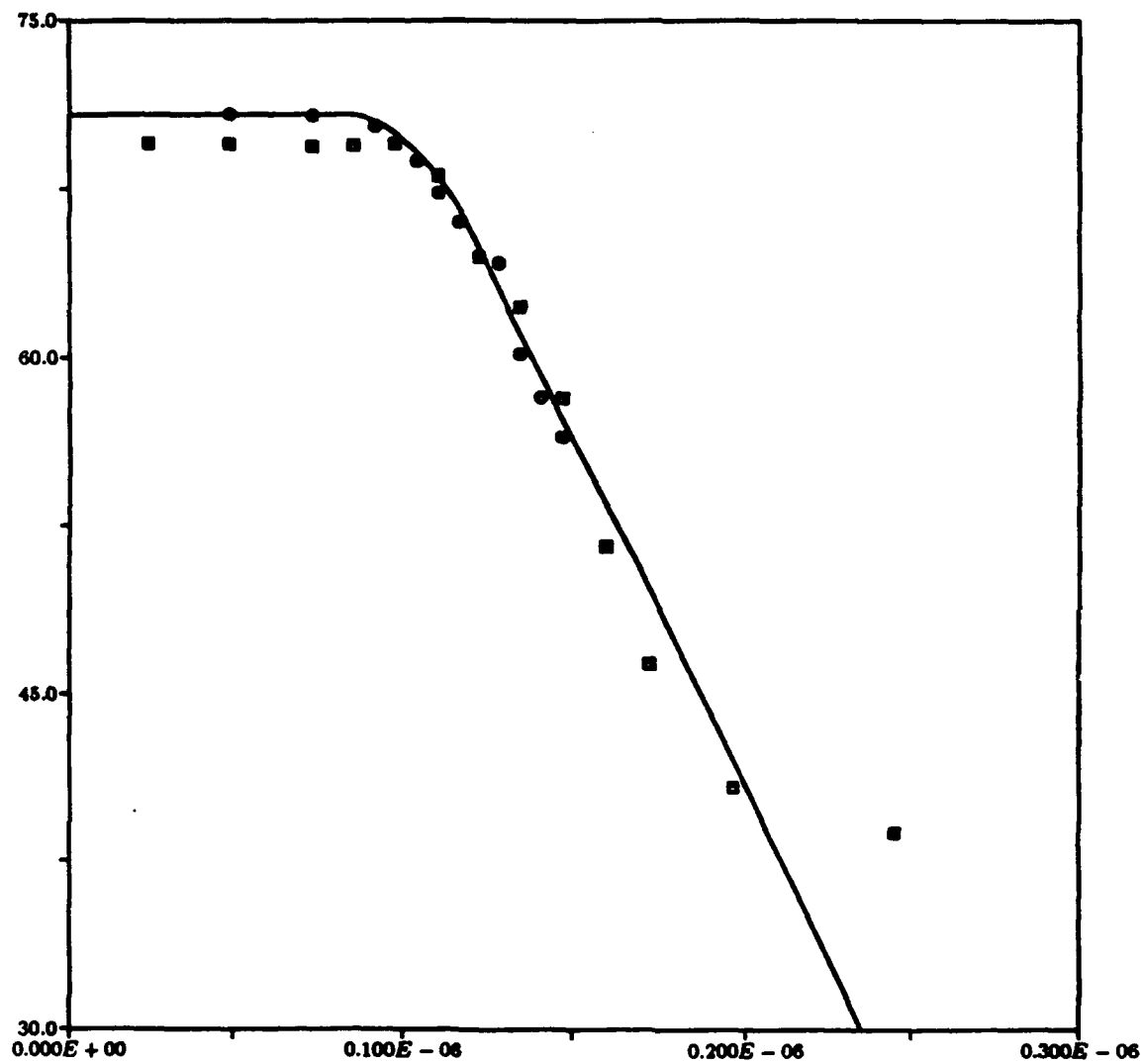
Figure 11. Comparison with experiments, analytical fit to the \sigma(c) curve and the measurements of Hirs (1990).
