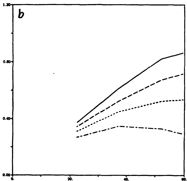
Figure 5. (a) The second moment of the contamination profile, \int (c - c_0)^2 dx versus time, for the runs in the previous figures. (b) The contaminant jump versus time, for the cases where a clean "hole" forms.
