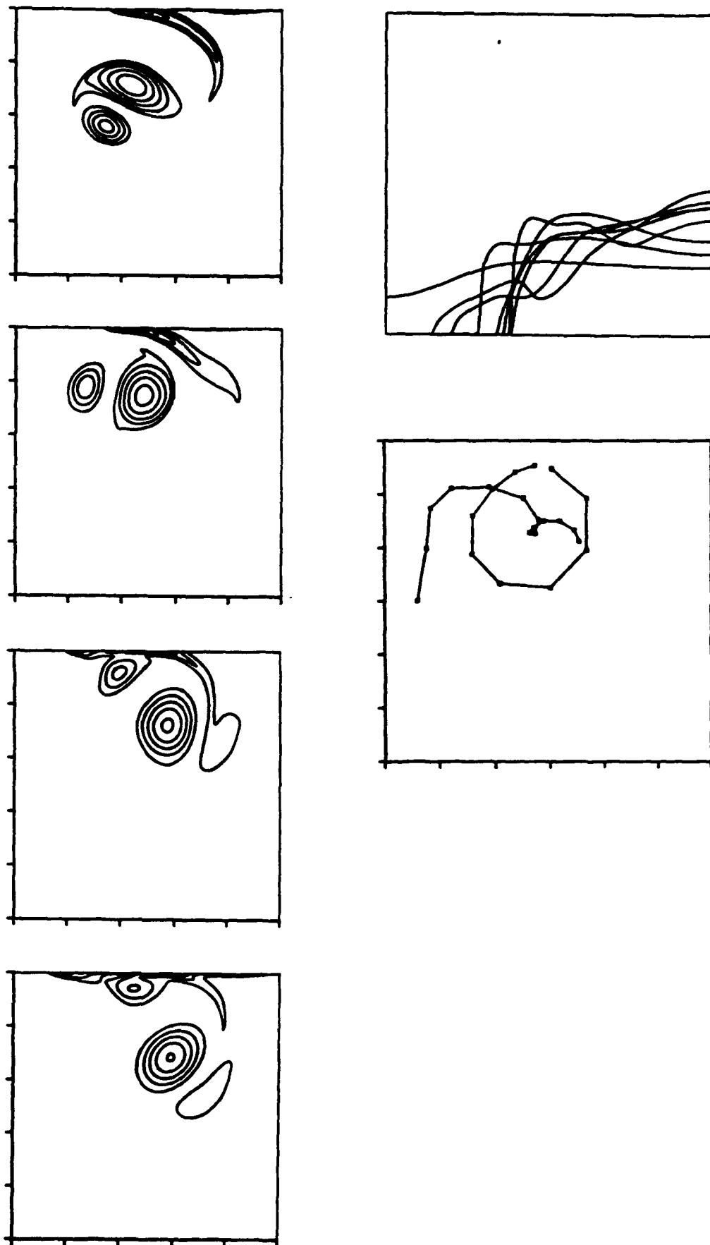
Figure 10. Long time evolution for Re = 3360 . (a) the vorticity at various times; (b) the corresponding contamination profiles; (c) Path of the vortices.
