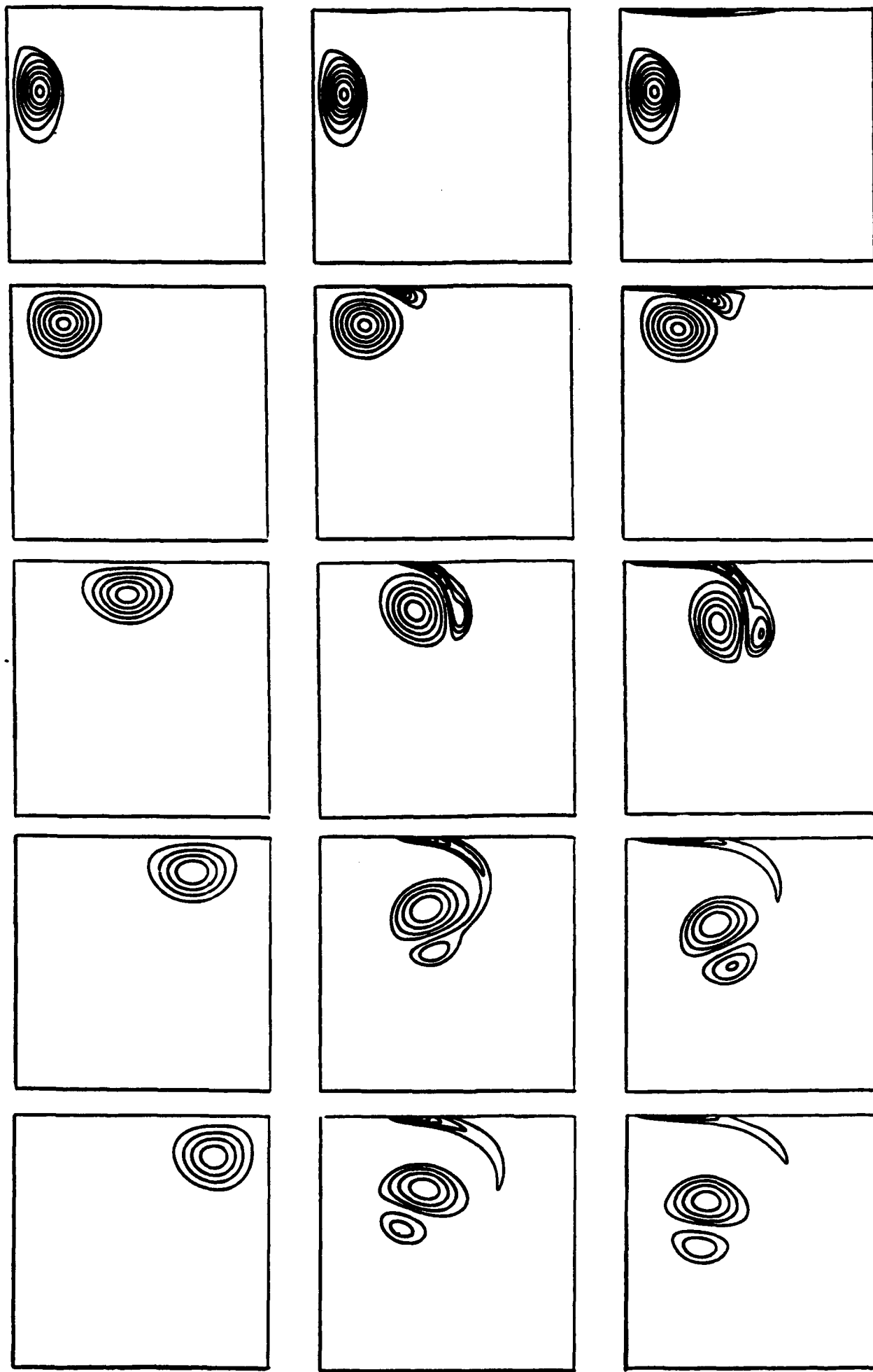
Figure 1. The collision of a vortex pair with a flat surface. Re = 1680 . The vorticity is shown at times (from the top): 7.4, 22.3, 37.2, 52.1, and 59.5. (a) Free-slip boundary; (b) Contaminated surface, W = 0.95 ; (c) No-slip boundary.
