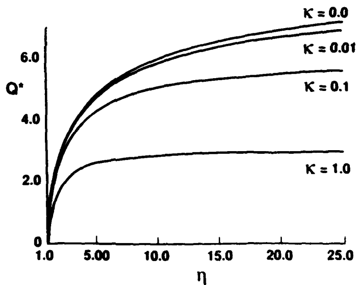
Figure B.4 Integral Heat Sink Versus Film Thickness for Several Values of \kappa .
