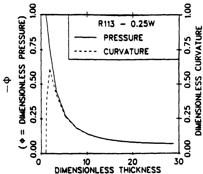
Figure 5.8 Plot of Dimensionless Pressure and Curvature vs. Dimensionless Film Thickness ( Q = 0.25W , \delta_0 = 4.8 nm, \pi_0 = 8.436 \times 10^2 N/m 2 ).
