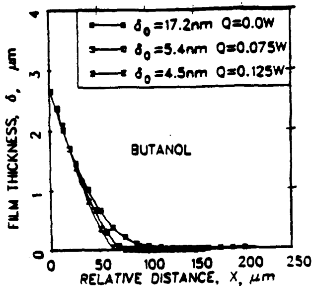
Figure 3.21 Film Thickness Profiles of Butanol on Silicon with a Native Surface Oxide. (With no heat input, \delta_0 \approx 17.2 nm and evaporation with controlled rate of heat inputs, \delta_0 = 5.4 nm and 4.5 nm).
