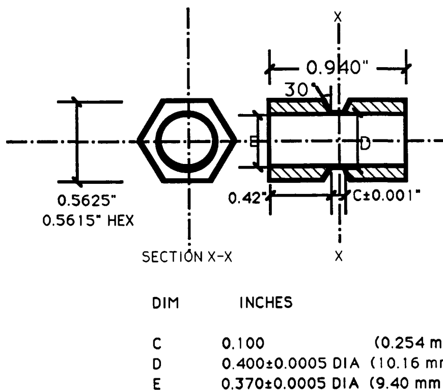
Figure 2. Specimen geometry.
