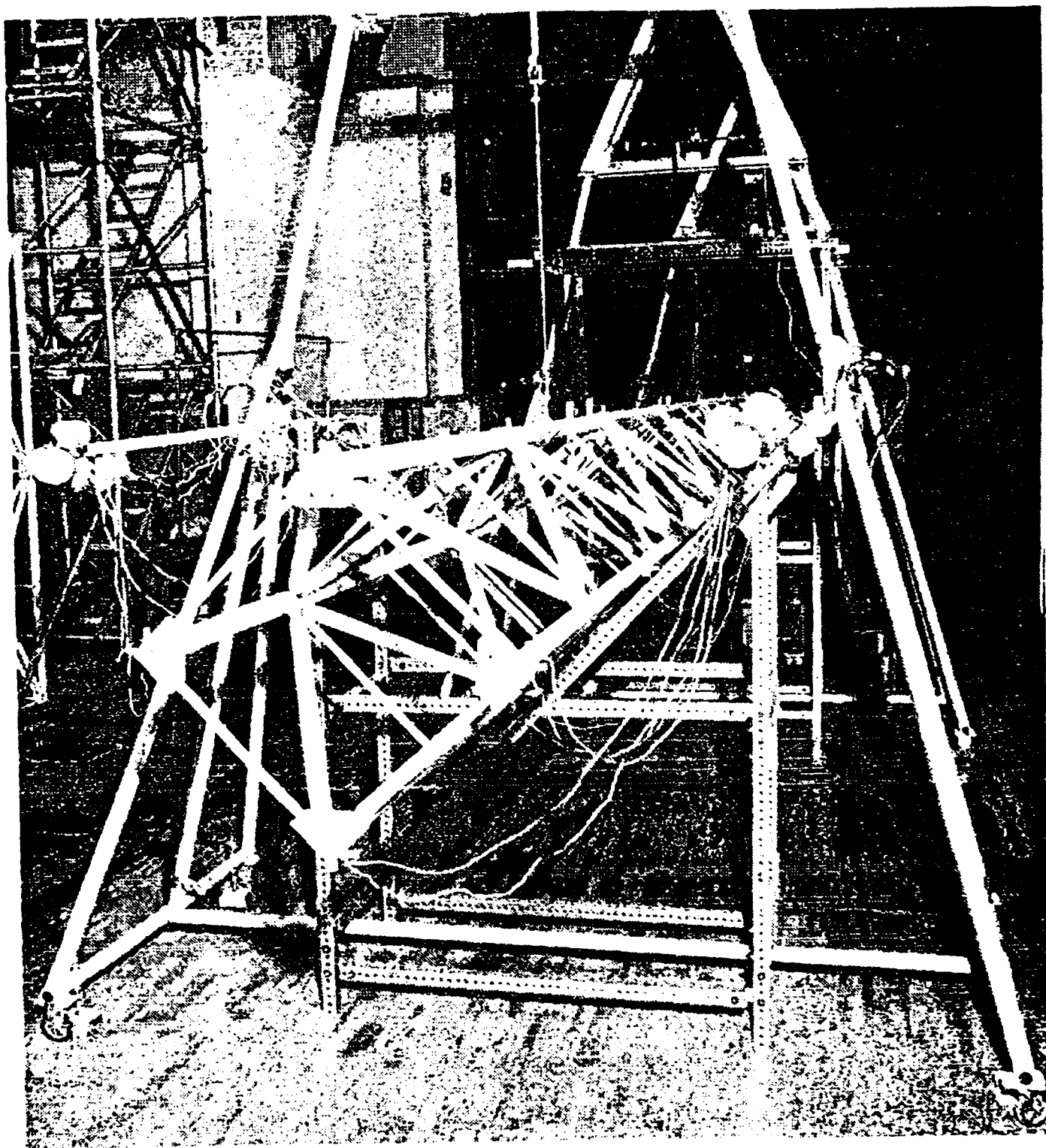
Figure 8. Horizontal Test of the Undamped 12-Meter Truss
