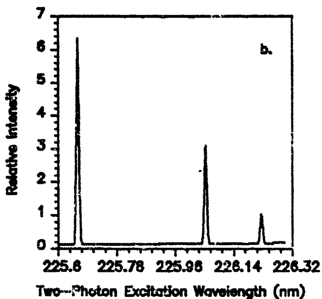
Figure 4b. Computer-Generated Excitation Spectrum Fit to a Thermodynamic Temperature of 1,000 \pm 200K.
