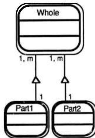
Figure I-4. Whole-Part Structure Notation
