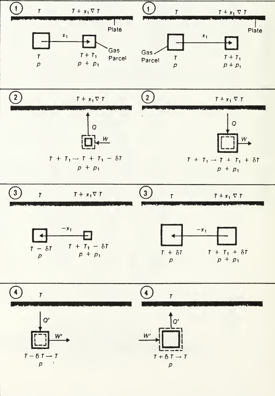
Figure 14: Schematic of the Acoustic Heat Engine Cycle (from Wheatley et al (1986))
