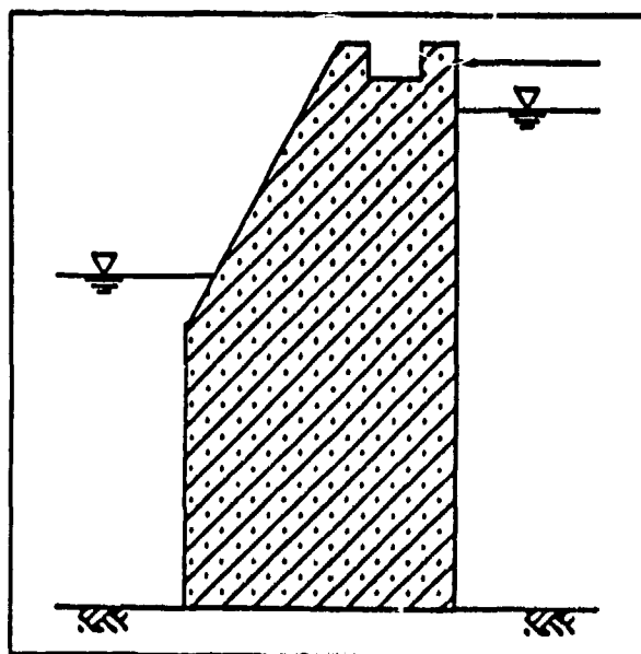
Figure A7. Cross sections through Emsworth R-4 and R-17, cases 14, 15, and 16
