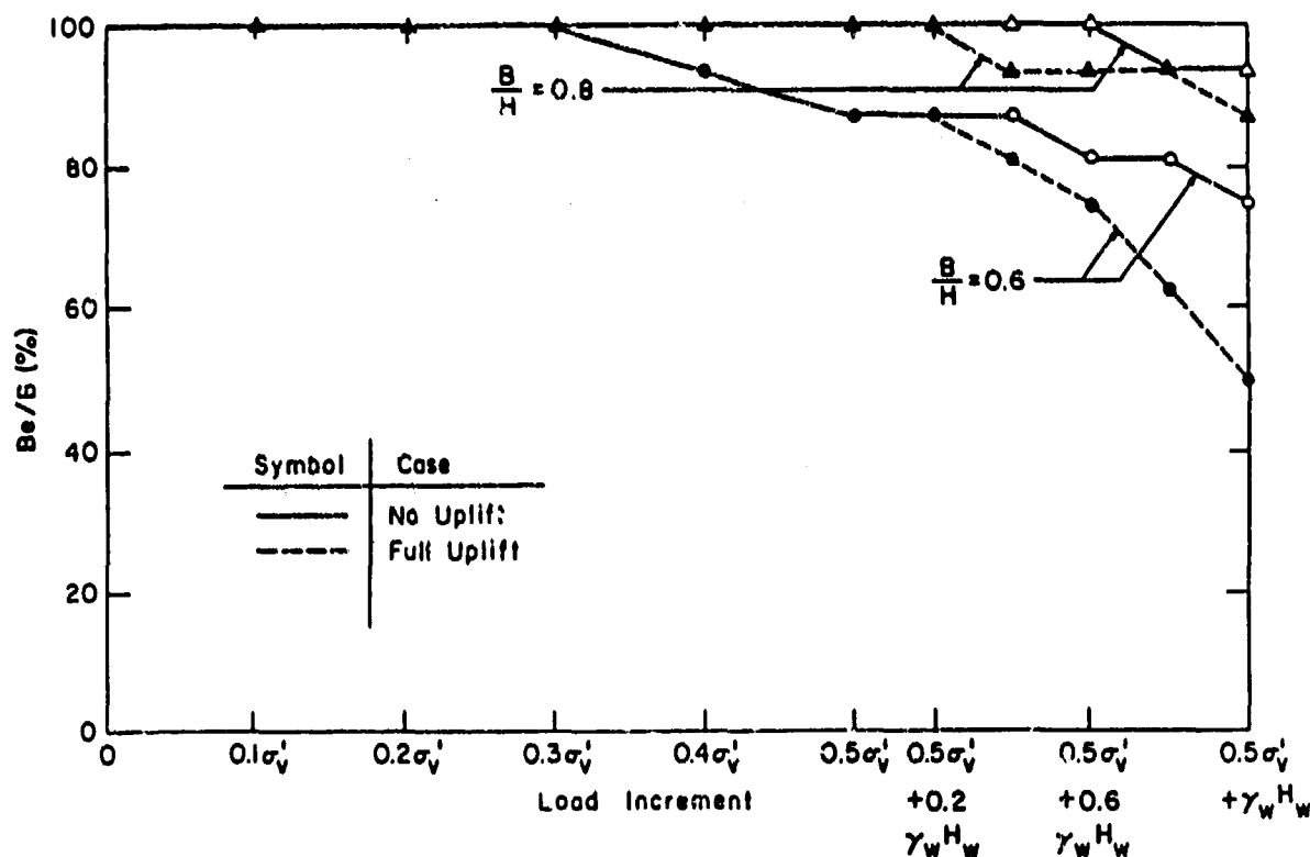
Figure 39. Variation of B_e/B with lateral load, walls with no uplift and full uplift pressures
