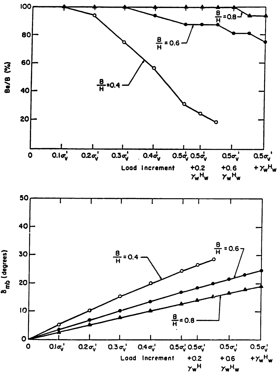
Figure 37. Variation of B_e/B and \delta_{bm} with lateral load, walls with B/H ratios equal to 0.4, 0.6, and 0.8
