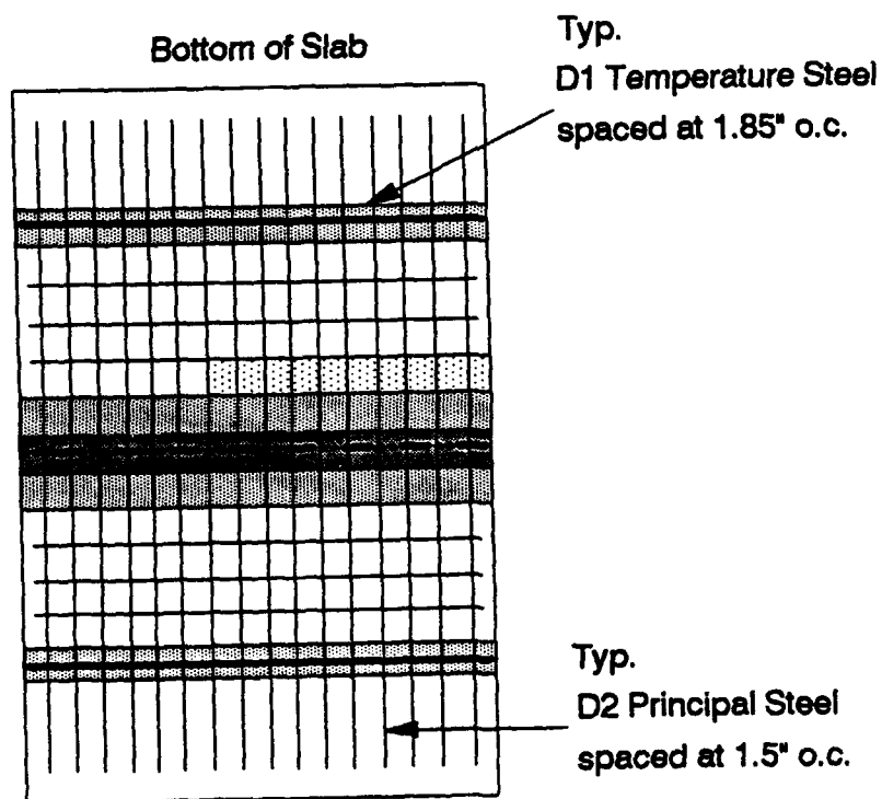
Figure 3.25. Damage Survey of Slab No. 7
