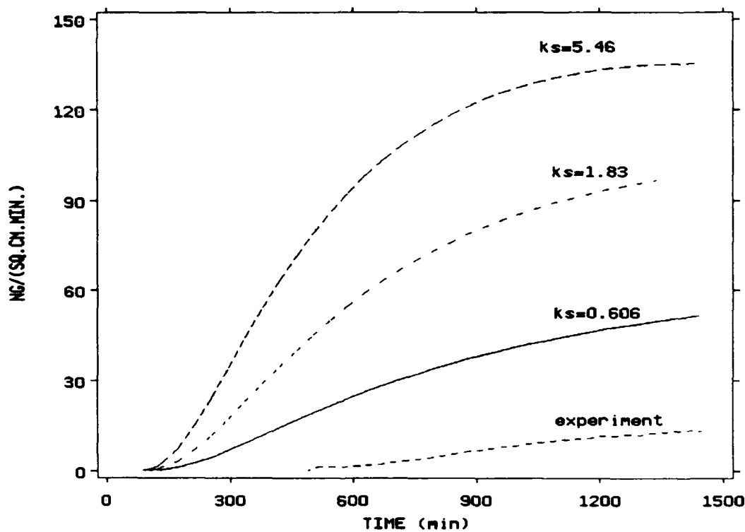
Figure 10. DIMP permeation rate vs. time for Neoprene membrane. L = 1.09 \times 10^{-1} cm; k_m = k_d = 0 ; sensitivity to assumed value of \hat{k}_r .
