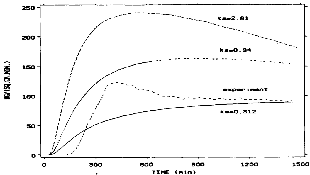
Figure 9. DIMP permeation rate vs. time for Neoprene membrane. L = 5.6 \times 10^{-2} cm; k_m = k_d = 0 ; sensitivity to assumed value of \hat{k}_r .
