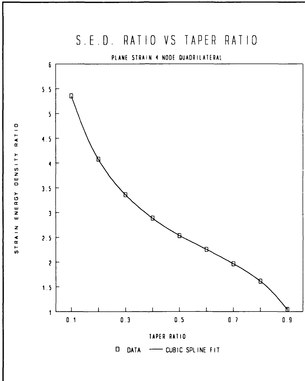
Figure 4.17. Strain energy density ratio versus taper ratio for a plane strain element
