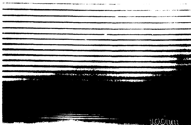
Fig. 10 — Transmission electron micrograph of multilayer film with alternating Si and \text{Si}_3\text{N}_4 layers deposited by IBAD at four different periodicities illustrating the excellent planarity and reproducibility of layer spacings
