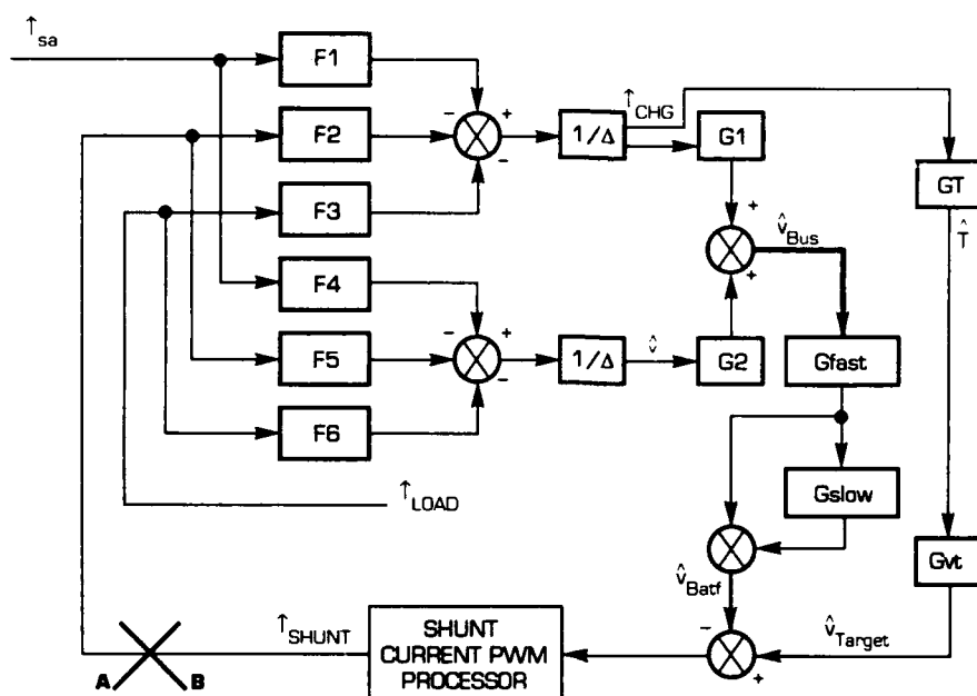
Fig. 11 — Spacecraft battery charger
