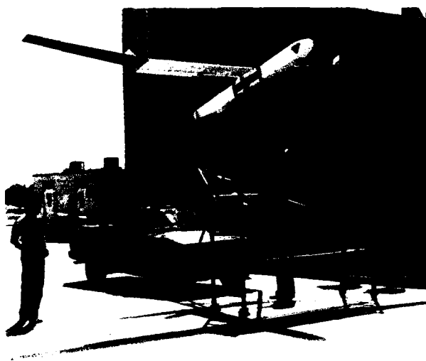
Fig. 6 — Captive carry test fixture with variable span LAURA installed
