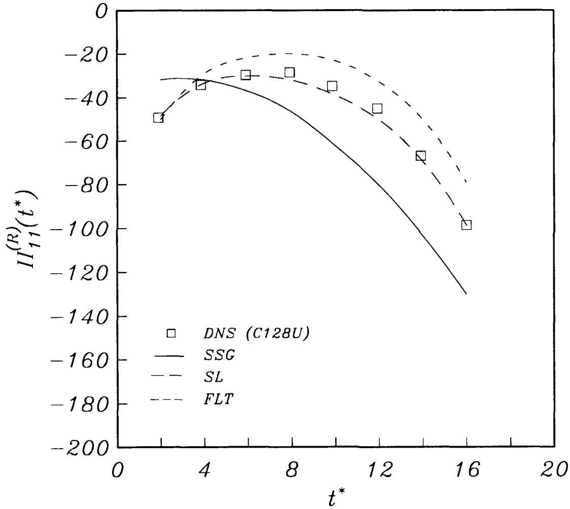
Figure 2. Comparison of the predictions of the SL, FLT and SSG models for the “rapid” pressure-strain correlation with the DNS results of Rogers et al. 9 for homogeneous shear flow (run C128U). (a) \Pi_{11}^{(R)} component, (b) \Pi_{12}^{(R)} component, and (c) \Pi_{22}^{(R)} component.
