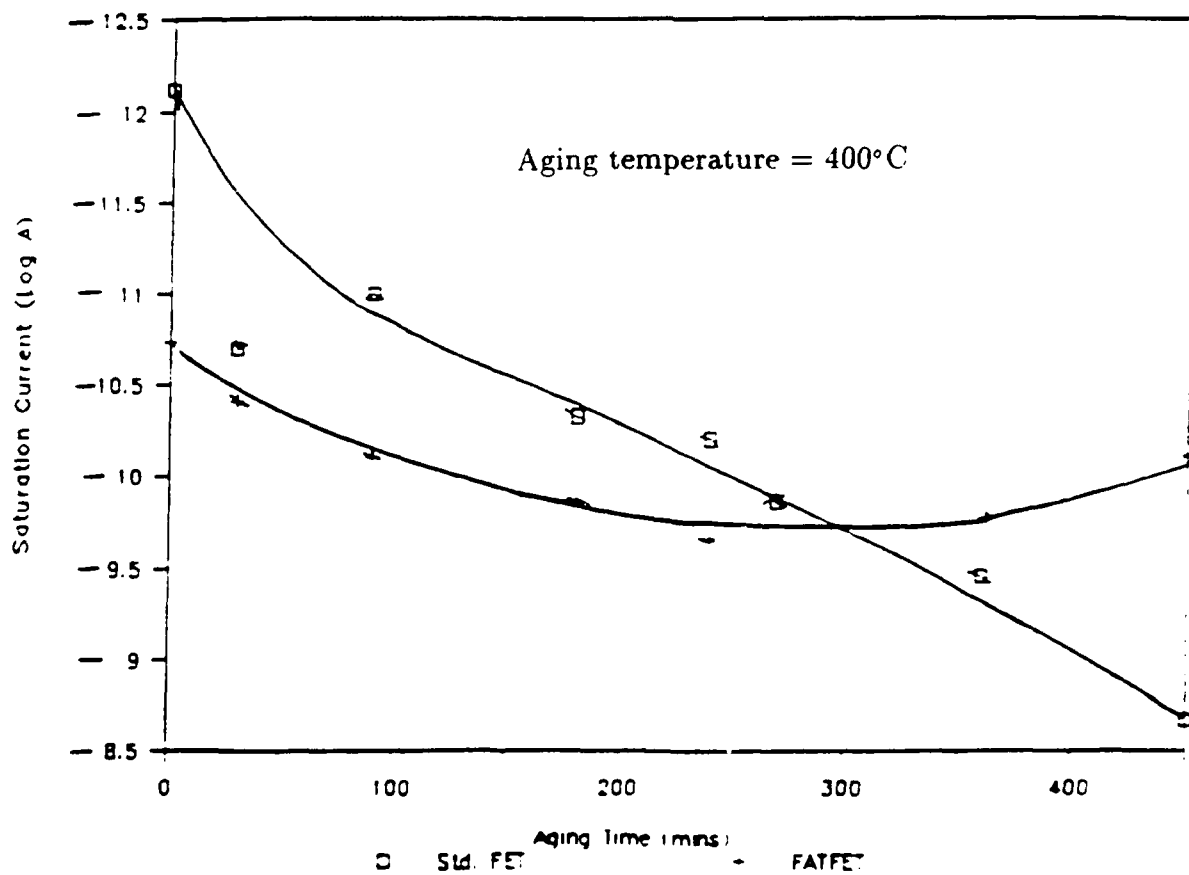
Fig.12(b) Variation of saturation current with aging time in Schottky contacts
