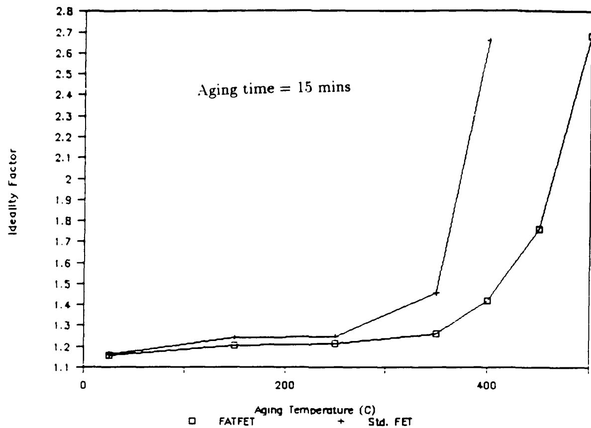
Fig.11(a) Variation of ideality factor with aging temperature in Schottky contacts.
