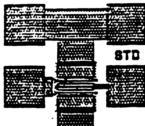
Fig.2 MESFET structures used for studies on Schottky contacts
