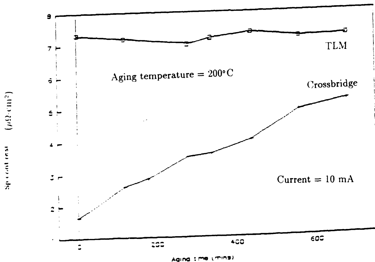
Fig.8 Variation of aging behavior in small area contacts.
