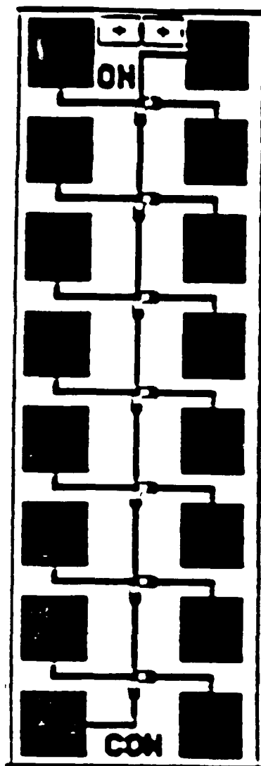
Fig.1 Test structures used for contact resistance measurement in ohmic contacts
