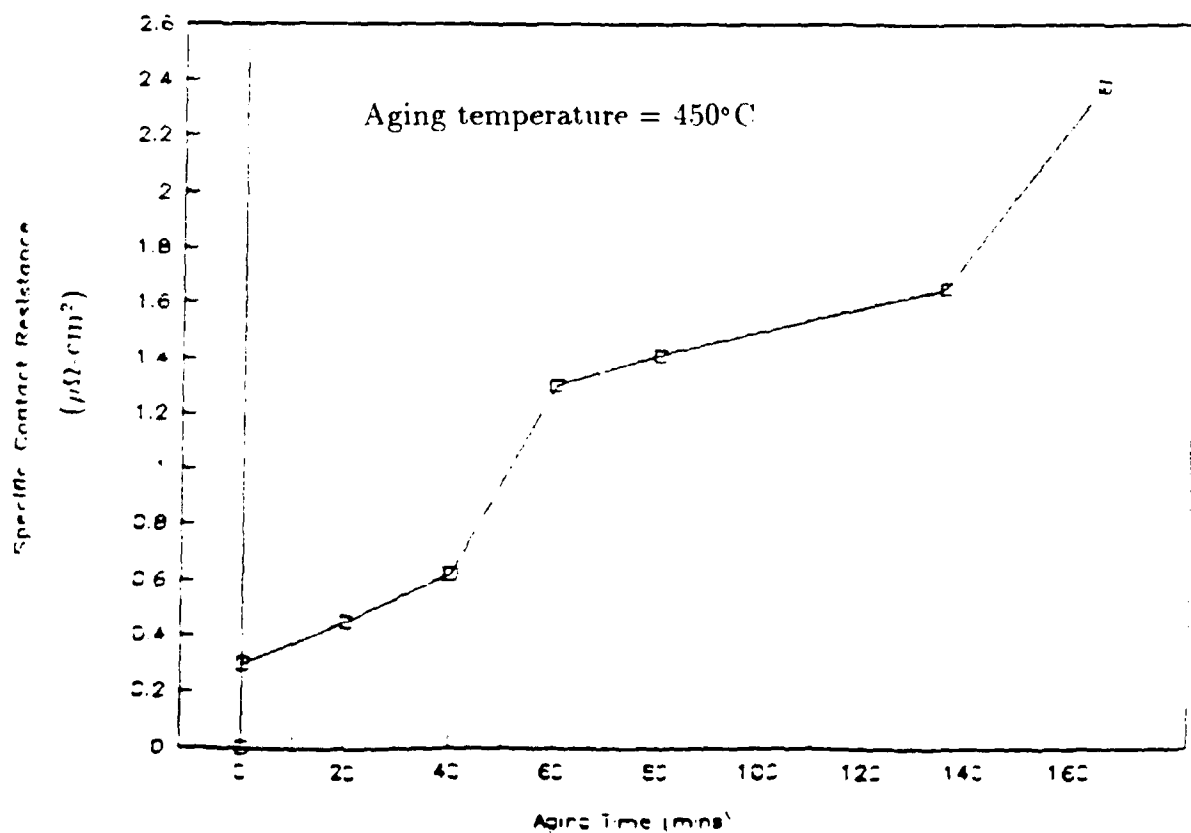
Fig.7 Variation of \rho_c with aging time in small area contacts
