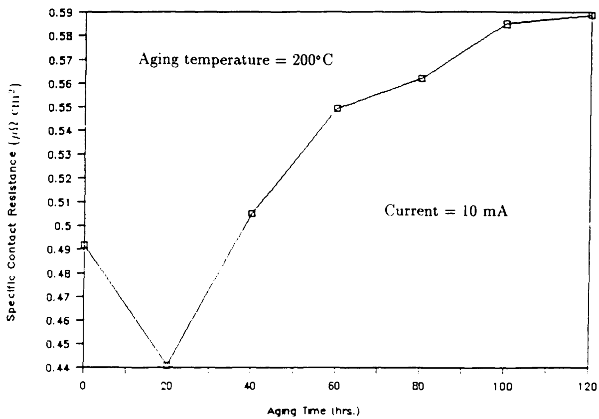
Fig.10 Aging behavior of small area contacts with low initial value of \rho_c , under applied electrical stress.
