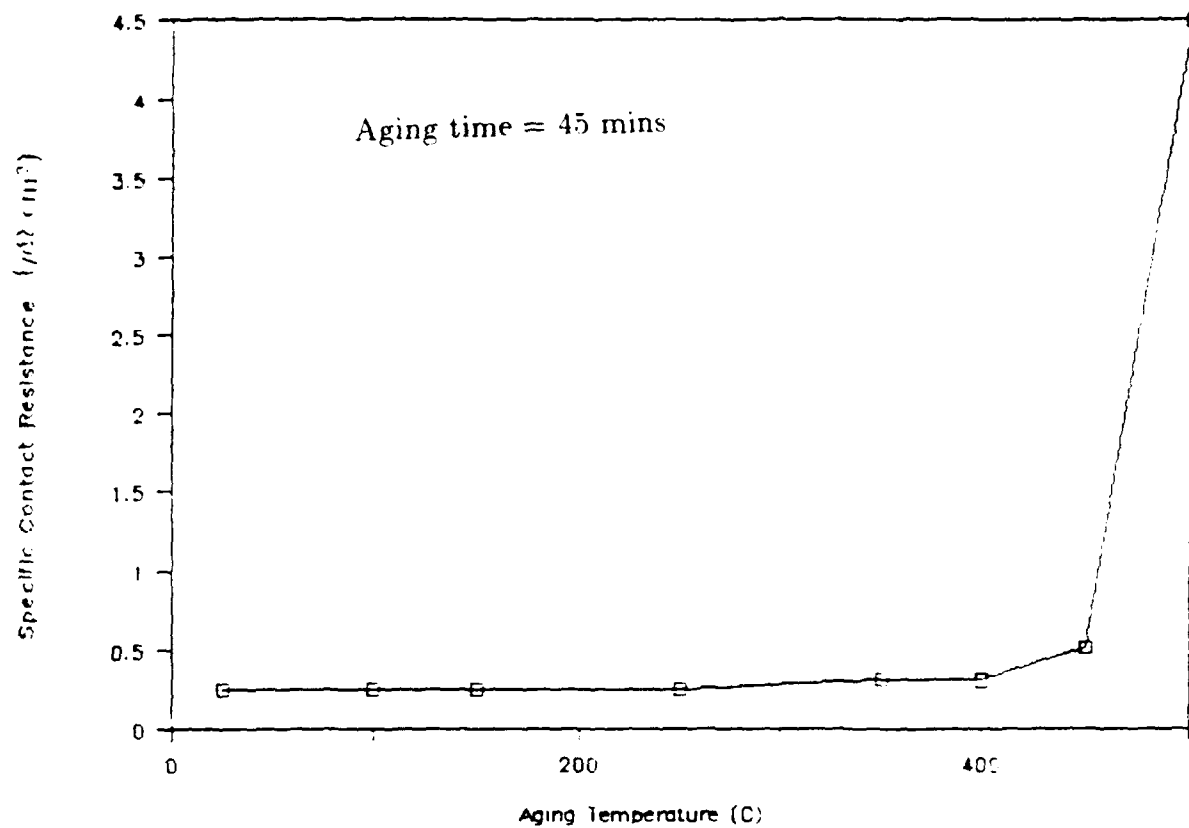
Fig.6 Variation of \rho_c with aging temperature in small area contacts
