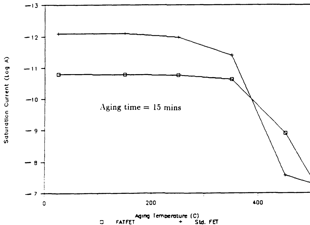
Fig.11(b) Variation of saturation current with aging temperature in Schottky contacts
