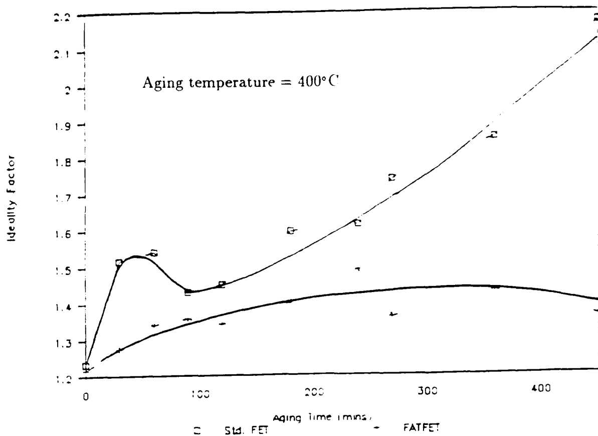
Fig.12(a) Variation of ideality factor with aging time in Schottky contacts
