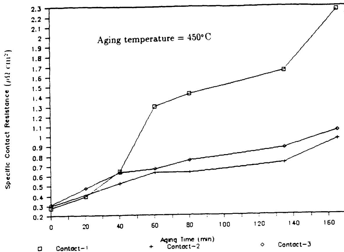
Fig.8 Variation of aging behavior in small area contacts.
