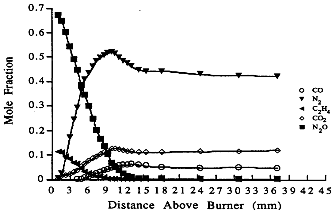
Figure 7. Concentration Profiles (in Mole Fraction) of Species Found by CID at m/z = 28 and 44 in Stoichiometric C_2H_4/N_2O/Ar Flame at 20 Torr. Compare to Total Ion Signals Prior to CID in Figure 6.
