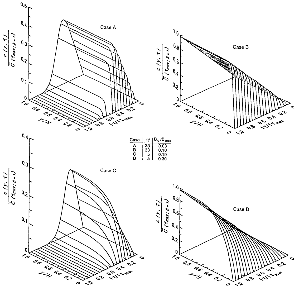
Figure 10. Normalized frazil concentration as a function of dimensionless depth and normalized dimensionless time for selected values of ft^* and B_c/B_{max} . Note the differences in the concentration scales.
