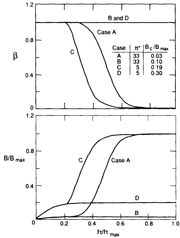
Figure 9. \beta and B/B_{max} as functions of normalized dimensionless time for selected values of fr^* and B_c/B_{max} .
