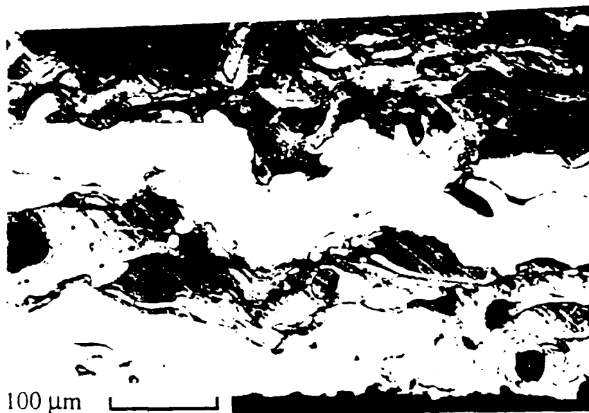
Fig. 12. Composite layered structure of 0.8% C steel and Invar.
