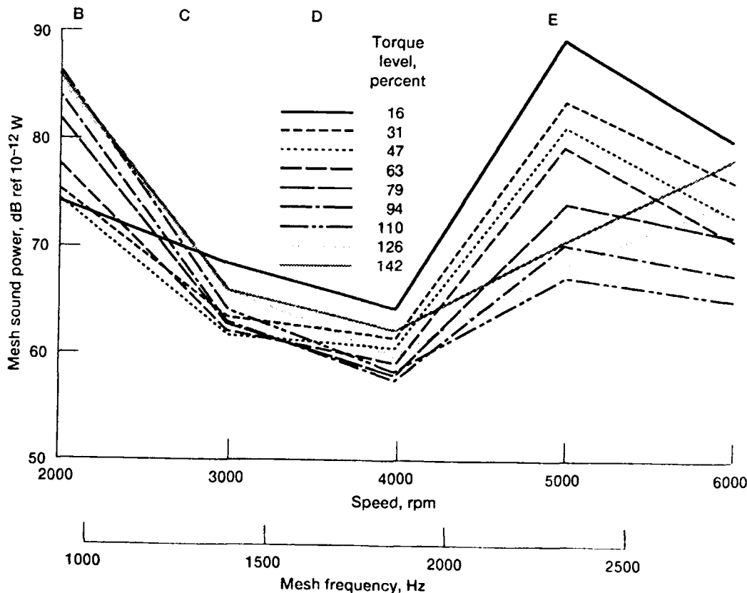
Figure 4.—Mesh sound power as a function of speed at 9 torque levels computed from the sum of values at mesh and at 3 pairs of sideband frequencies.
