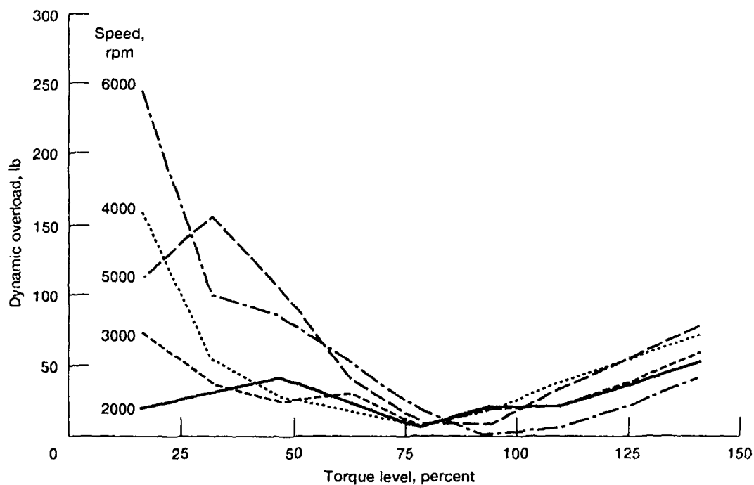
Figure 6.—Gear tooth dynamic overload predicted by DANST. Dynamic overload is computed from the difference between maximum tooth load and static tooth load.
