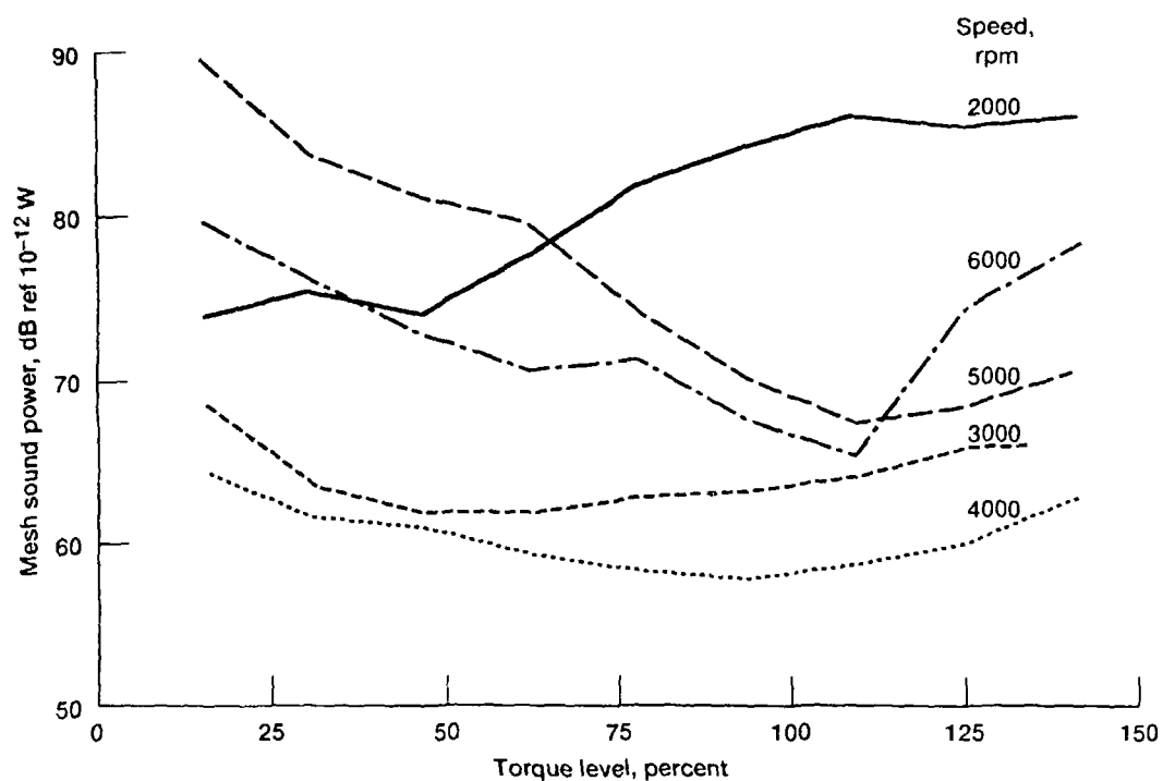
Figure 5.—Mesh sound power as a function of torque at 5 speeds computed from the sum of values at mesh and at 3 pairs of sideband frequencies.
