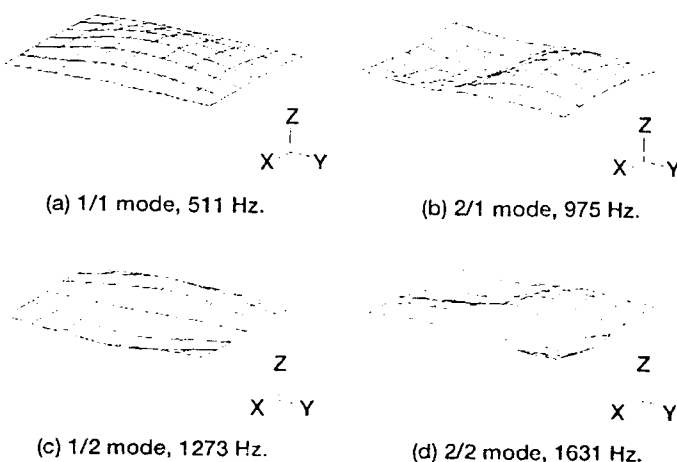
Figure 2.—Gearbox vibration modes.
