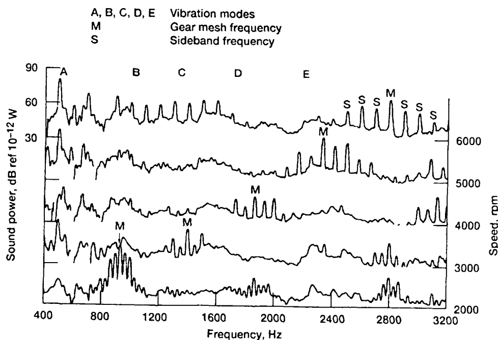
Figure 3.—Sound power measurements at 5 speeds (constant 94-percent torque level).
