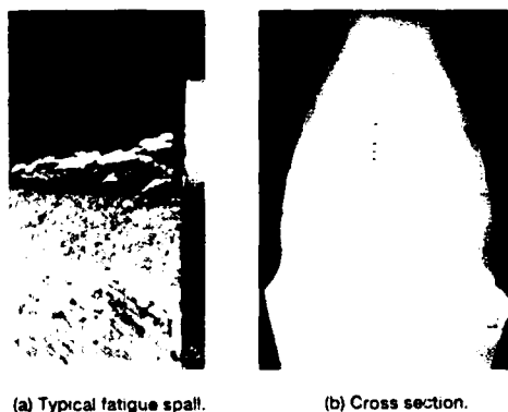
Figure 5.—Fatigue spall for medium-intensity-shot-peened gears.
