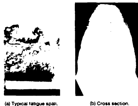
Figure 6.—Fatigue spall for high-intensity-shot-peened gears.
