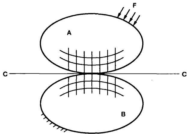
Figure 1.—Two typical bodies in contact.
