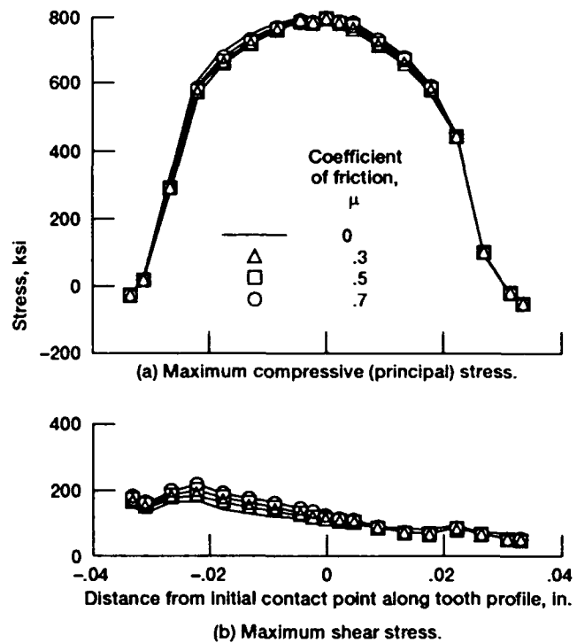
Figure 15.—Stresses on driving gear teeth.
