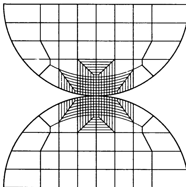
Figure 5.—Semicylinder finite element mesh.
