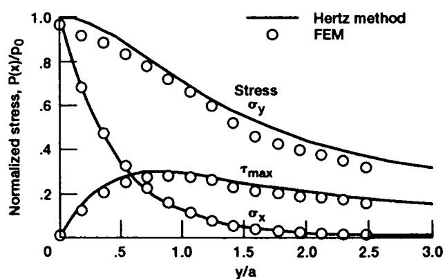
Figure 6.—Subsurface stresses along axis of symmetry. (Stress values are normalized by p_0 , the maximum normal contact pressure.)
