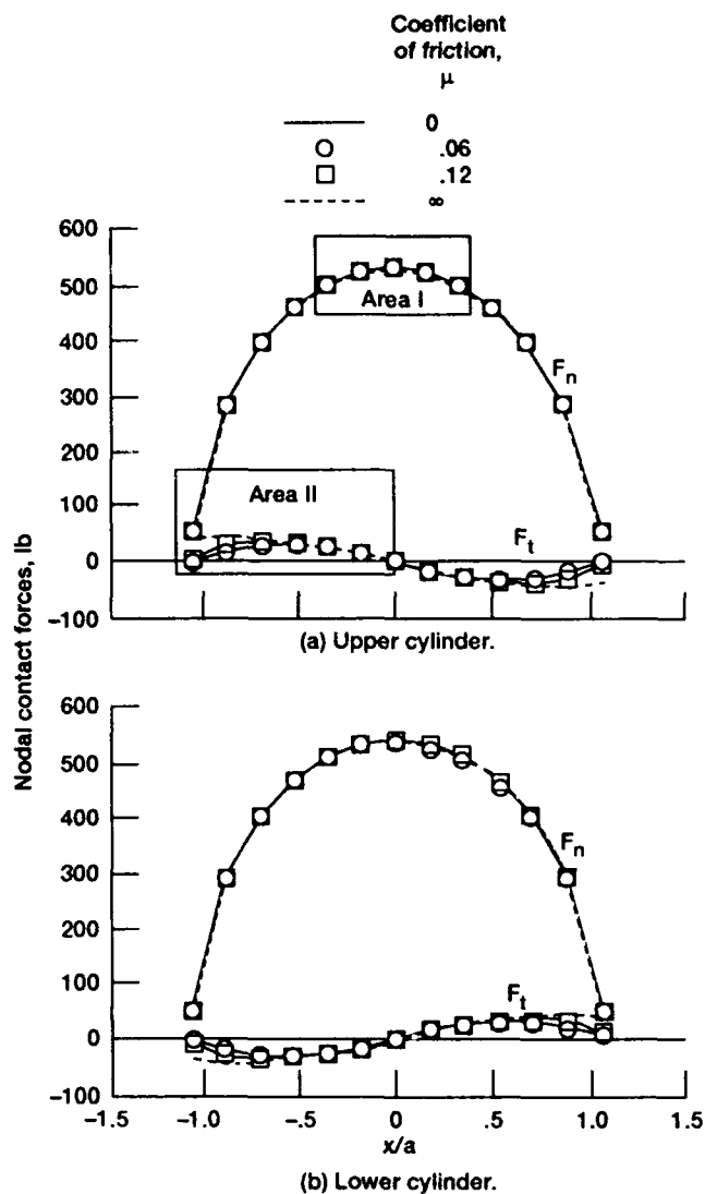
Figure 8.—Distribution of contact forces.
