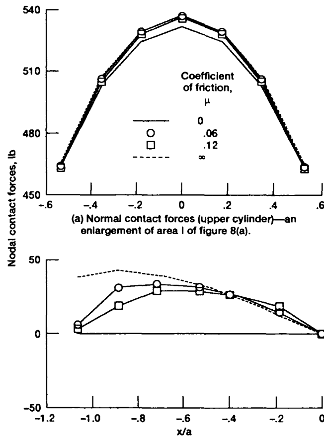
Figure 9.—Detailed representation of forces.
