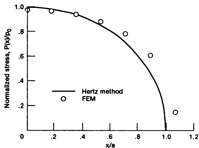
Figure 7.—Distribution of normal stress in contact surface. (Stress values are normalized by p_0 , the maximum normal contact pressure.)
