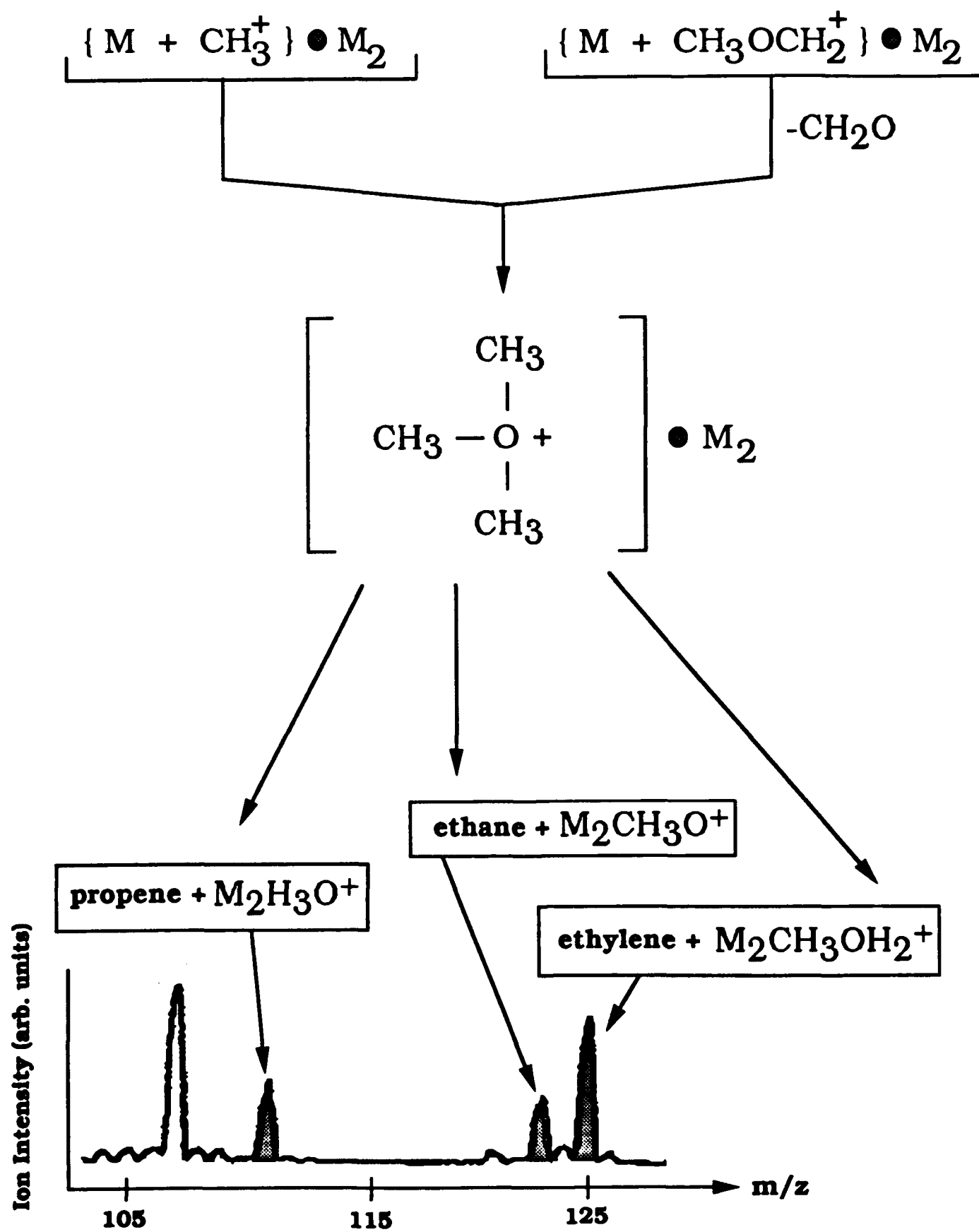
Figure 2. Fragmentation of the \{M + \text{CH}_3^+\} \bullet M_2 and \{M + \text{CH}_3\text{OCH}_2^+\} \bullet M_2 ion complexes.
