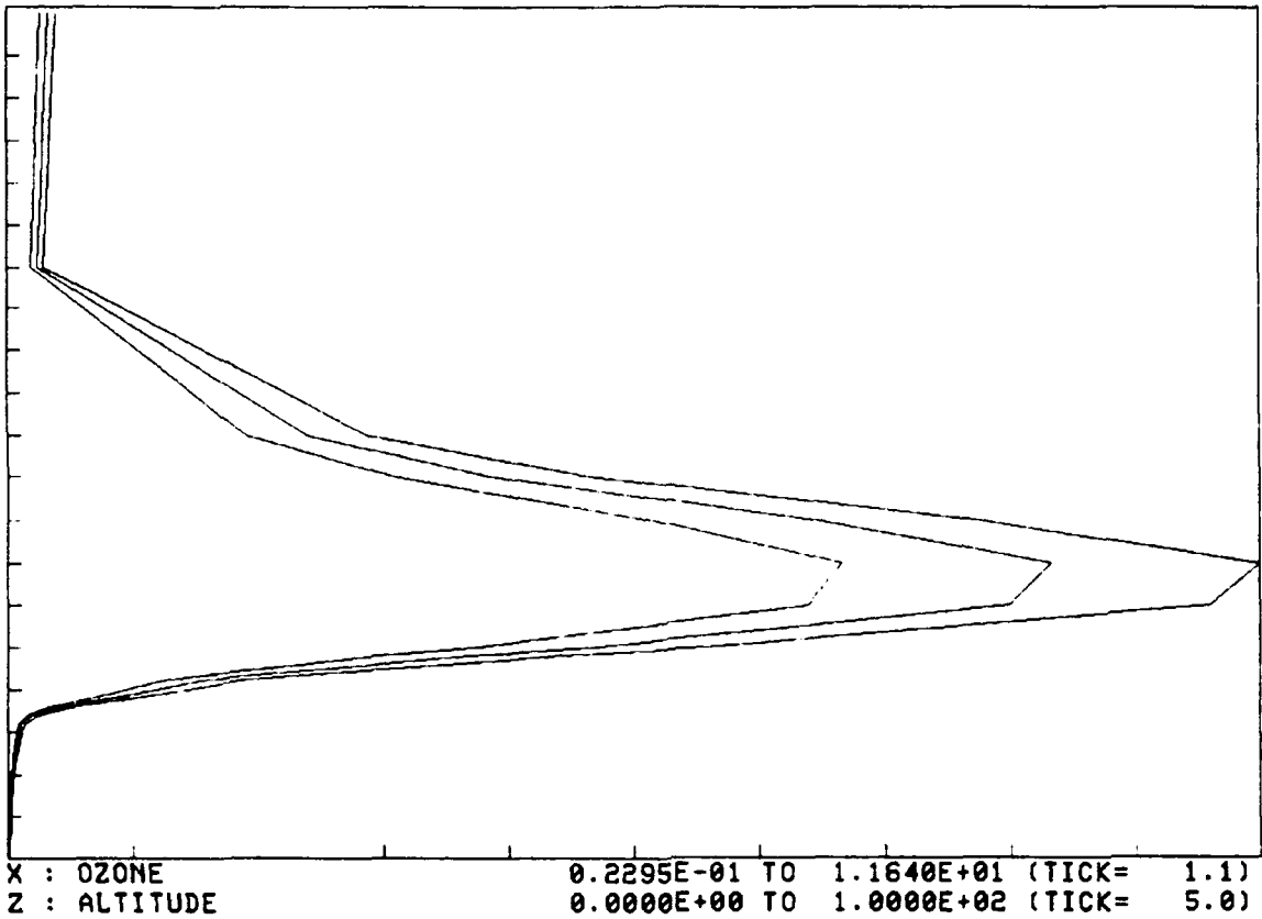
Figure 21. An Example of a 2-D Plot of an O 3 Input Profile with ± 20% Perturbations Assumed
