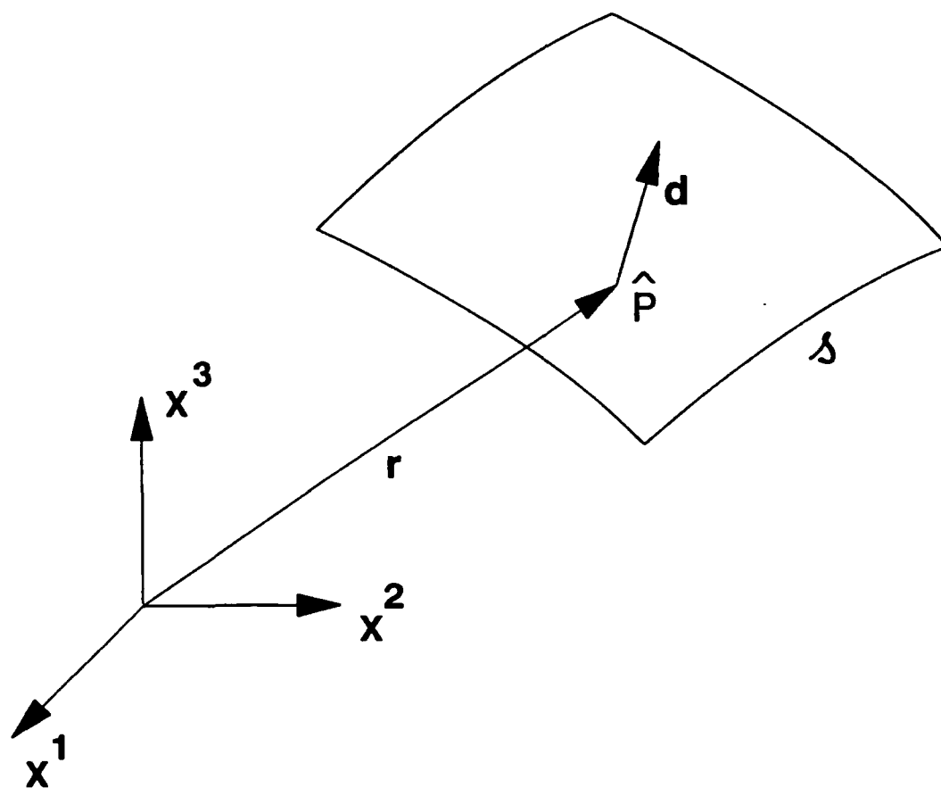
Figure 2 A typical Cosserat surface
