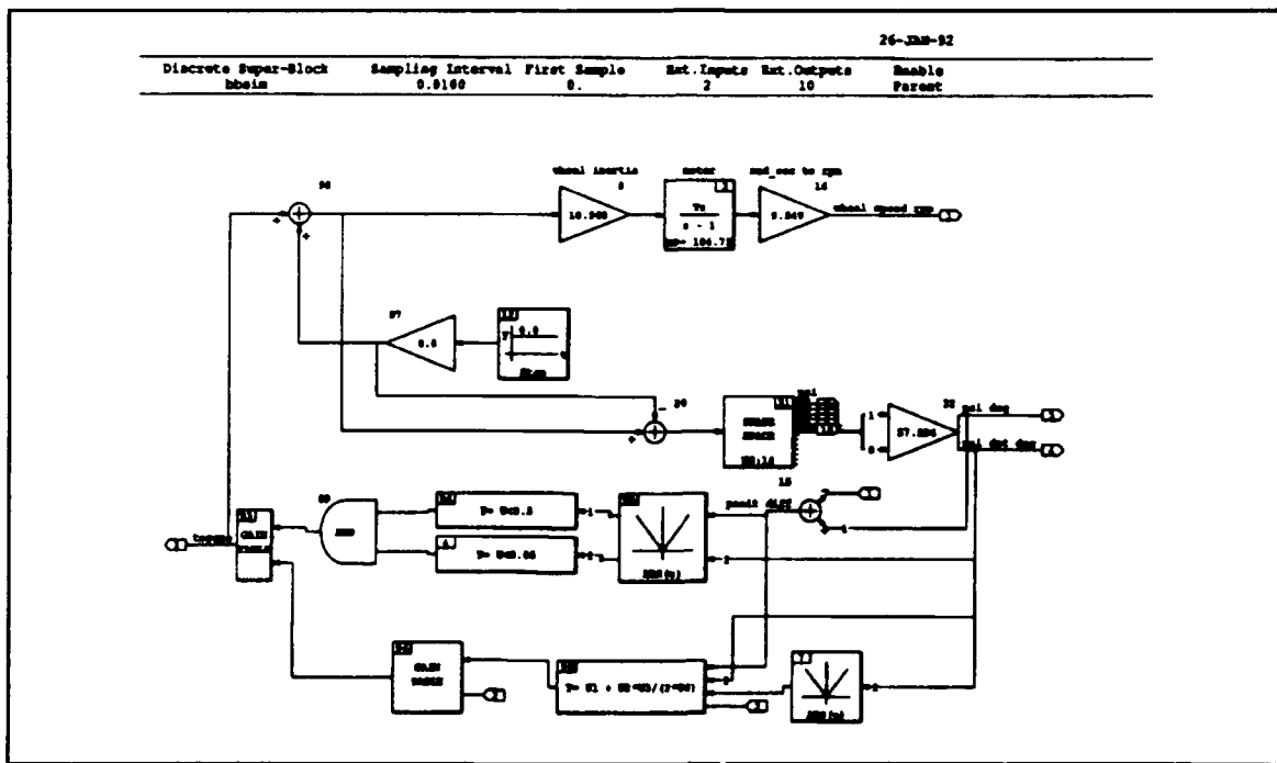
Figure 28. Bang-Bang Block Diagram
