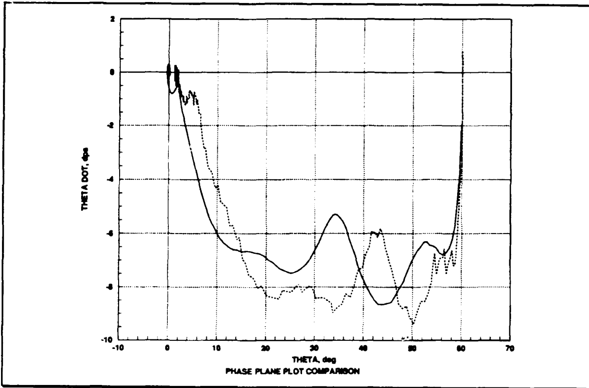
Figure 18. Phase Plot for a 60° Slew
