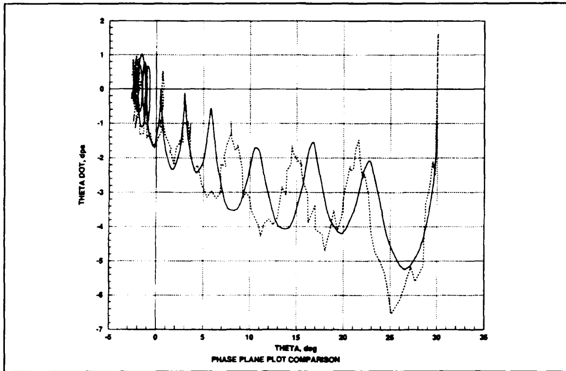
Figure 26. Phase Plot for a 30° Slew
