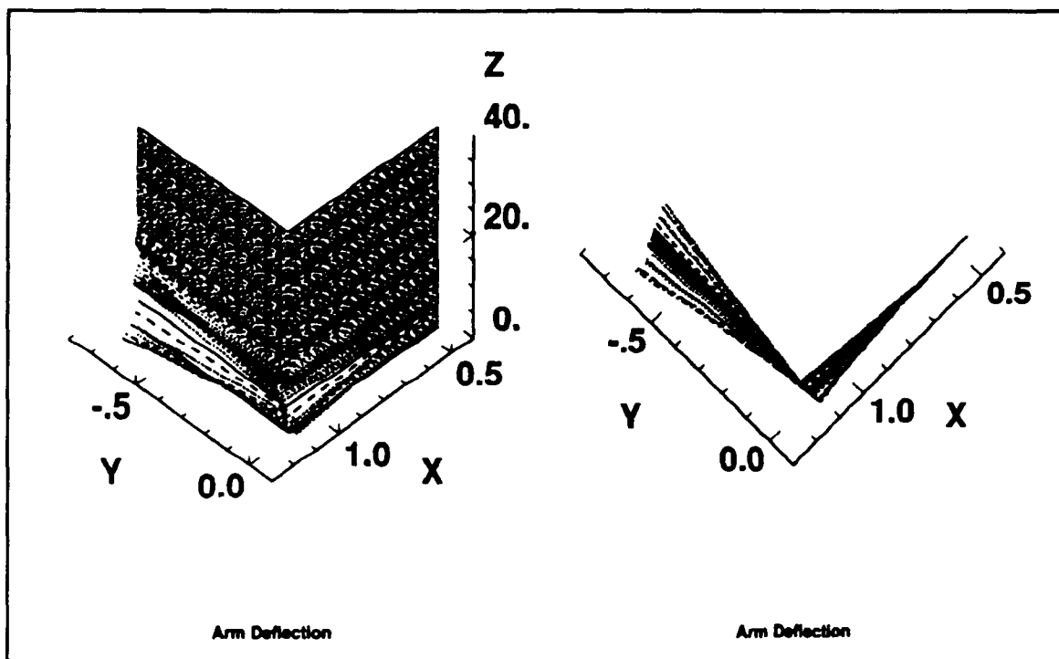
Figure 15. Arm Deflection for a 30° Slew
