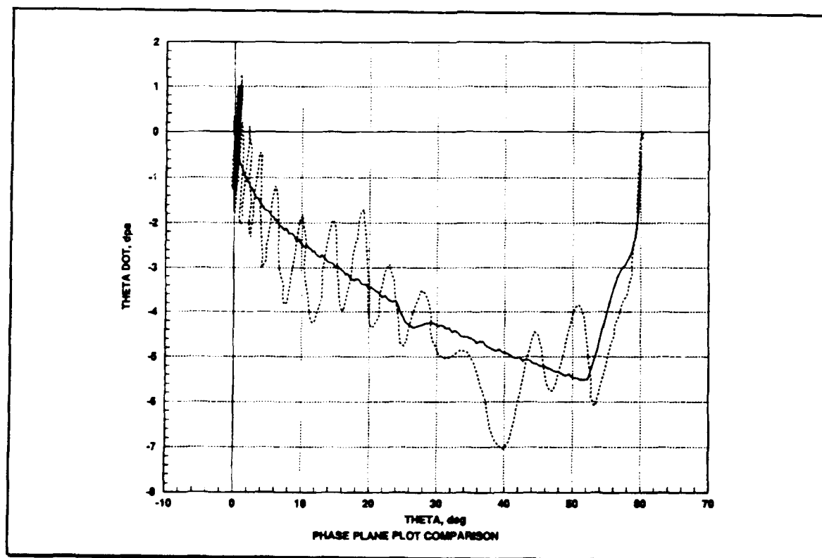
Figure 34. Phase Plot for a 60° Slew
