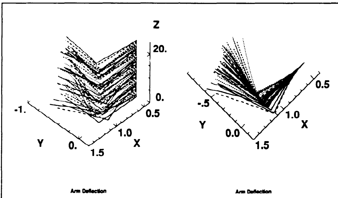
Figure 58. Arm Deflection for a 60° Slew
