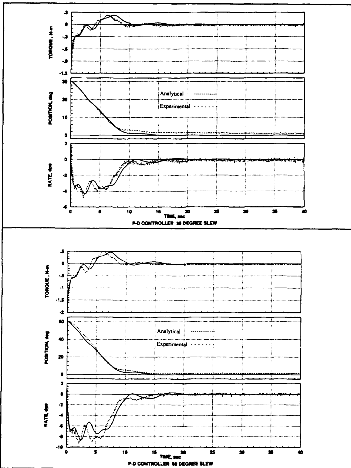
Figures 13 and 14. PD Controller Response
