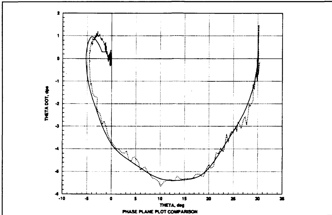
Figure 49. Phase Plot for a 30° Slew
