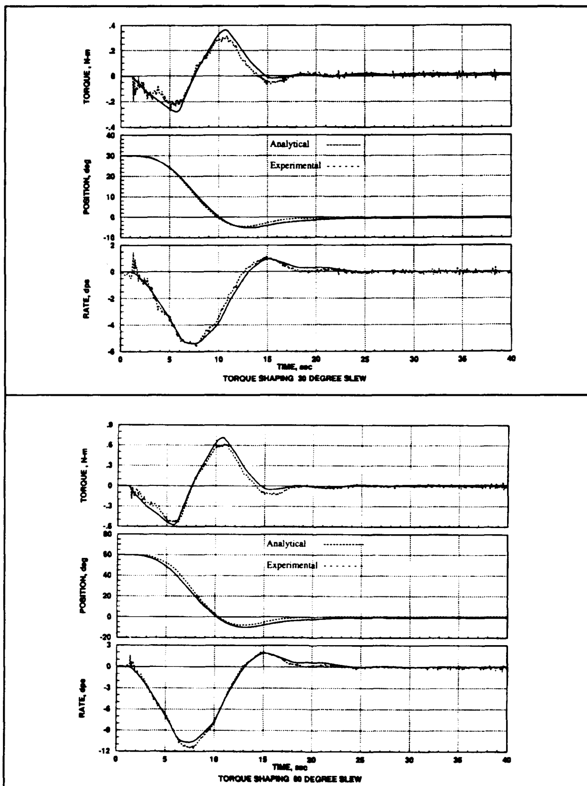
Figures 45 and 46. Pseudo-Square Controller Response
