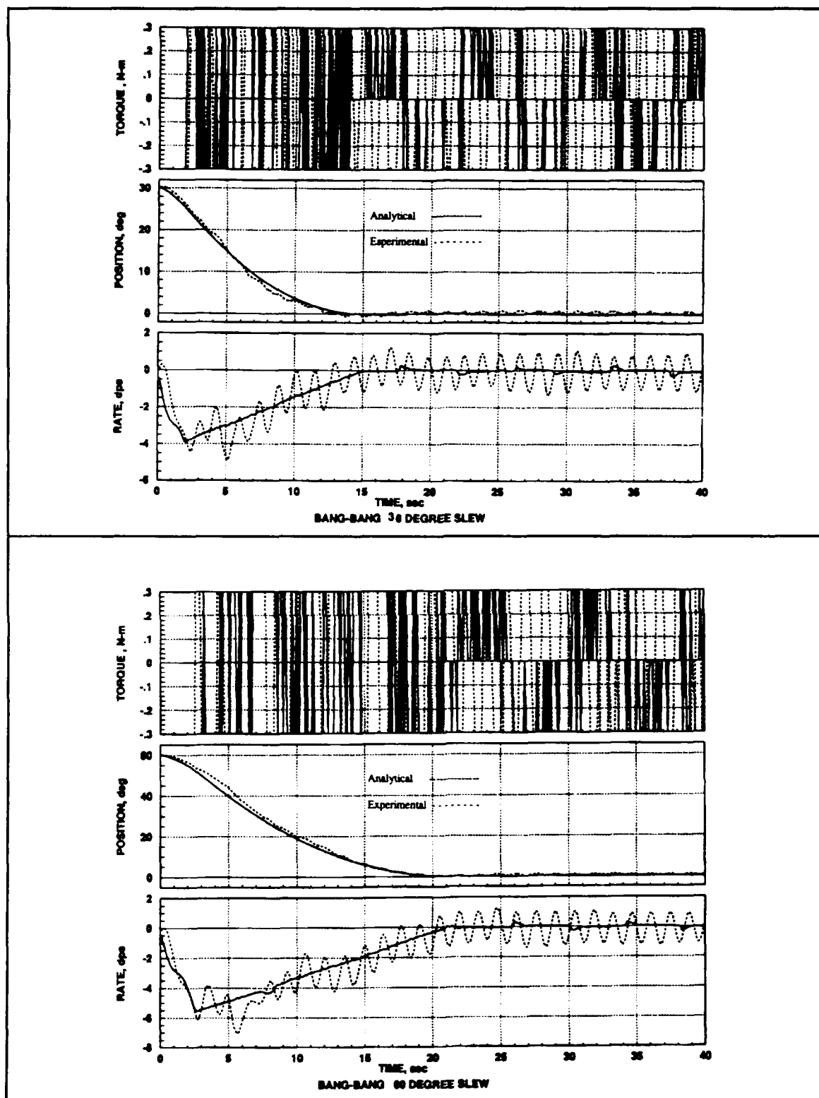
Figure 29 and 30. Bang-Bang Response
