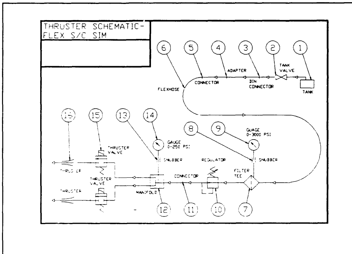
Figure 59. Thruster System Schematic
