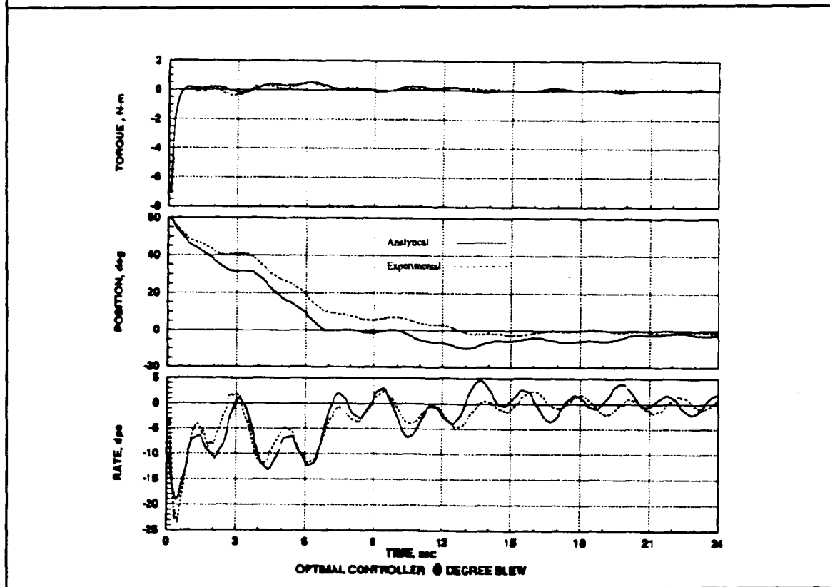
Figures 55 and 56. Optimal Response
