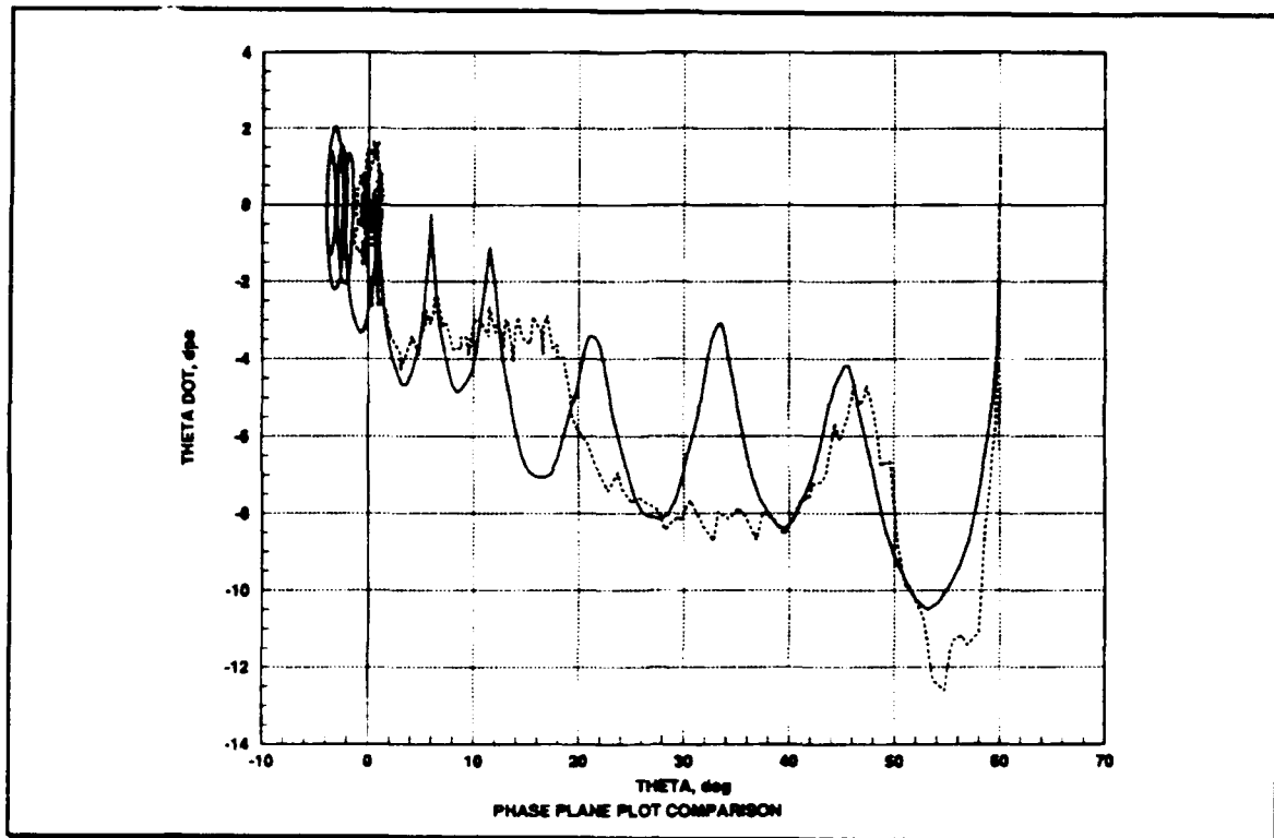
Figure 27. Phase Plot for a 60° Slew
