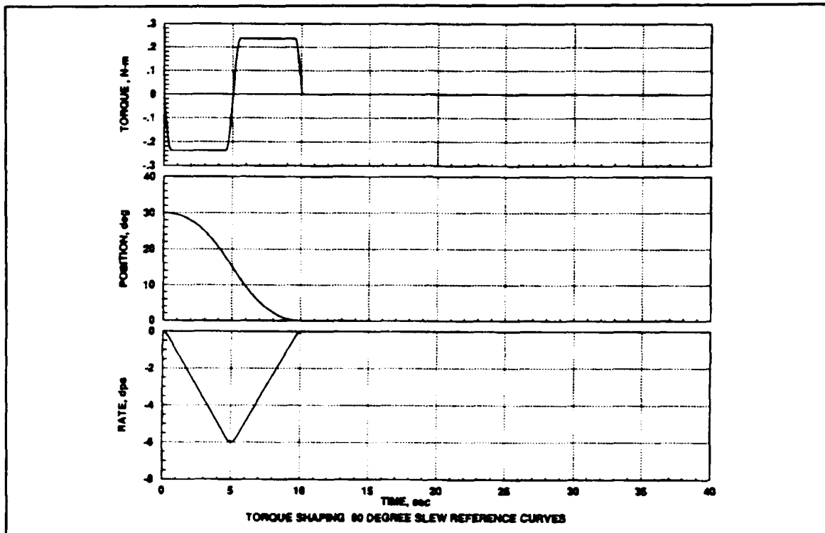
Figure 44. Reference Curves
