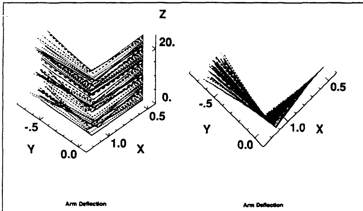
Figure 22. Arm Deflection for a 30° Slew
