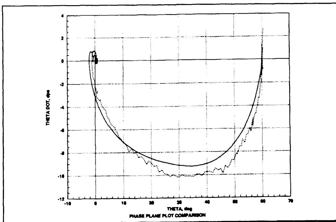
Figure 42. Phase Plot for a 60° Slew
