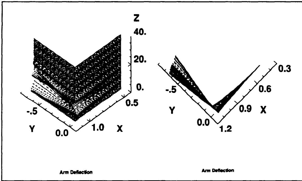
Figure 47. Arm Deflection for a 30° Slew
