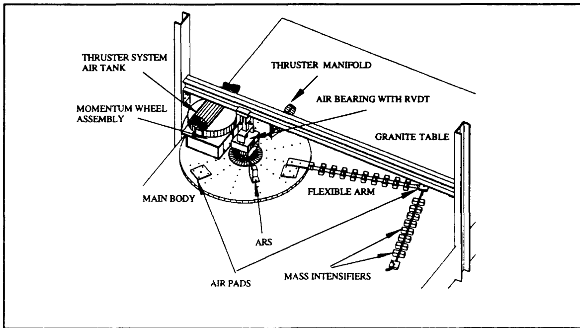
Figure 1. Flexible Spacecraft Simulator Configuration
