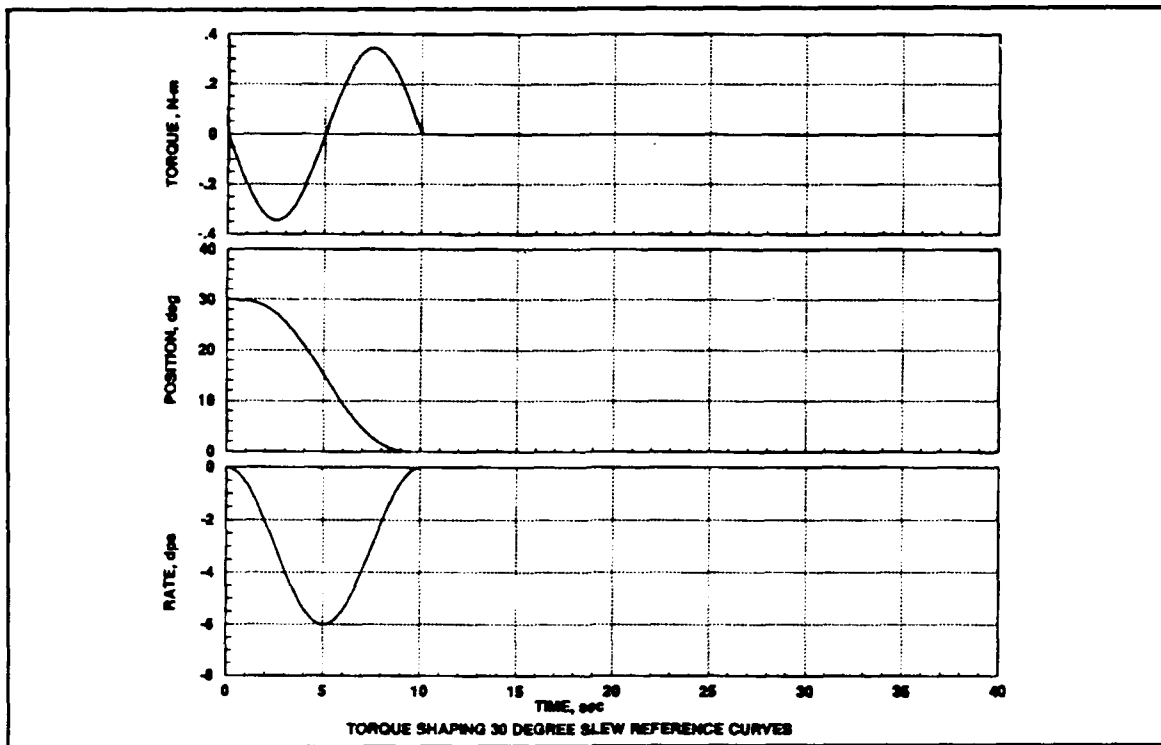
Figure 36. Reference Curves
