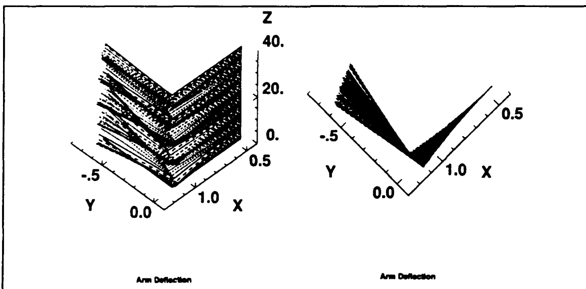
Figure 32. Arm Deflection for a 60° Slew
