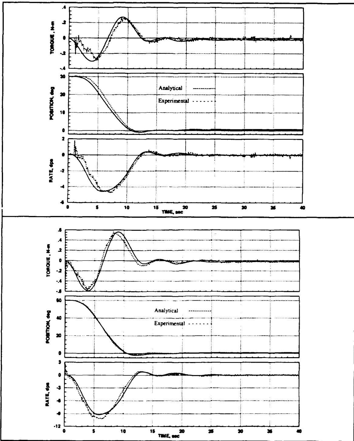
Figures 37 and 38. Sinusoidal Torque Shape Response
