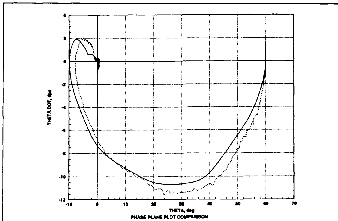
Figure 50. Phase Plot for a 60° Slew
