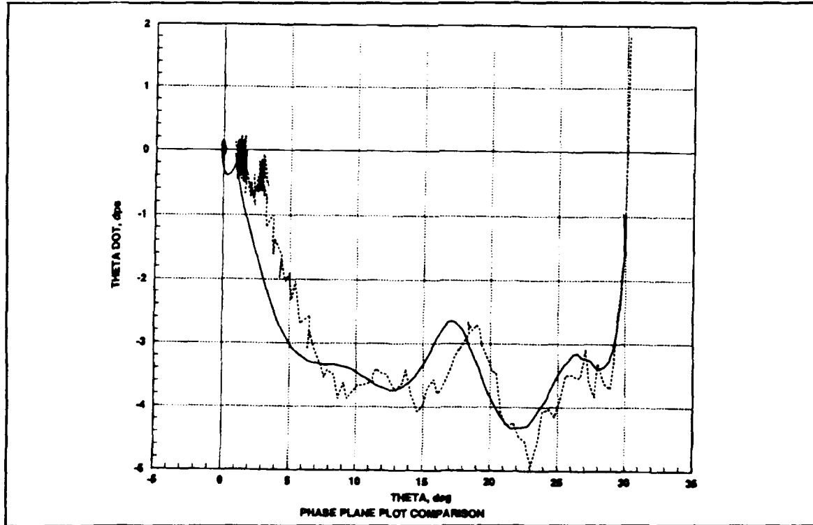
Figure 17. Phase Plot for a 30° Slew
