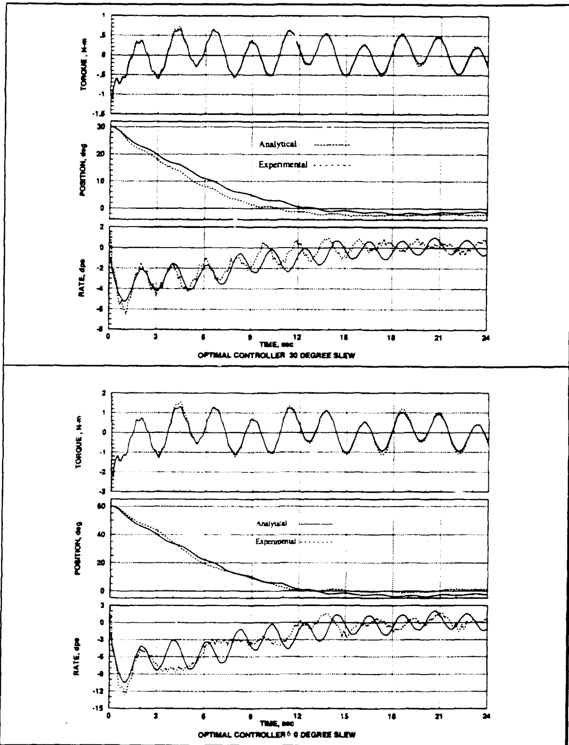
Figures 20 and 21. LQG Response
