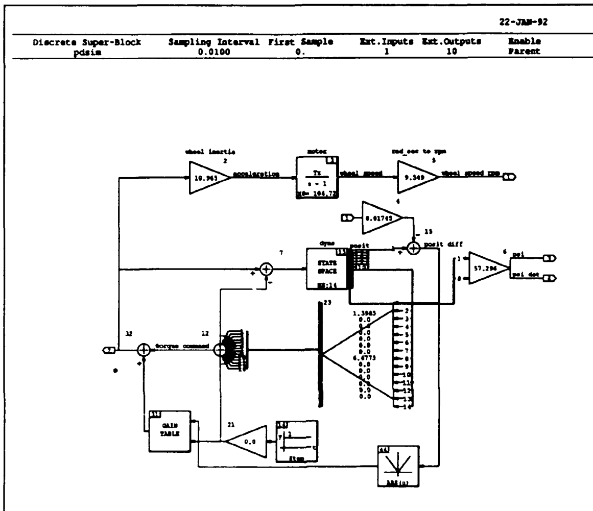
Figure 12. PD Controller Block Diagram
