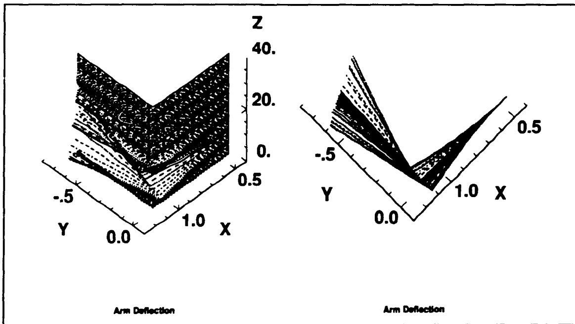
Figure 48. Arm Deflection for a 60° Slew
