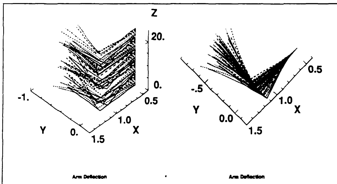
Figure 23. Arm Deflection for a 60° Slew
