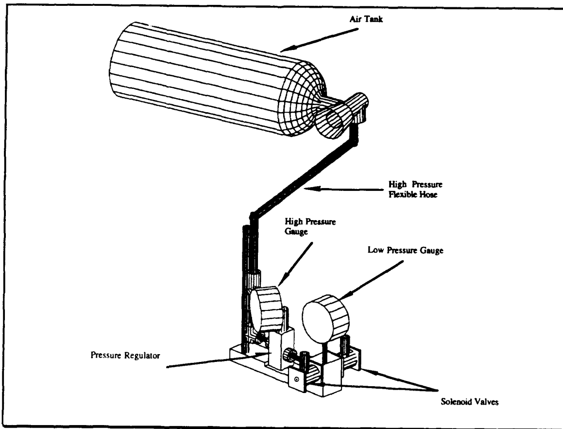
Figure 3. Thruster System Configuration
