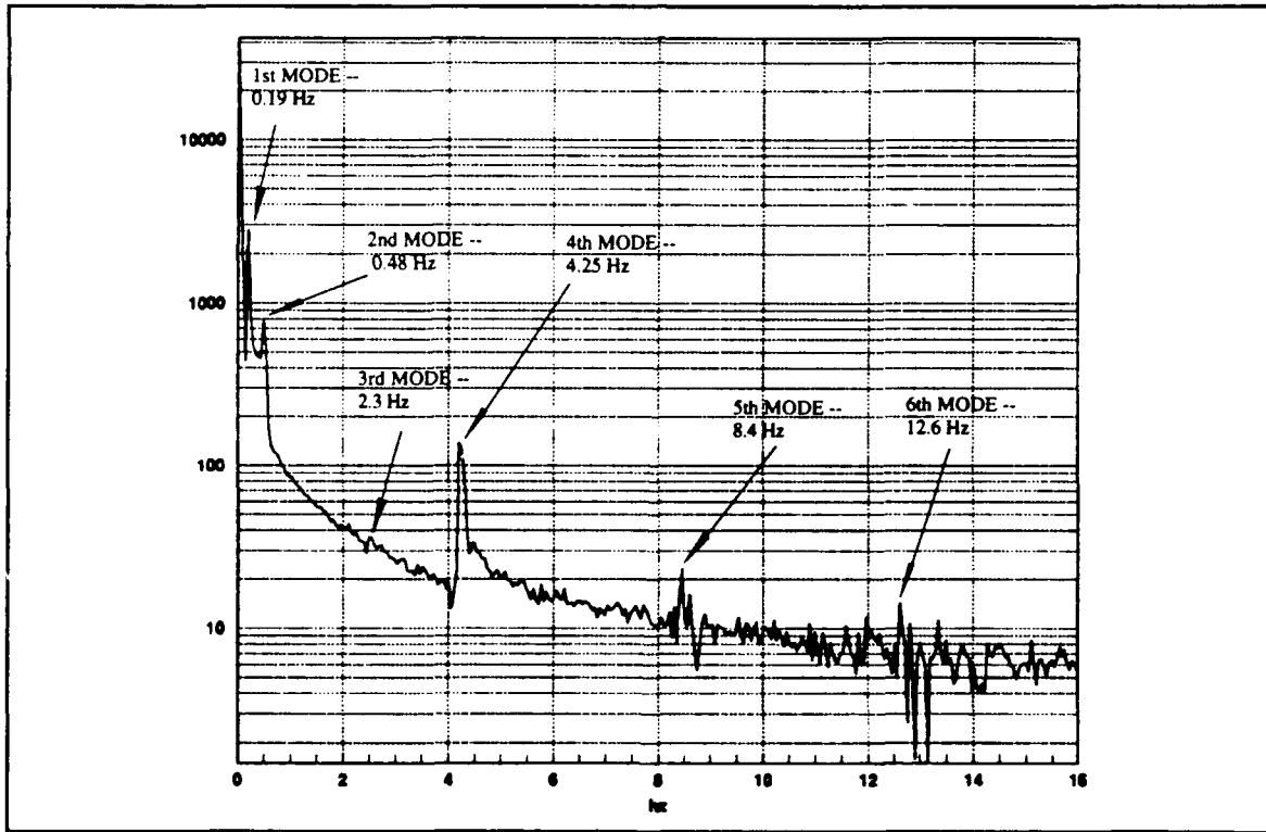
Figure C1. Modal Frequency Verification
