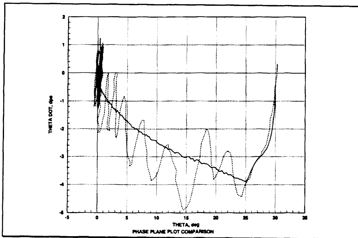
Figure 33. Phase Plot for a 30° Slew
