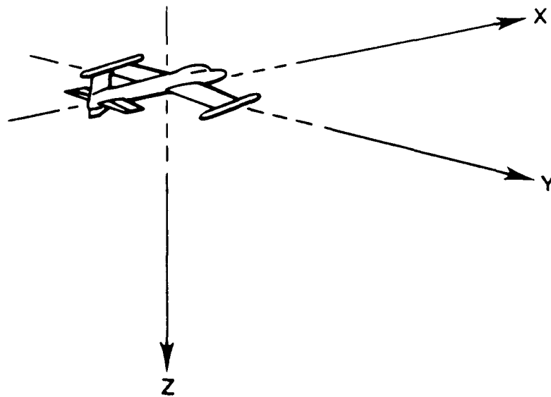
FIGURE 3 MANOEUVRE FRAME OF REFERENCE (conventional fixed/earth axis system)
