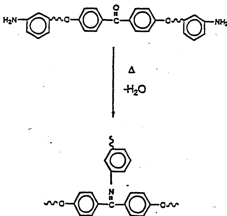
Figure 22. Proposed crosslinking mechanism for amine-terminated poly(arylene ether ketone)s [168].
