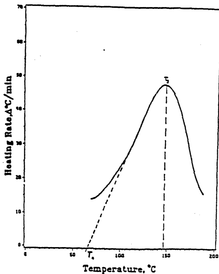
Figure 7. Heating rate ( dT/dt ) as a function of sample temperature provides the critical temperature, T_c , and the T_g at 2.45 GHz.
