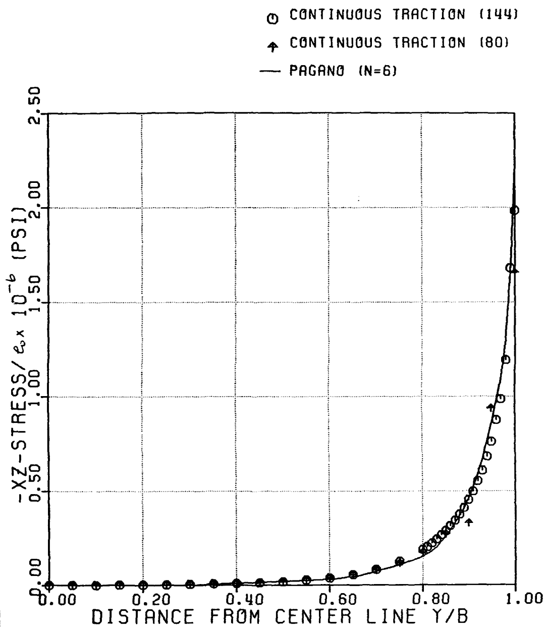
Figure 28: Distribution of XZ-stress Along \pm 45 Interface—Effect of Mesh Refinement
