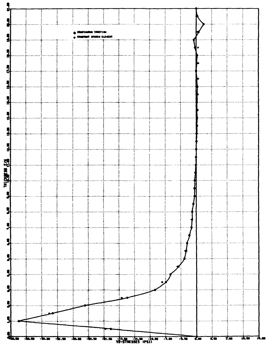
Figure 57: Through-Thickness Distribution of YZ-stress at the Center of the Second Element From the Free-Edge for Specimen D
