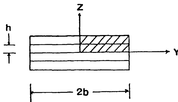
(a) Symmetric Laminate
