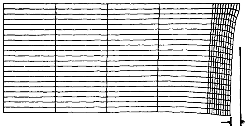
(b) Deformed Model of D Laminate
