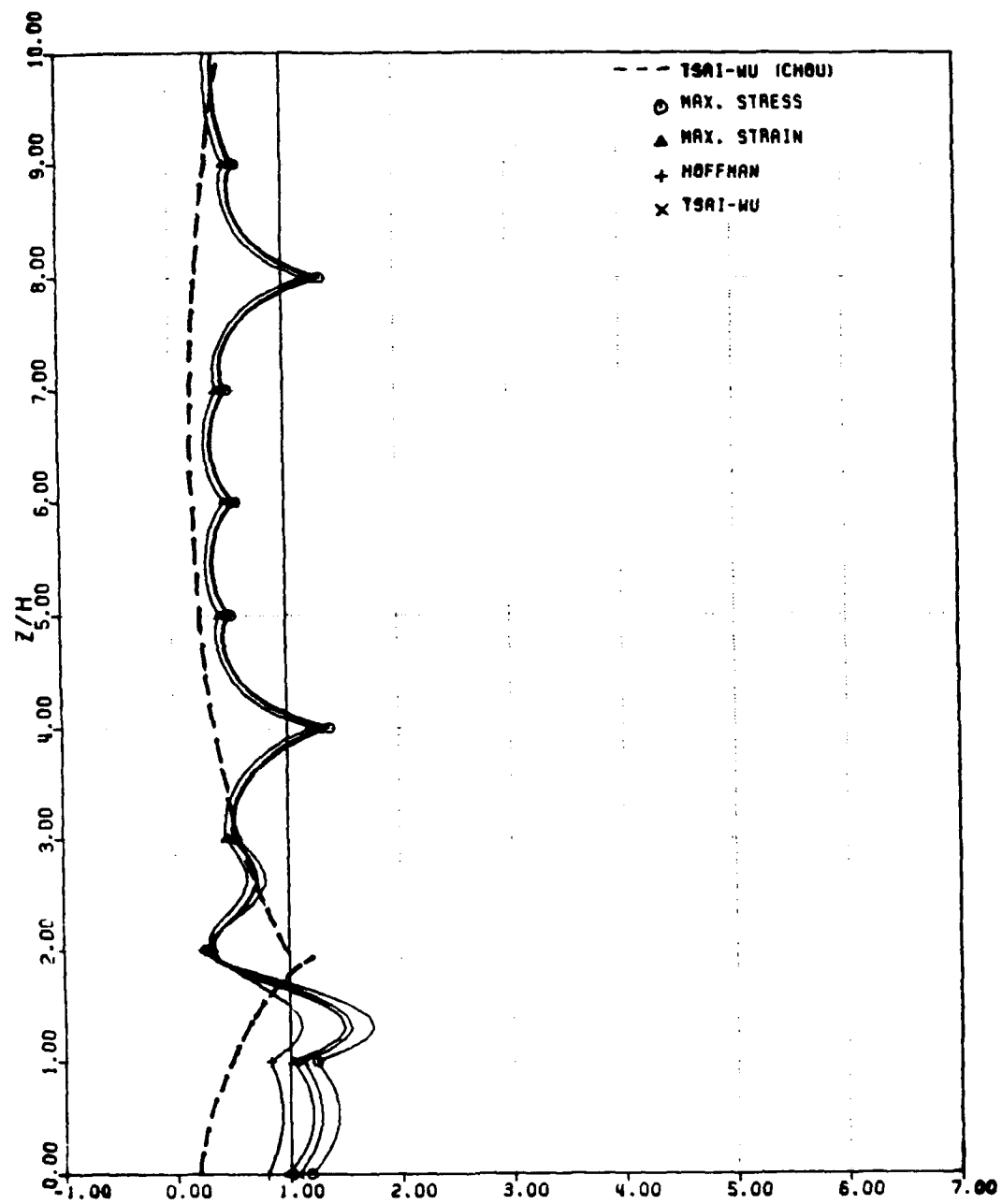
Figure 62: Ratio of Stress-to-Strength Tensor for [(\pm 15)_2/90]_5 Laminate under Transverse Cracks Loading
