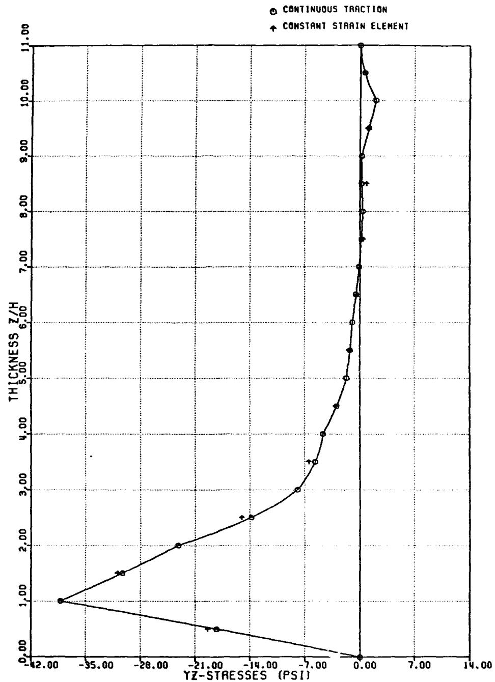
Figure 54: Through-Thickness Distribution of YZ-stress at the Center of the Second Element From the Free-Edge for Specimen A
