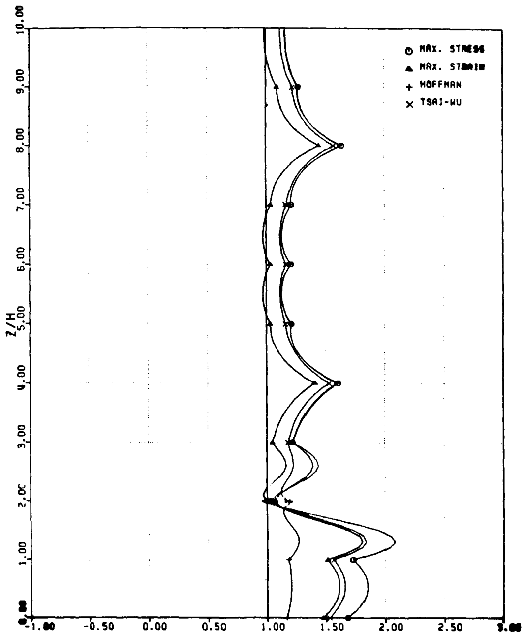
Figure 66: Ratio of Stress-to-Strength Tensor for [(\pm 5)_2/90]_S Laminate under Delamination Loading
