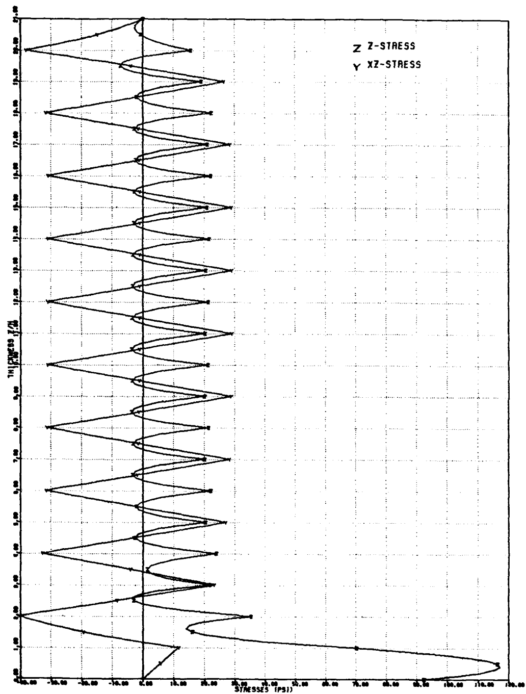
Figure 41: Through-Thickness Stress Distributions at the Free-Edge of Specimen D Based on the Continuous Traction Q-23 Element
