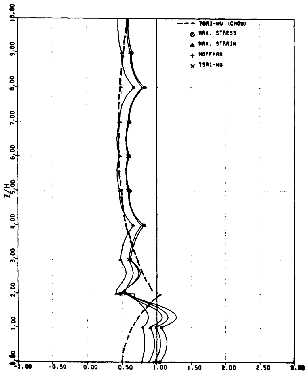
Figure 61: Ratio of Stress-to-Strength Tensor for [(\pm 5)_2/90]_S Laminate under Transverse Cracks Loading
