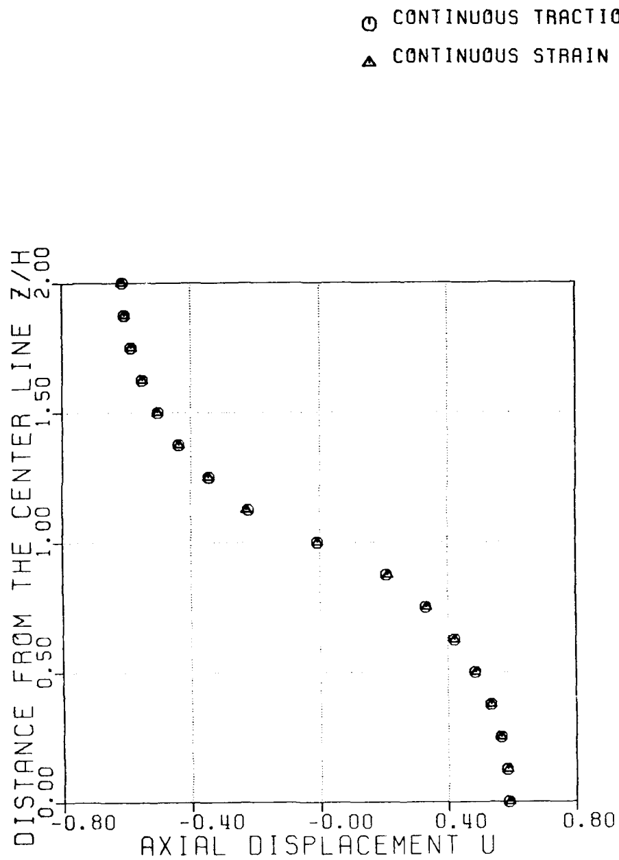
Figure 16: Through-Thickness Distribution of Axial Displacement at the Free-Edge of [45/-45]_s Laminate
