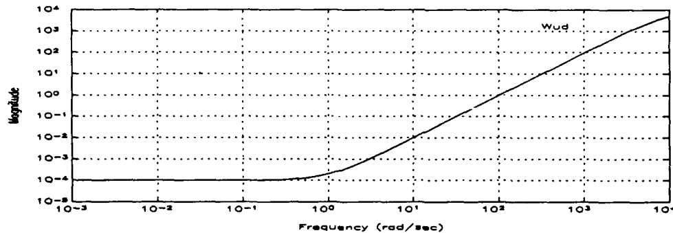
FIGURE 14. EXAMPLE OF UNMODELED DYNAMICS WEIGHT
