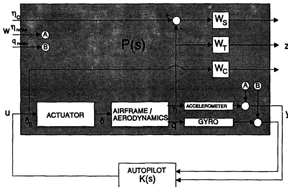
FIGURE 11. H_\infty FRAMEWORK FOR MISSILE AUTOPILOT EXAMPLE
