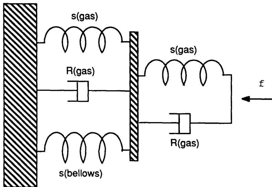
Figure 2.4 The Mass Element Resonator Mechanical Analogy
