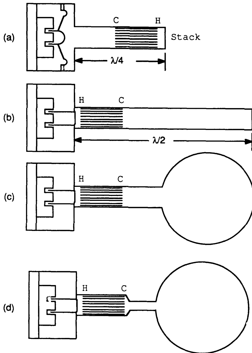
Figure 1.2 Resonator Evolution
