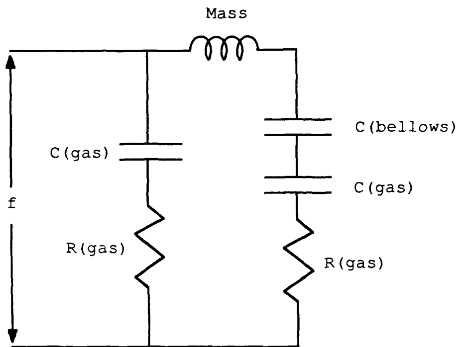
Figure 2.5 The Electrical Equivalent Circuit
